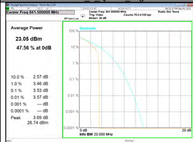
Band 26_1_Q16_High
