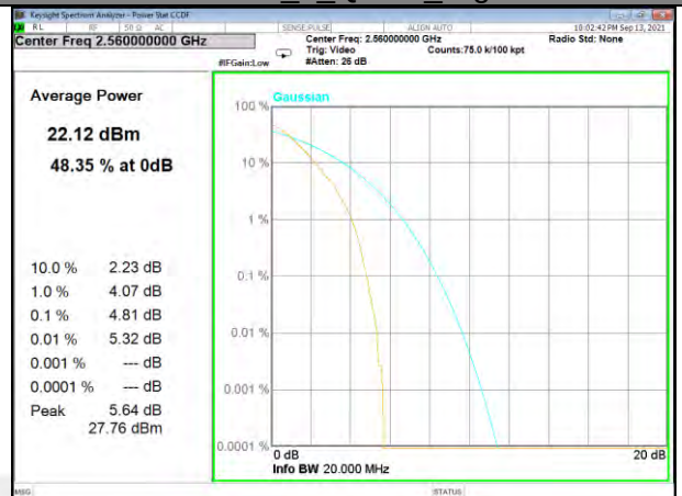
Band 7_1_Q16_High
