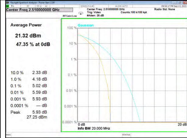
Band 7_100_Q16_Low
