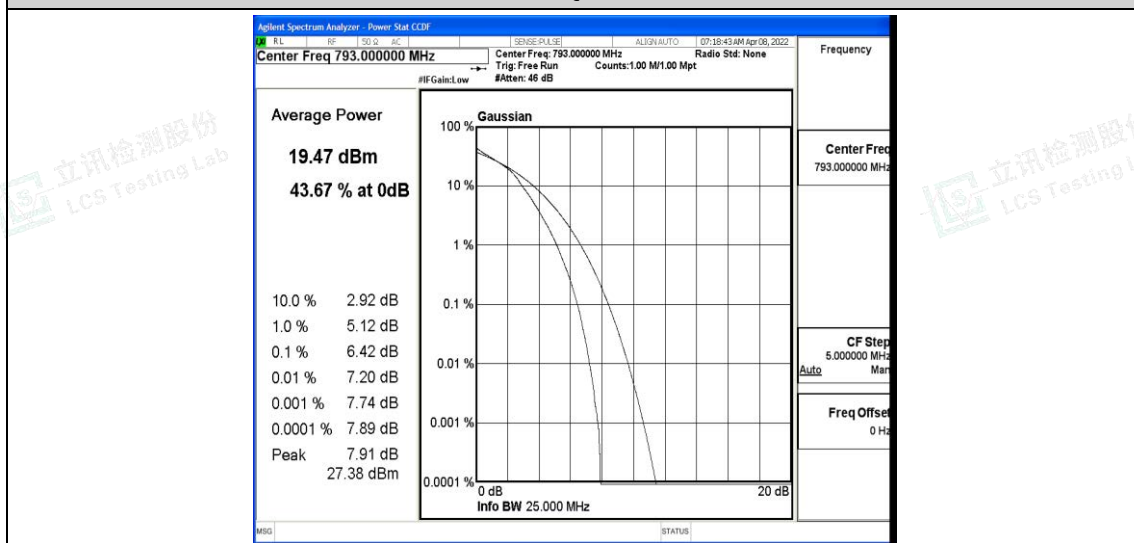
Band14-10MHz-16QAM-23330-50RB#0
