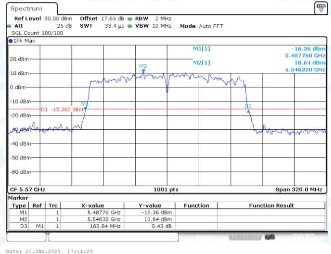
11AC160-CDD-Ant2-5570
