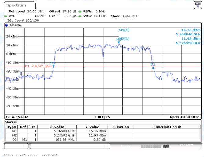
11AC160-CDD-Ant2-5250
