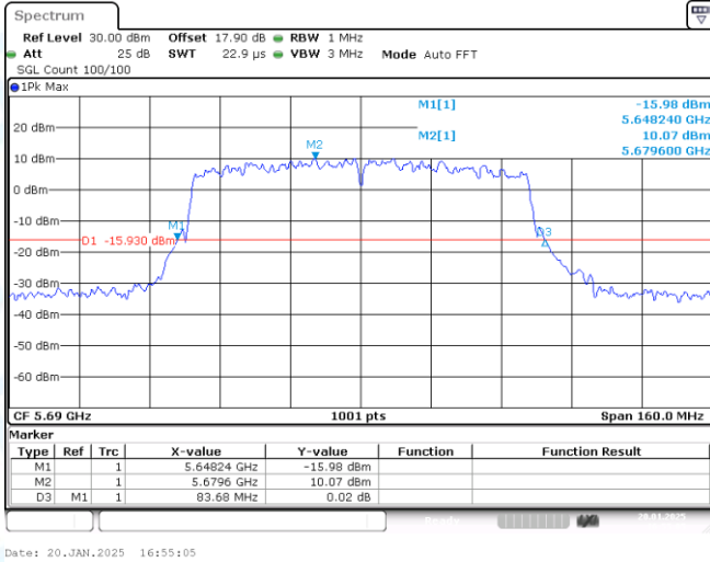
11AC80-CDD-Ant1-5690
