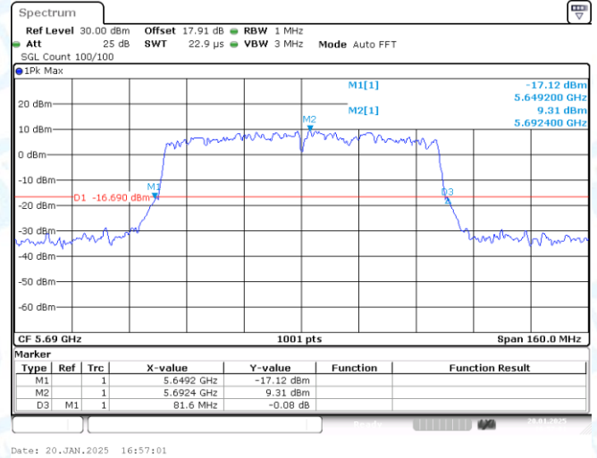
11AC80-CDD-Ant2-5690
