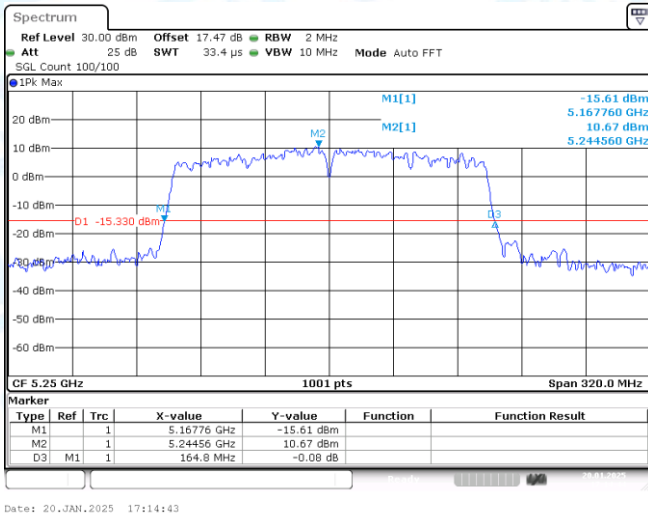
11AC160-CDD-Ant1-5250
