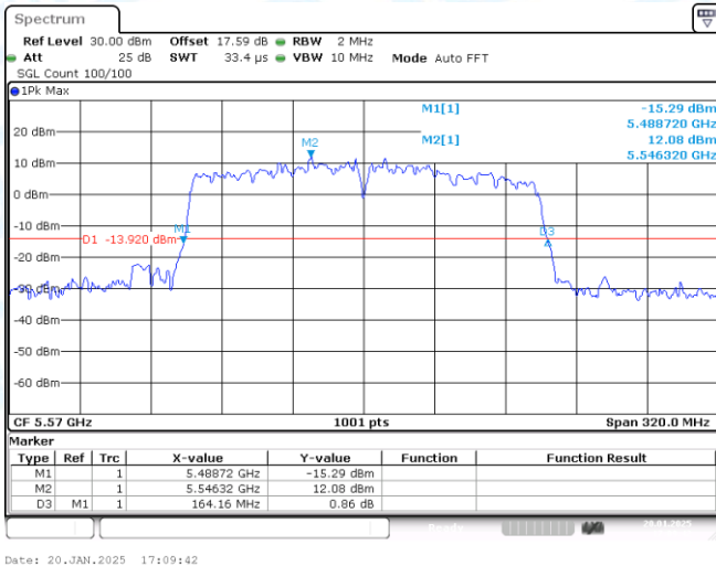
11AC160-CDD-Ant1-5570
