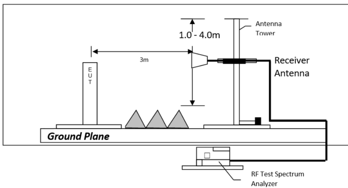
Test setup of radiated emissions above 1GHz
