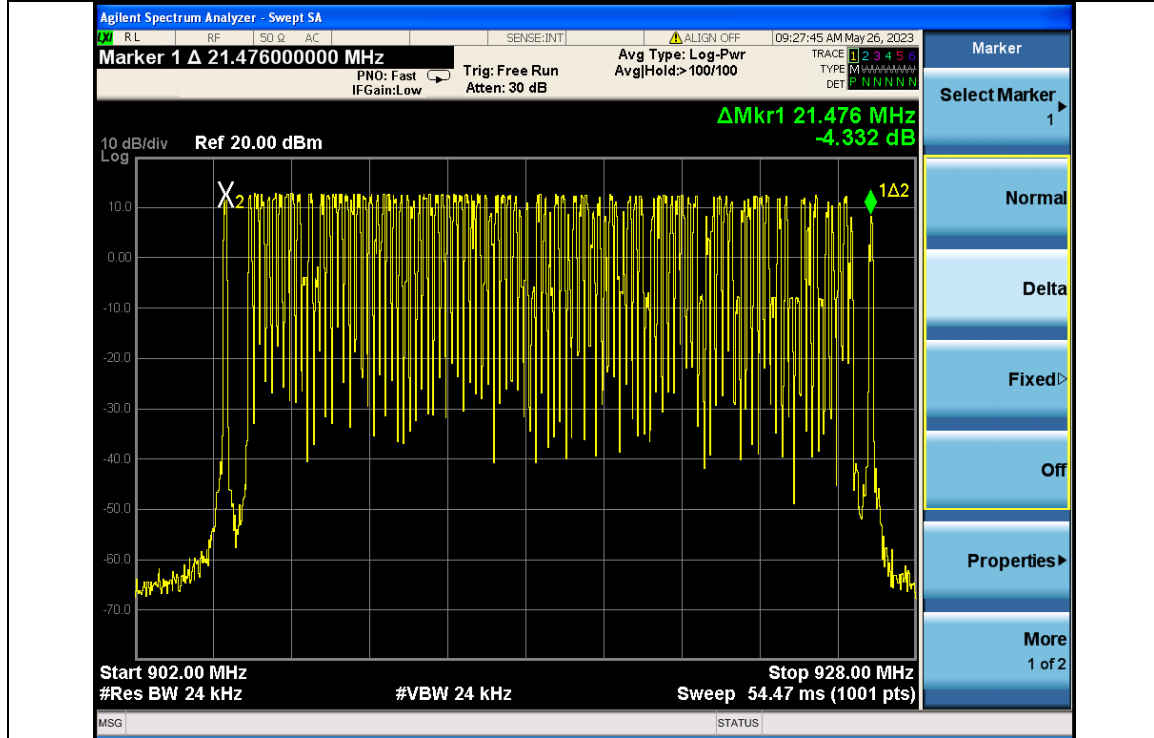
Number of Hopping Channel Plot
