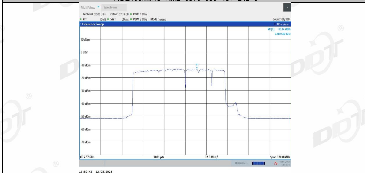
11BE160MIMO Ant3 5570 996+484 1
