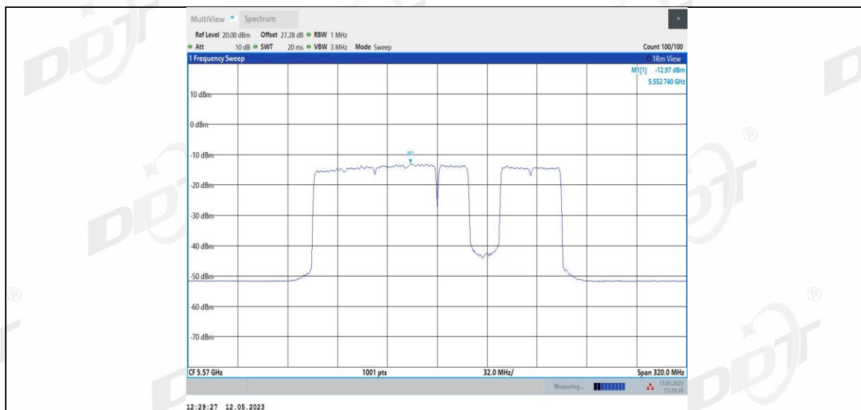
11BE160MIMO Ant2 5570 996+484+242 7
