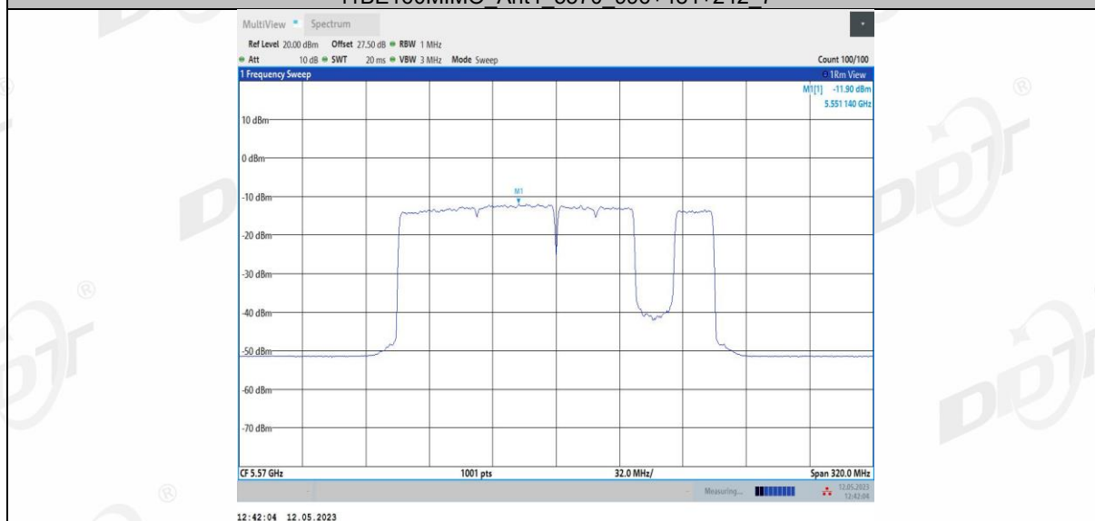
11BE160MIMO Ant4 5570 996+484+242_8
