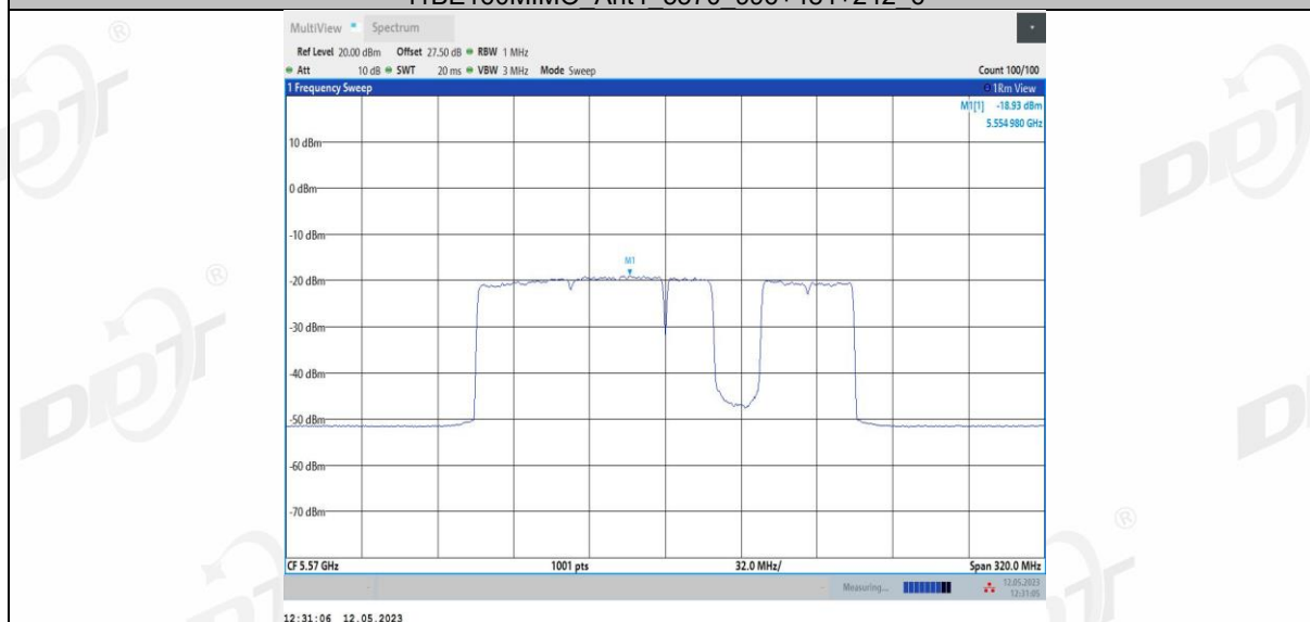
11BE160MIMO Ant4 5570 996+484+242_7
