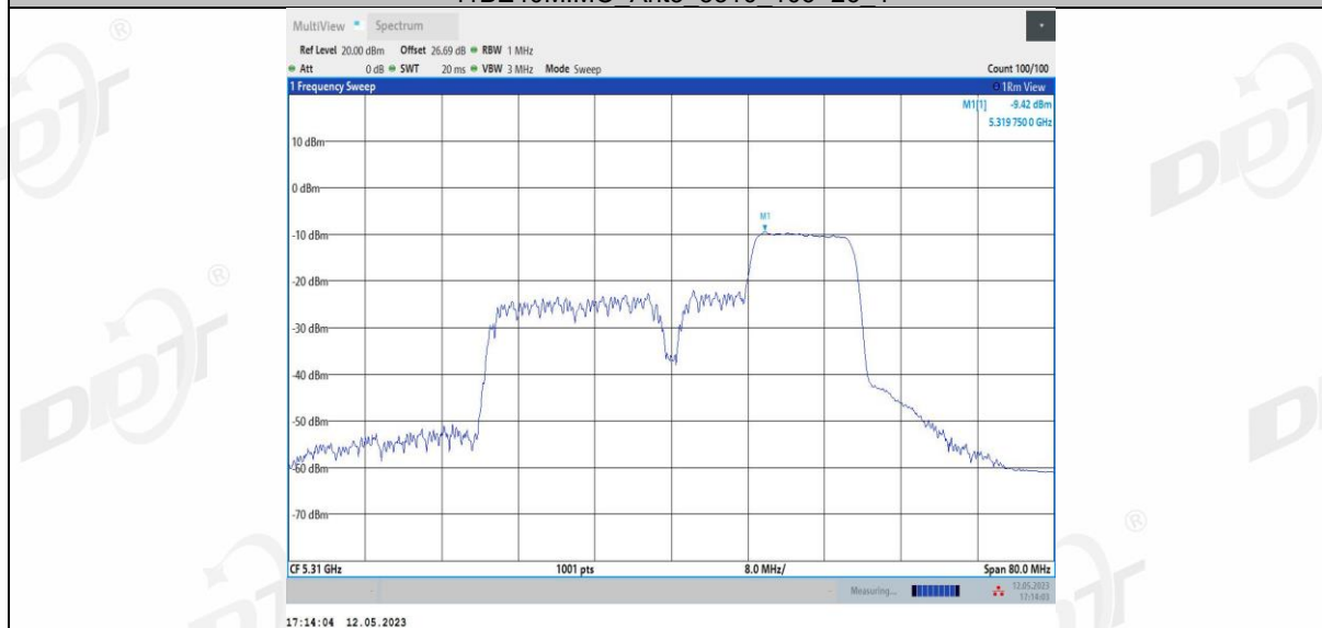
11BE40MIMO Ant4 5310 106+26 3
