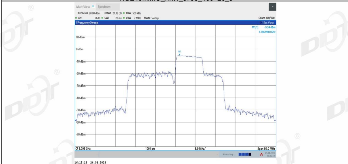
11BE40MIMO Ant4 5795 106+26 4
