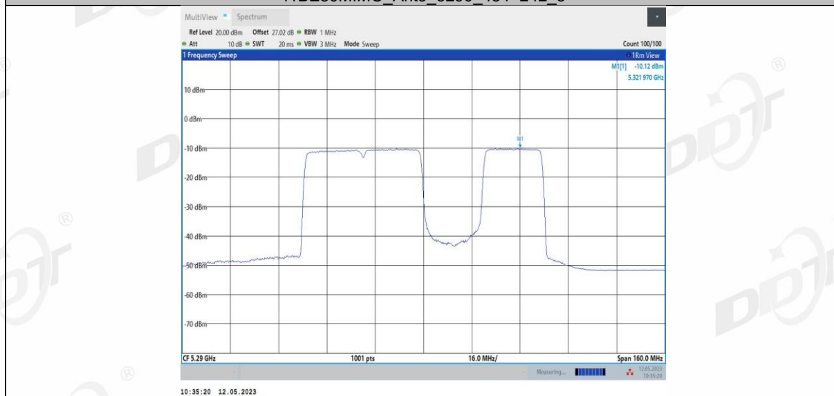
11BE80MIMO Ant3 5290 484+242 4
