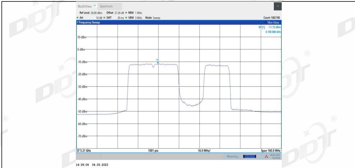
11BE80MIMO Ant2 5210 484+242 4
