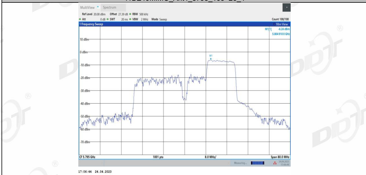
11BE40MIMO Ant4 5795 106+26 4
