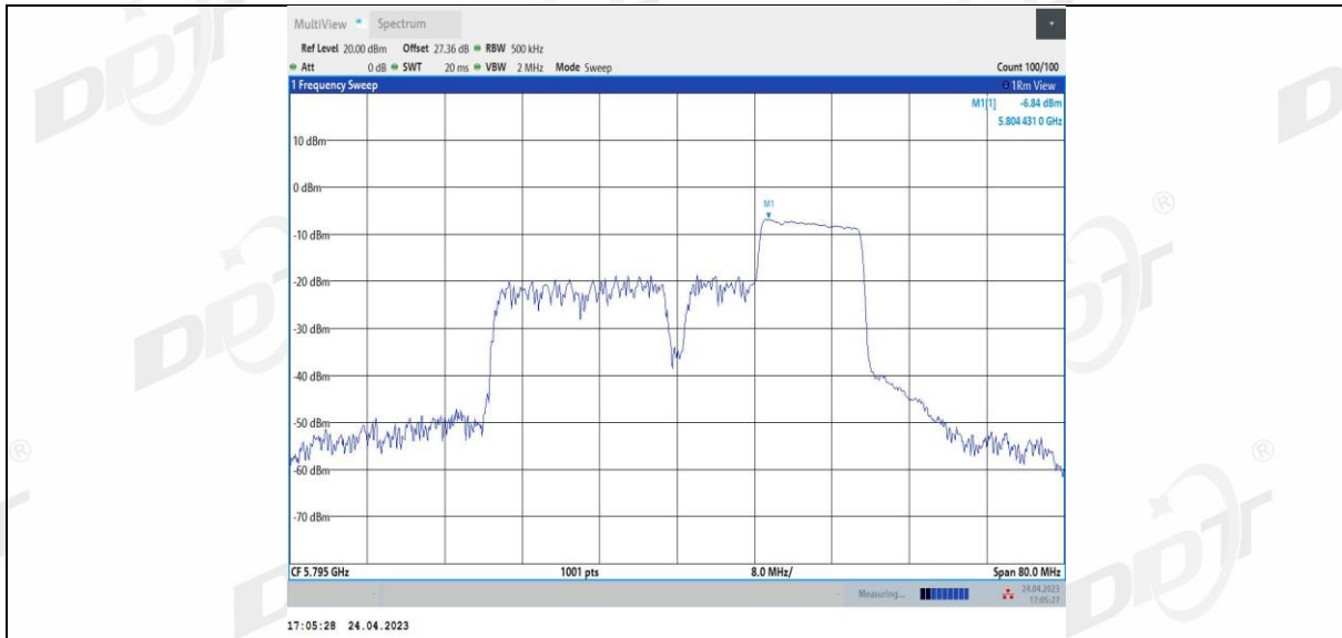
11BE40MIMO Ant4 5795 106+26 3
