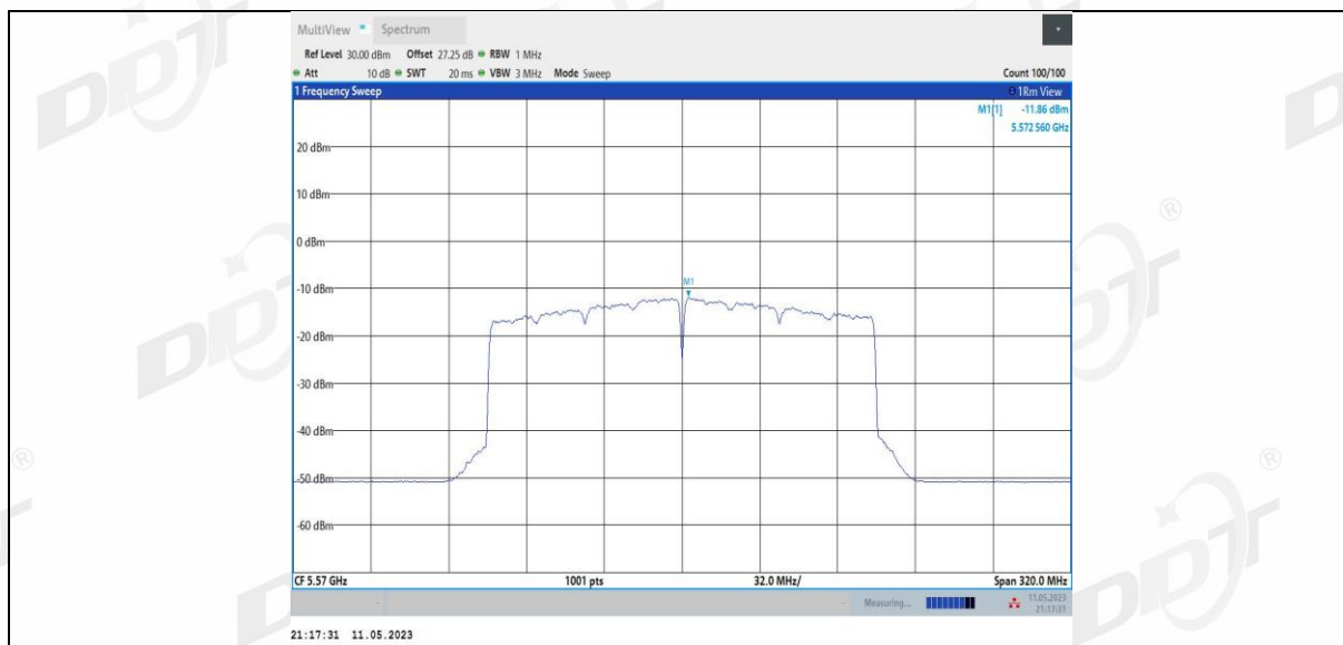
11AX160MIMO Ant3 5570
