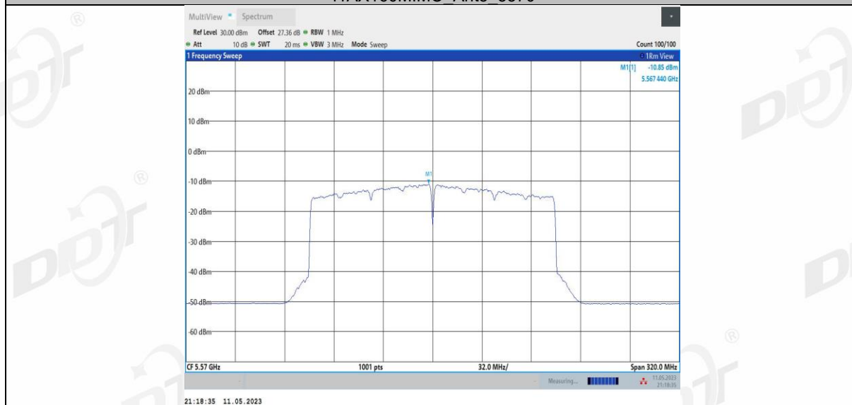
11AX160MIMO Ant4 5570
