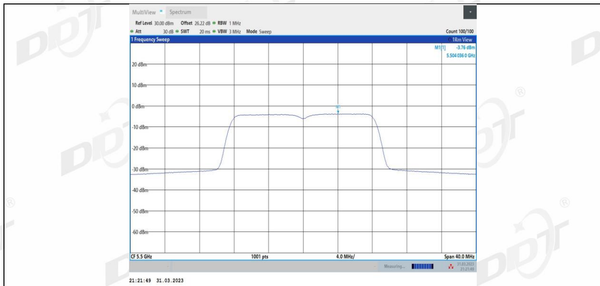
11A-CDD Ant4 5500
