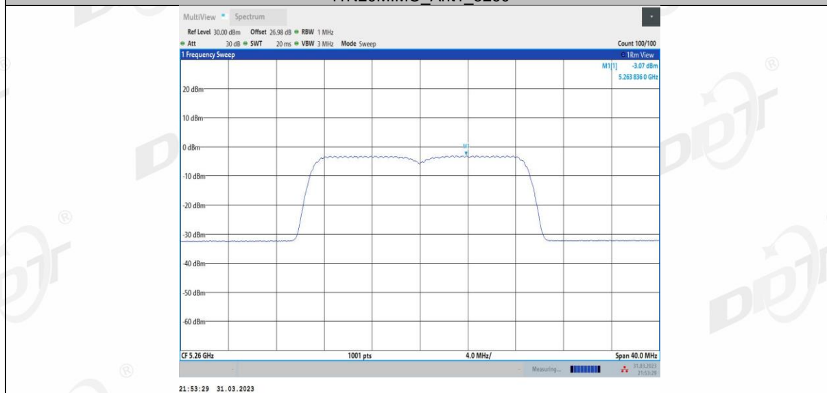
11N20MIMO Ant2 5260
