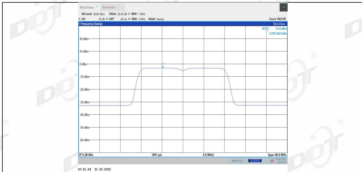
11A-CDD Ant3 5280
