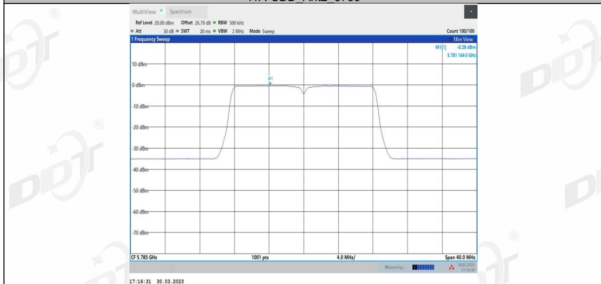
11A-CDD Ant3 5785
