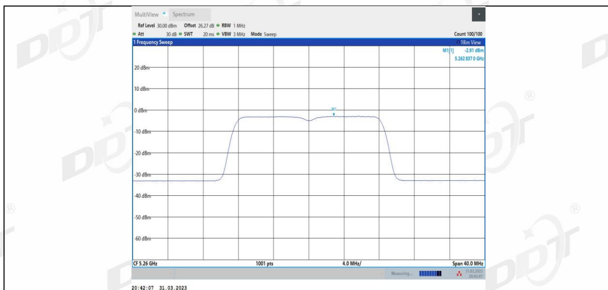
11A-CDD Ant4 5260
