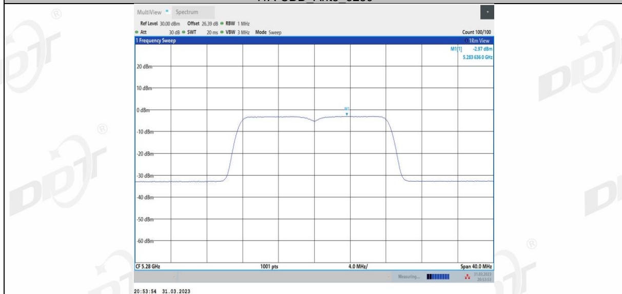
11A-CDD Ant4 5280
