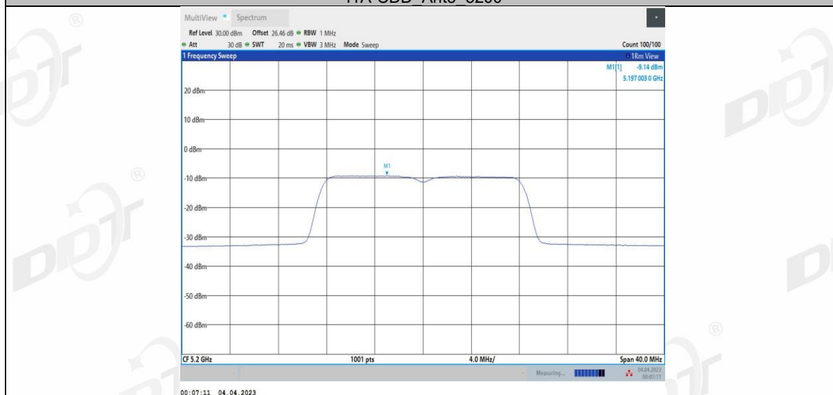
11A-CDD Ant4 5200
