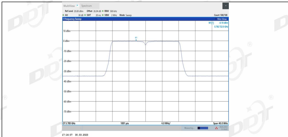
11A-CDD Ant2 5785
