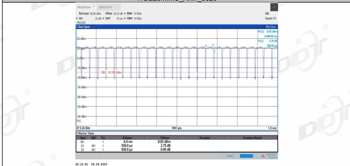
11BE20MIMO Ant2 5320
