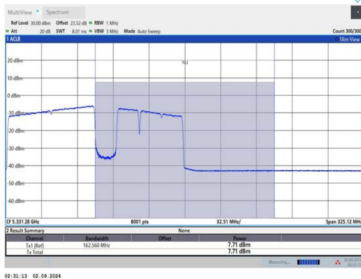
11BE160MIMO Ant1 5250 UNII-2A 996+484+242 OFDMA 6
