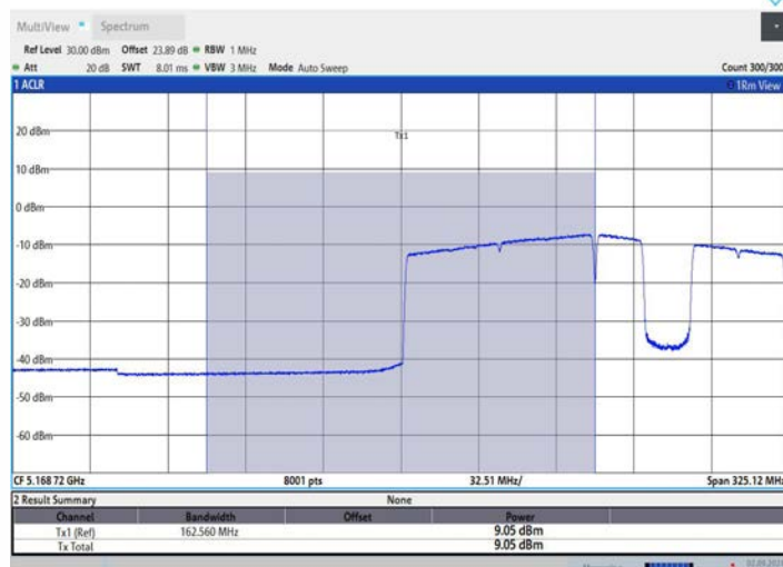
11BE160MIMO_Ant2_5250_UNII-1_996+484+242_OFDMA_7
