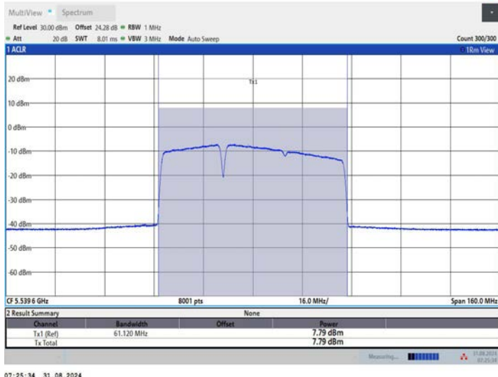
11BE80MIMO_Ant1_5530_484+242_OFDMA_1
