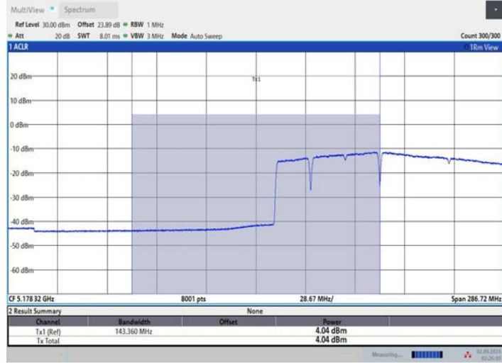
11BE160MIMO_Ant2_5250_UNII-1_996+484+242_OFDMA_1
