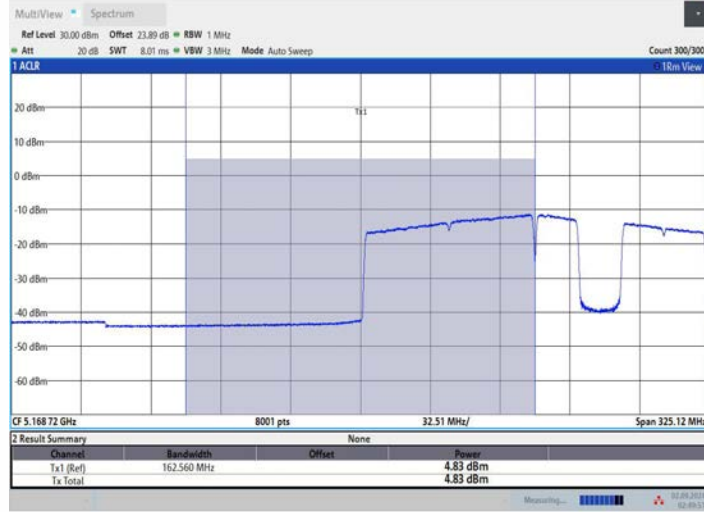
11BE160MIMO_Ant2_5250_UNII-1_996+484+242_OFDMA_6
