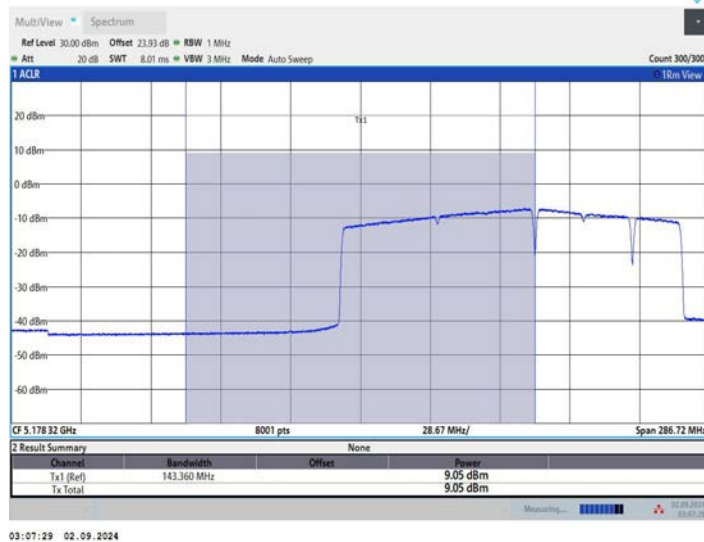
11BE160MIMO_Ant3_5250_UNII-1_996+484+242_OFDMA_1
