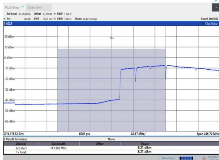
11BE160MIMO_Ant2_5250_UNII-1_996+484+242_OFDMA_2
