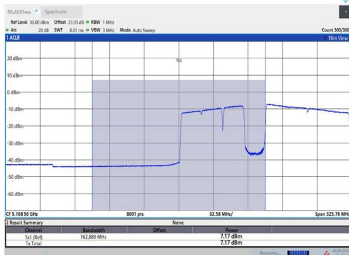
11BE160MIMO_Ant2_5250_UNII-1_996+484+242_OFDMA_5
