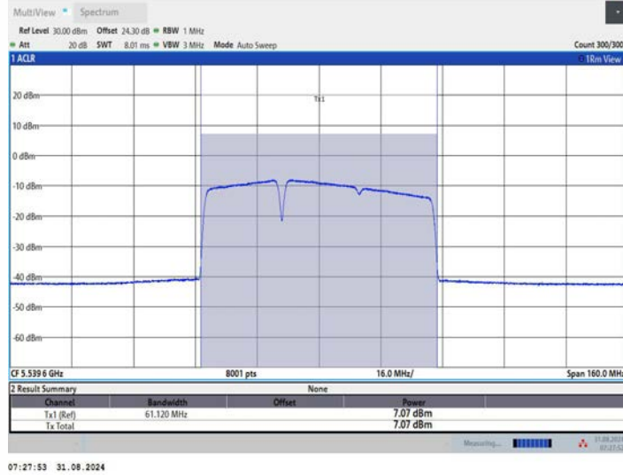
11BE80MIMO_Ant3_5530_484+242_OFDMA_1
