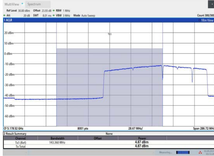
11BE160MIMO_Ant2_5250_UNII-1_996+484+242_OFDMA_8
