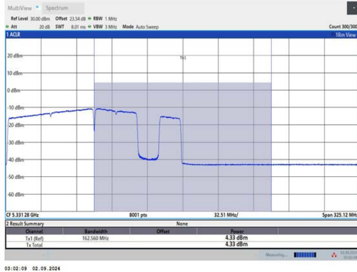
11BE160MIMO Ant3 5250 UNII-2A 996+484+242 OFDMA 7
