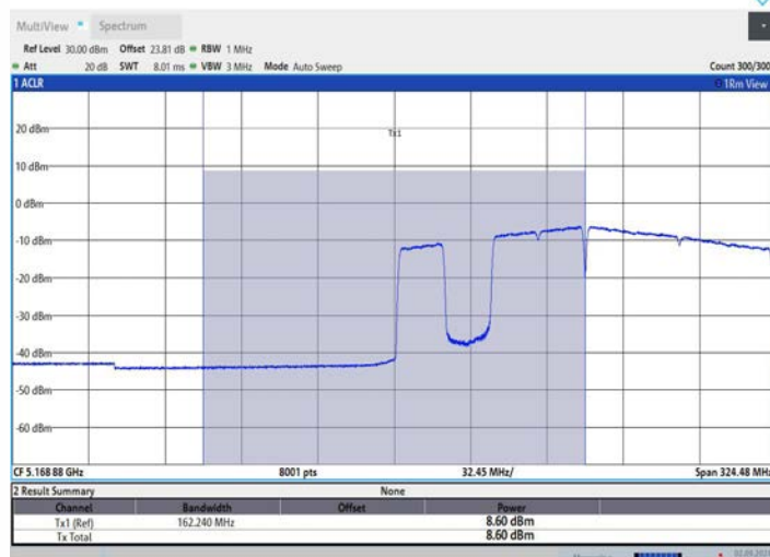
11BE160MIMO_Ant1_5250_UNII-1_996+484+242_OFDMA_3
