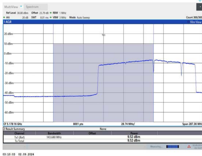
11BE160MIMO_Ant1_5250_UNII-2A_996+484+242_OFDMA_1
