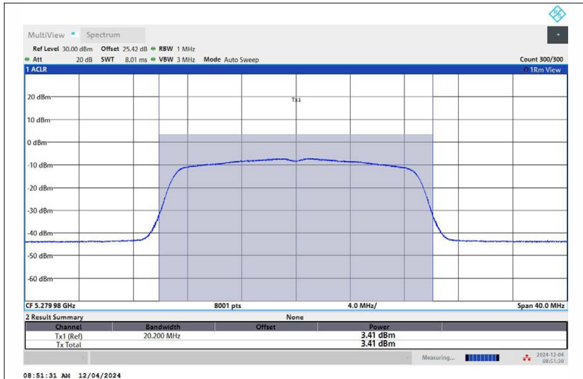
11AC20MIMO-Ant1-5280-TPC_L-PASS
