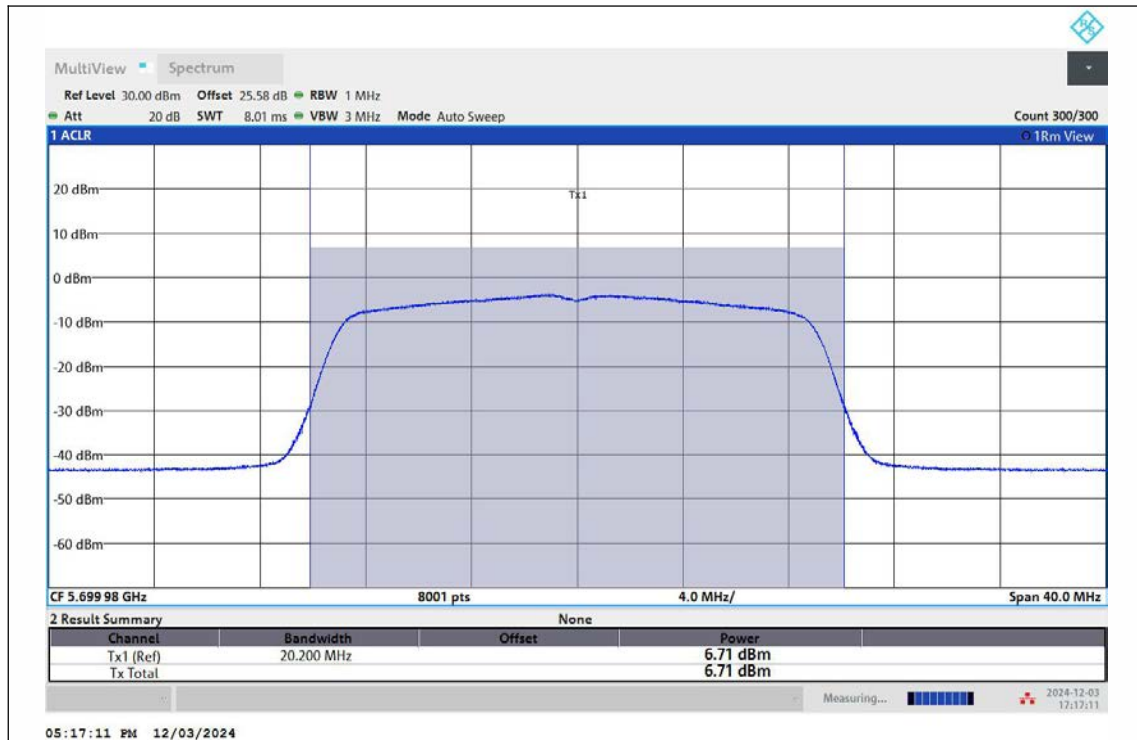
11AC20MIMO-Ant1-5700-TPC_H-PASS
