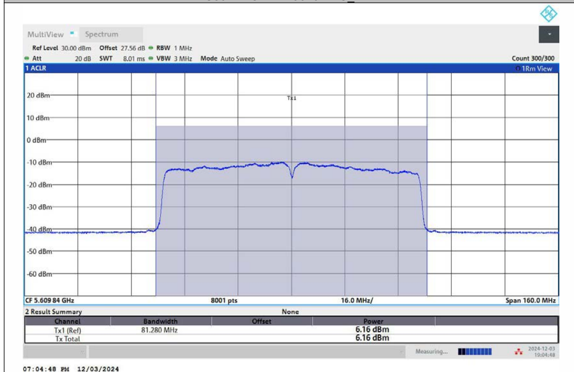
11AC80MIMO-Ant2-5610-TPC_H-PASS
