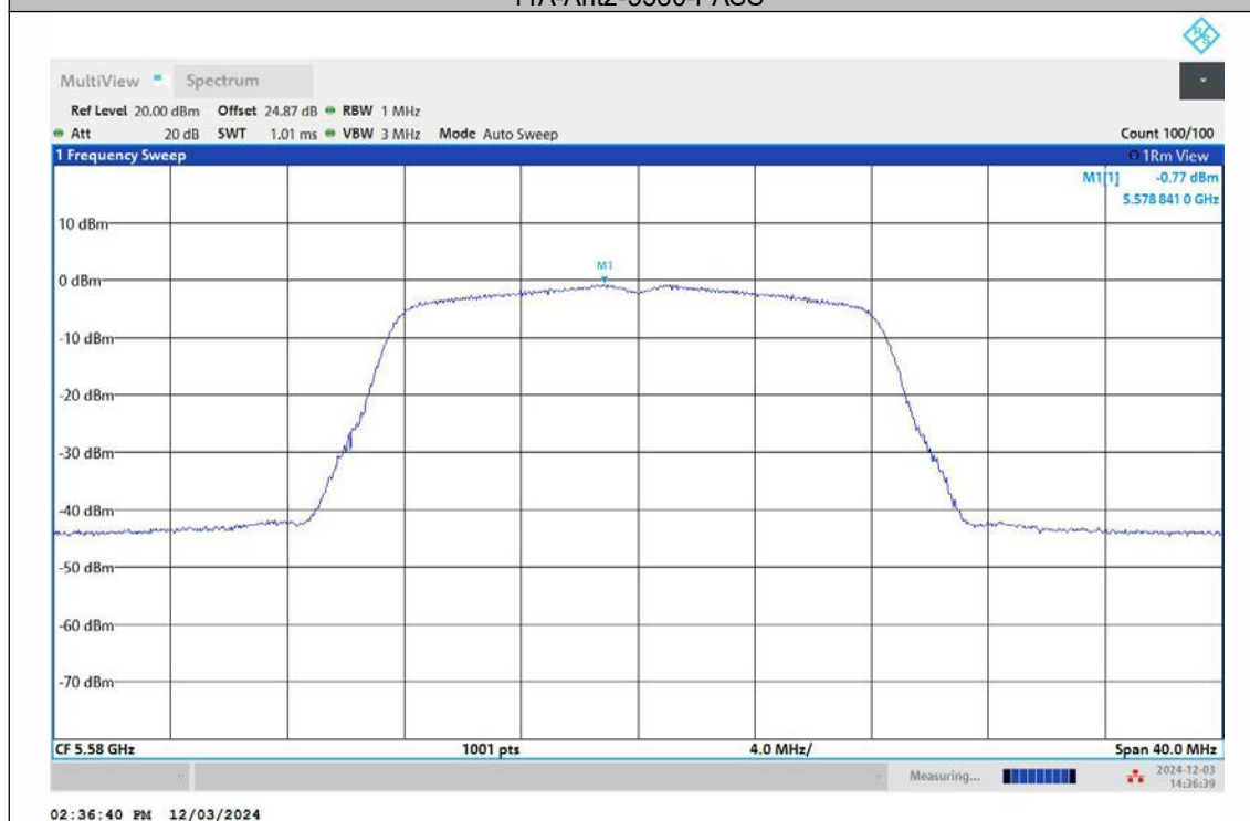
11A-Ant1-5580-PASS
