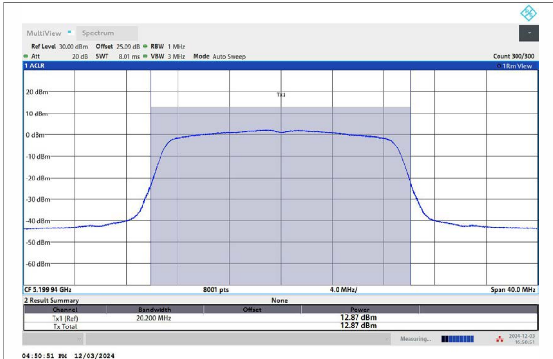
11AC20MIMO-Ant1-5200-PASS
