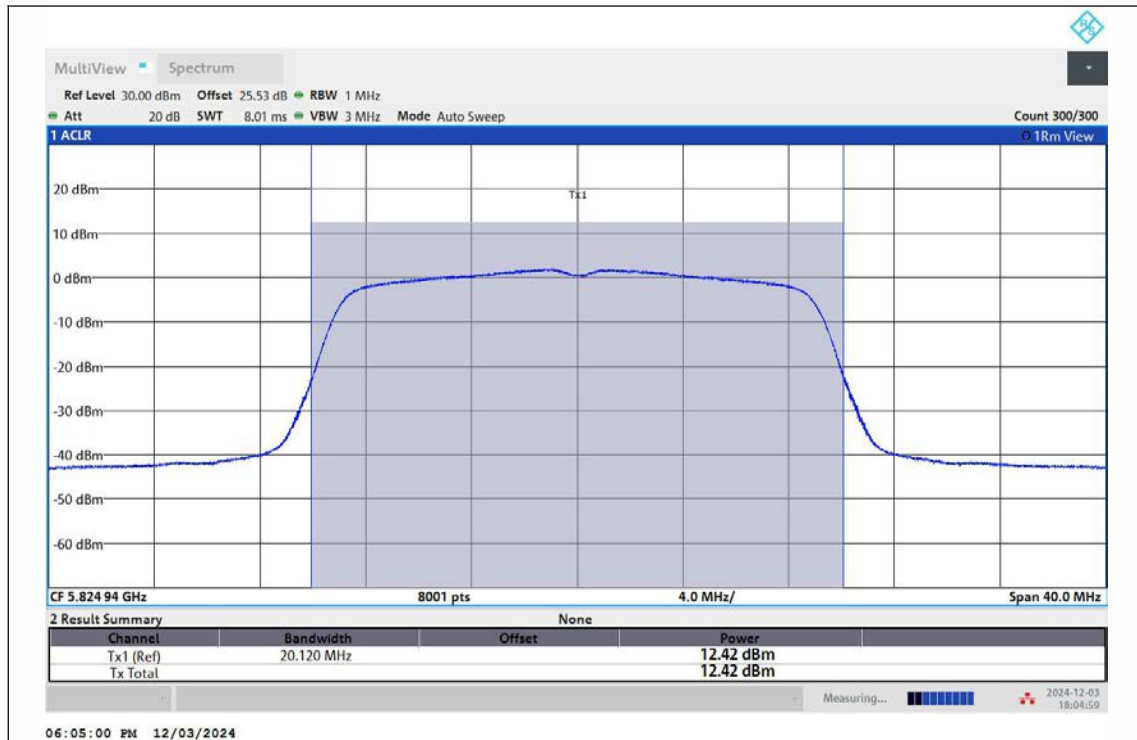
11AC20MIMO-Ant1-5825-PASS
