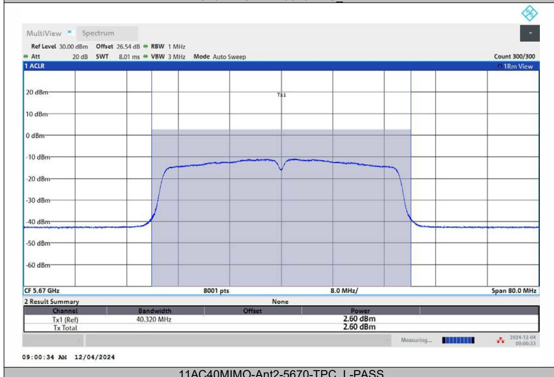
11AC40MIMO-Ant2-5670-TPC_L-PASS
