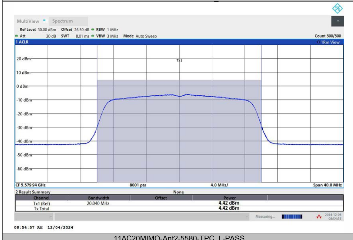
11AC20MIMO-Ant2-5580-TPC_L-PASS
