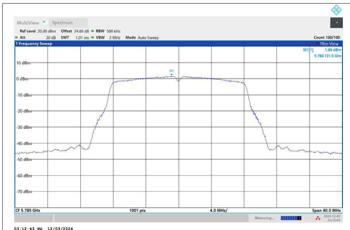
11A-Ant2-5785-PASS
