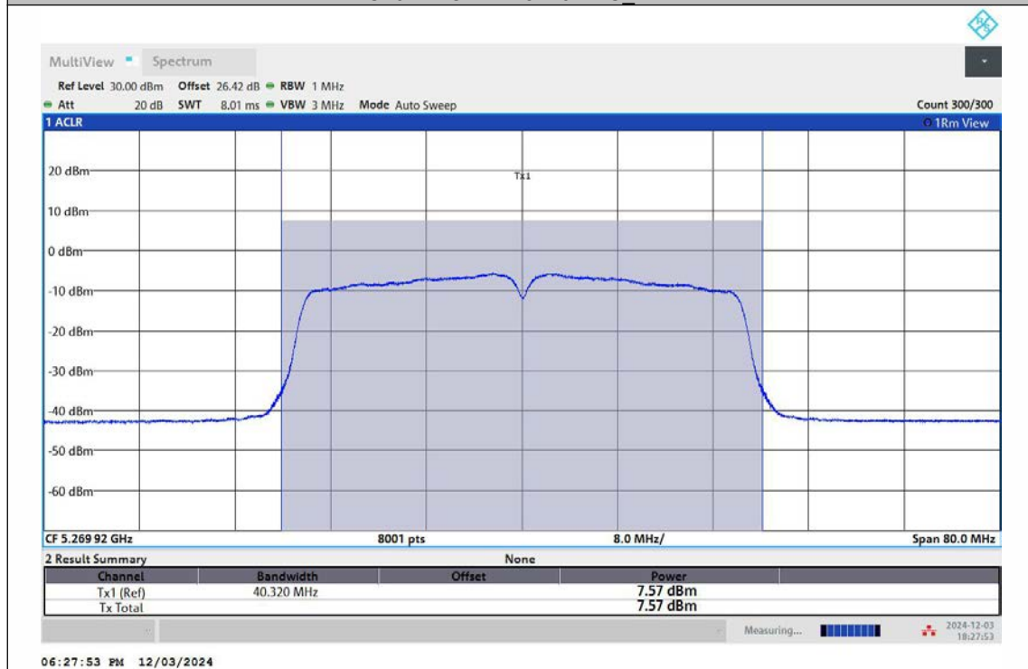
11AC40MIMO-Ant2-5270-TPC_H-PASS
