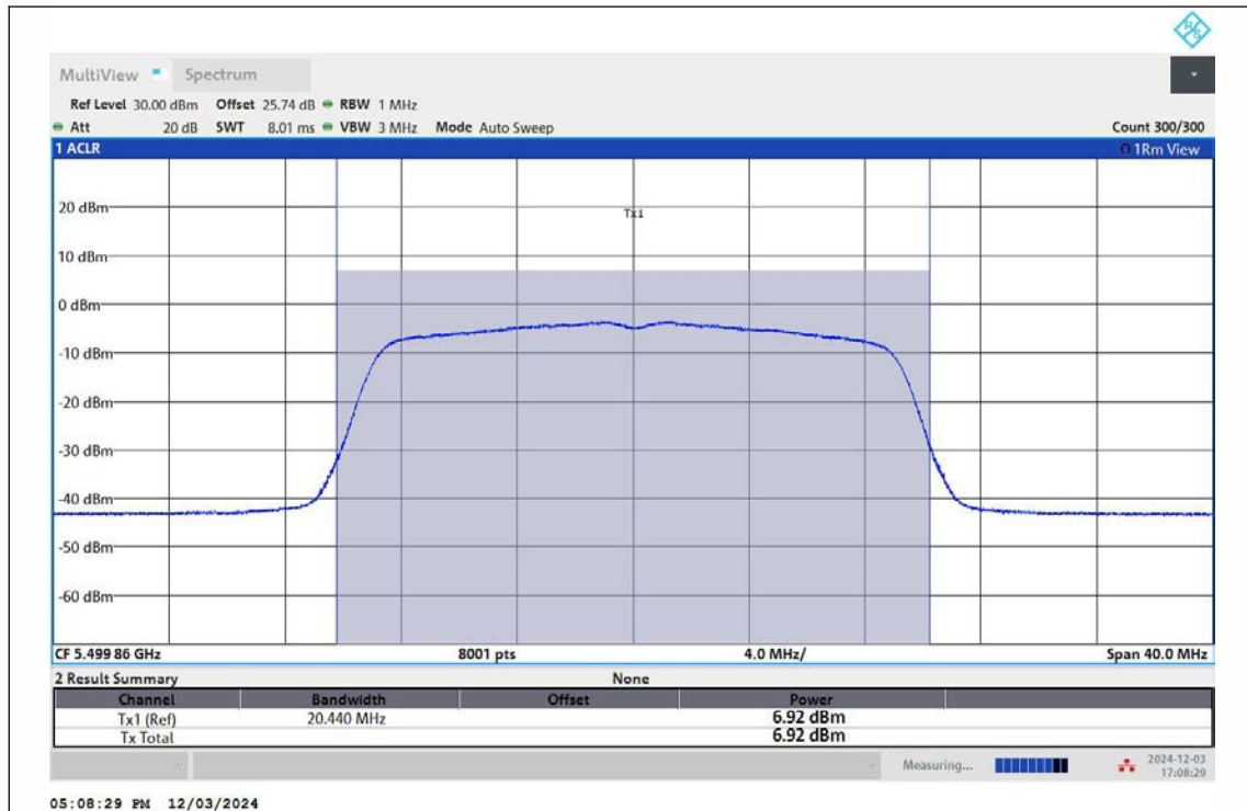
11AC20MIMO-Ant1-5500-TPC_H-PASS
