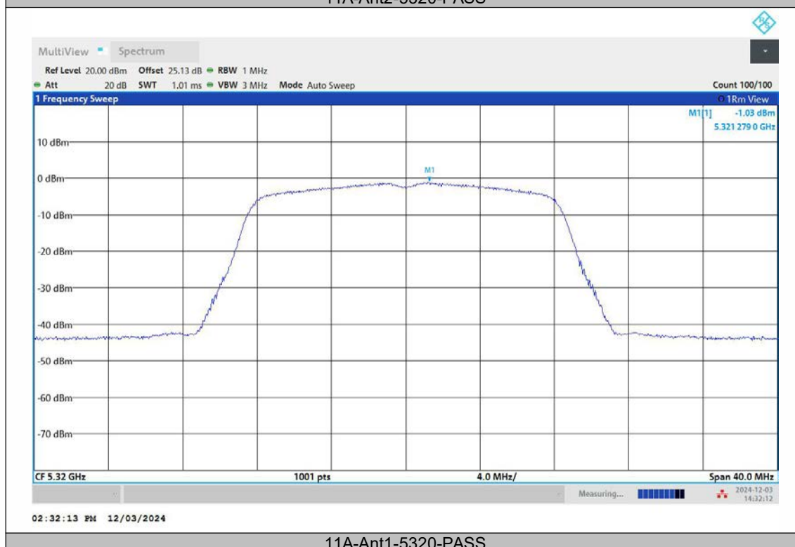
11A-Ant1-5320-PASS
