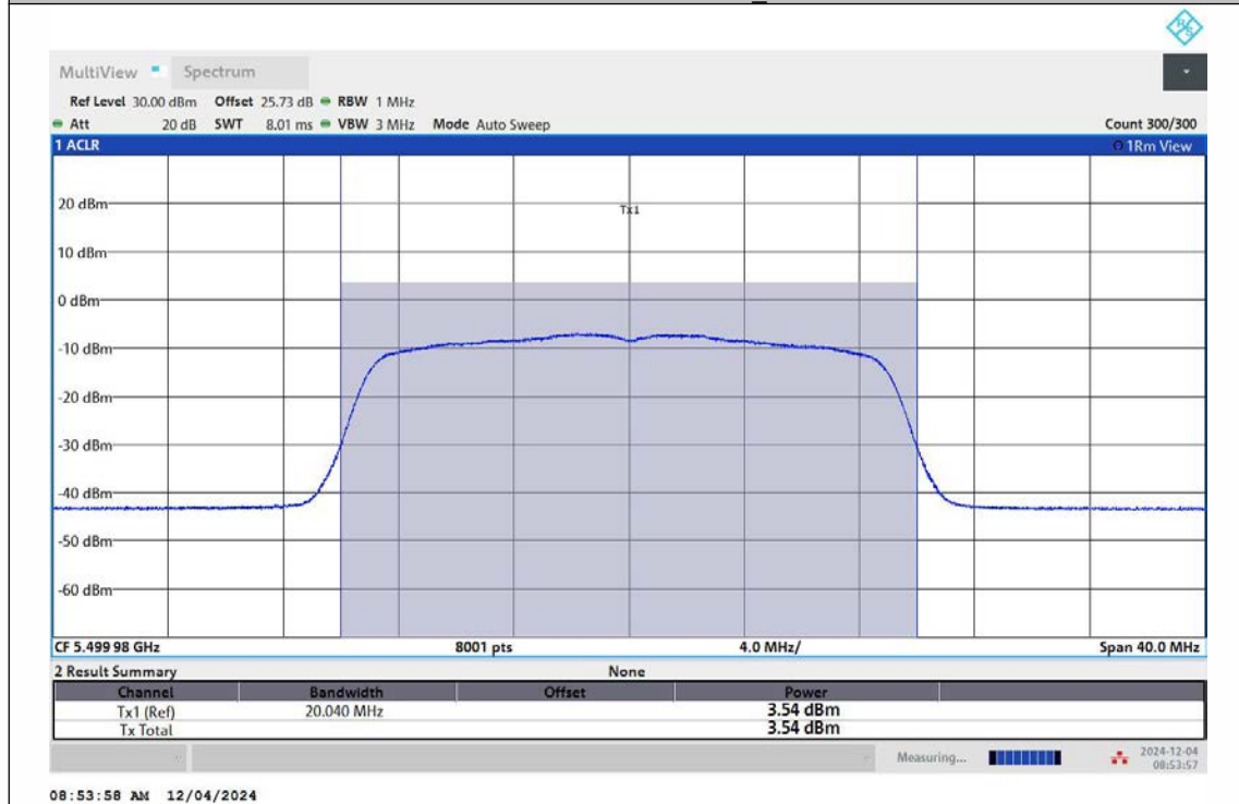
11AC20MIMO-Ant2-5500-TPC_L-PASS
