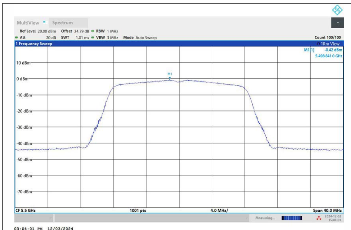
11A-Ant2-5500-PASS
