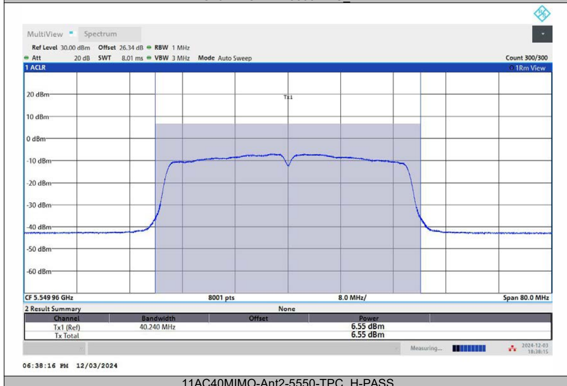
11AC40MIMO-Ant2-5550-TPC_H-PASS
