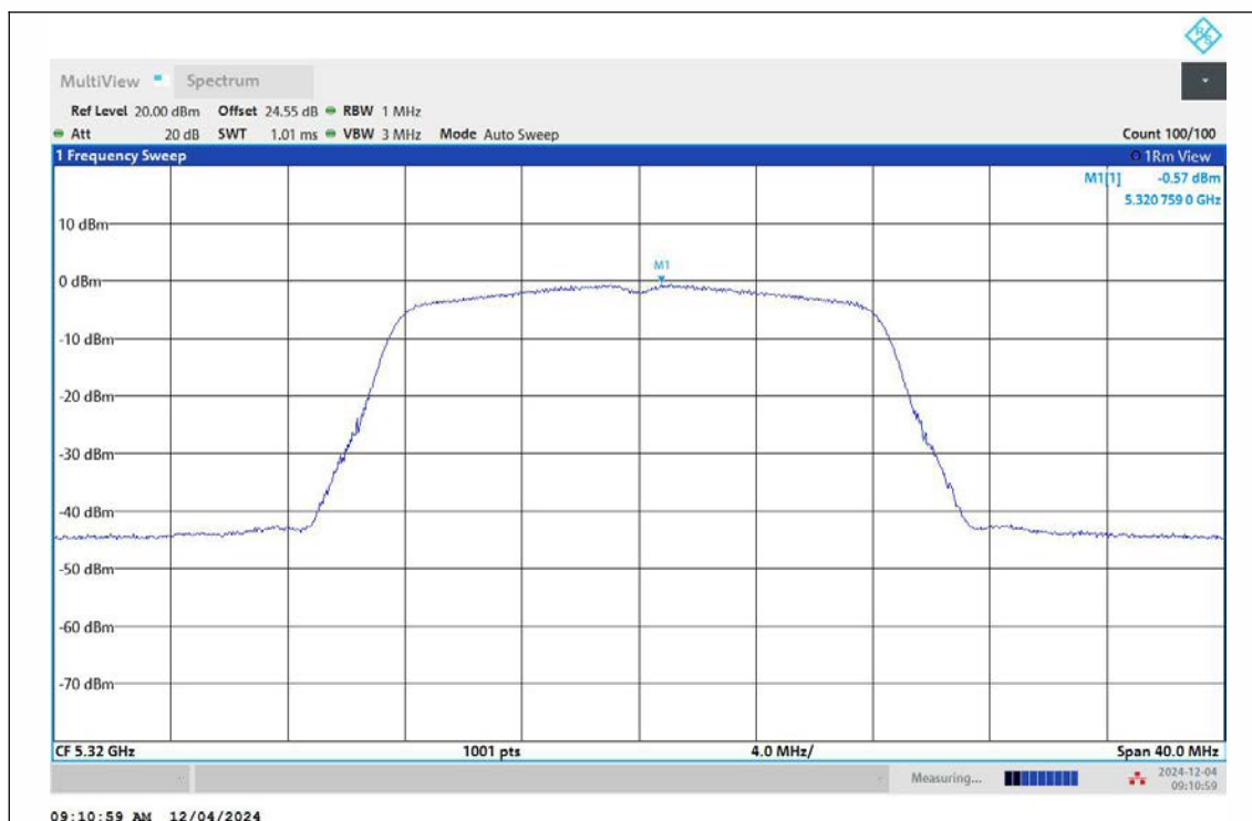
11A-Ant2-5320-PASS
