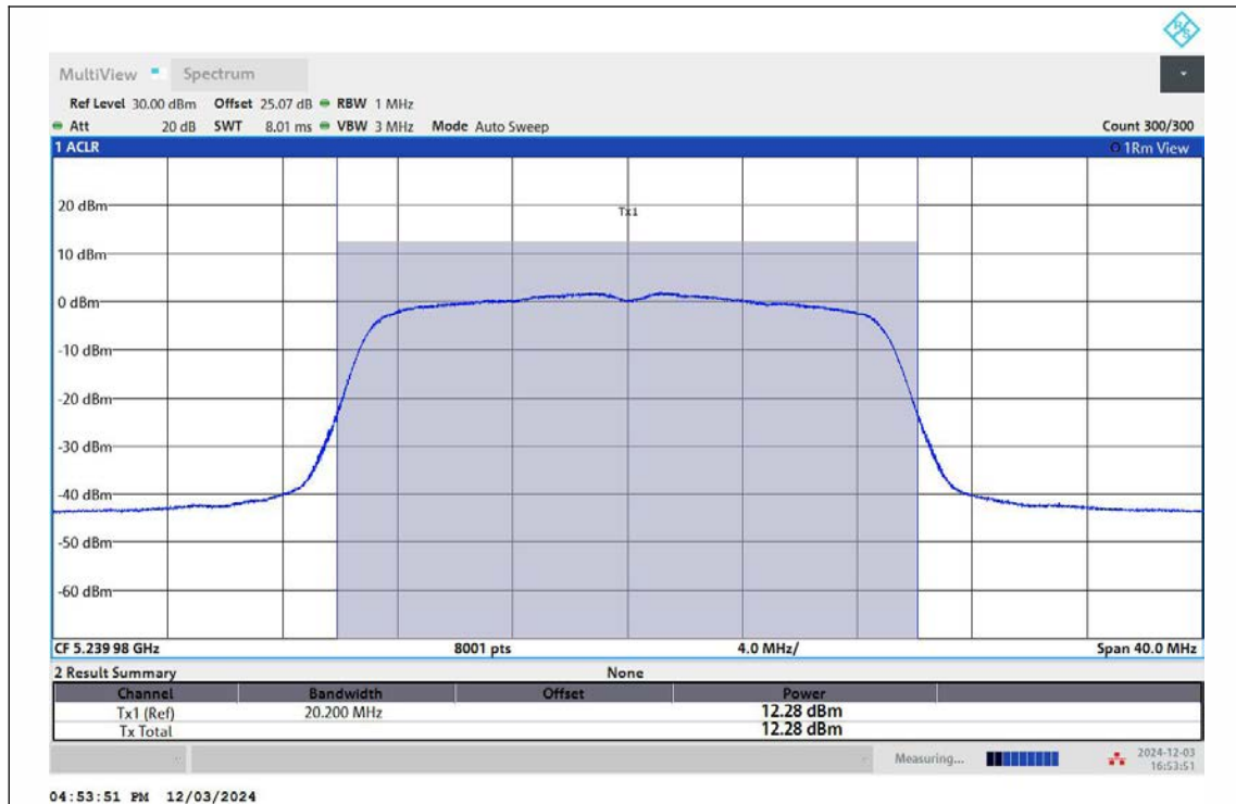
11AC20MIMO-Ant1-5240-PASS
