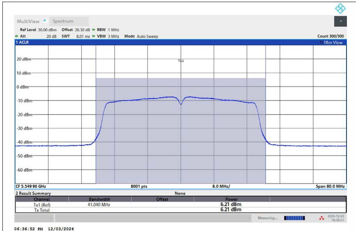
11AC40MIMO-Ant1-5550-TPC_H-PASS
