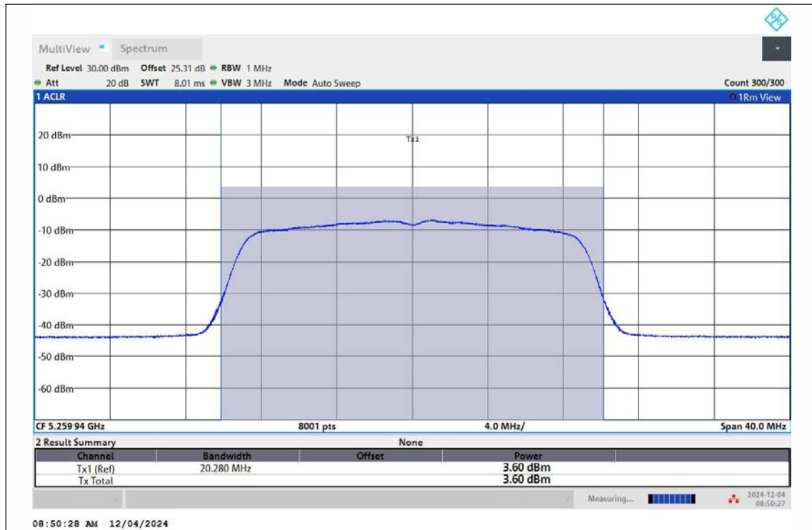
11AC20MIMO-Ant1-5260-TPC_L-PASS
