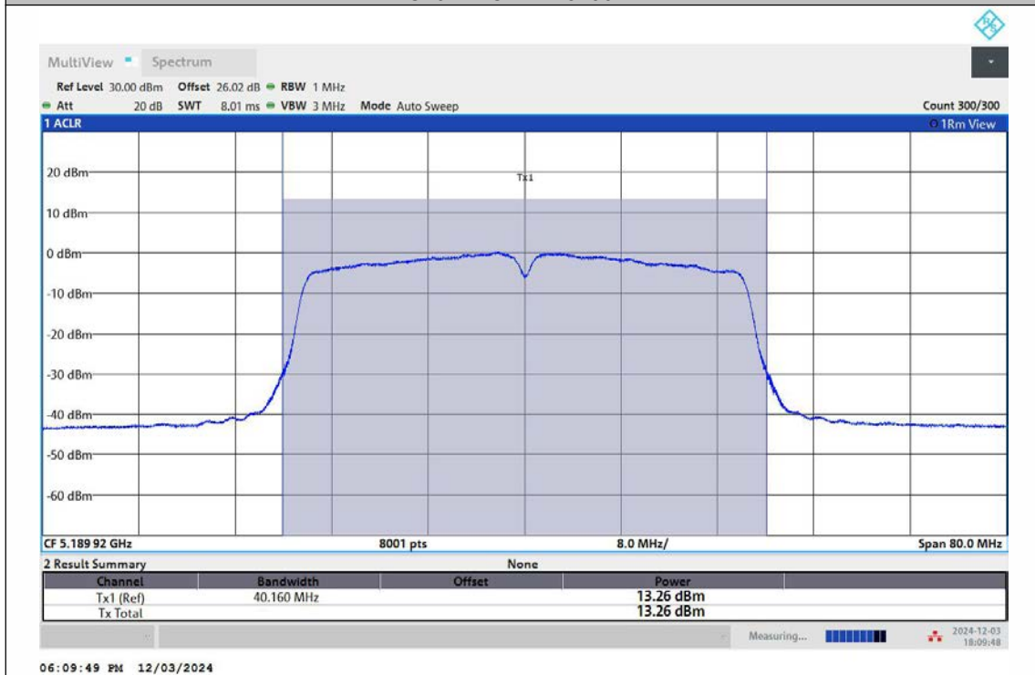
11AC40MIMO-Ant2-5190-PASS
