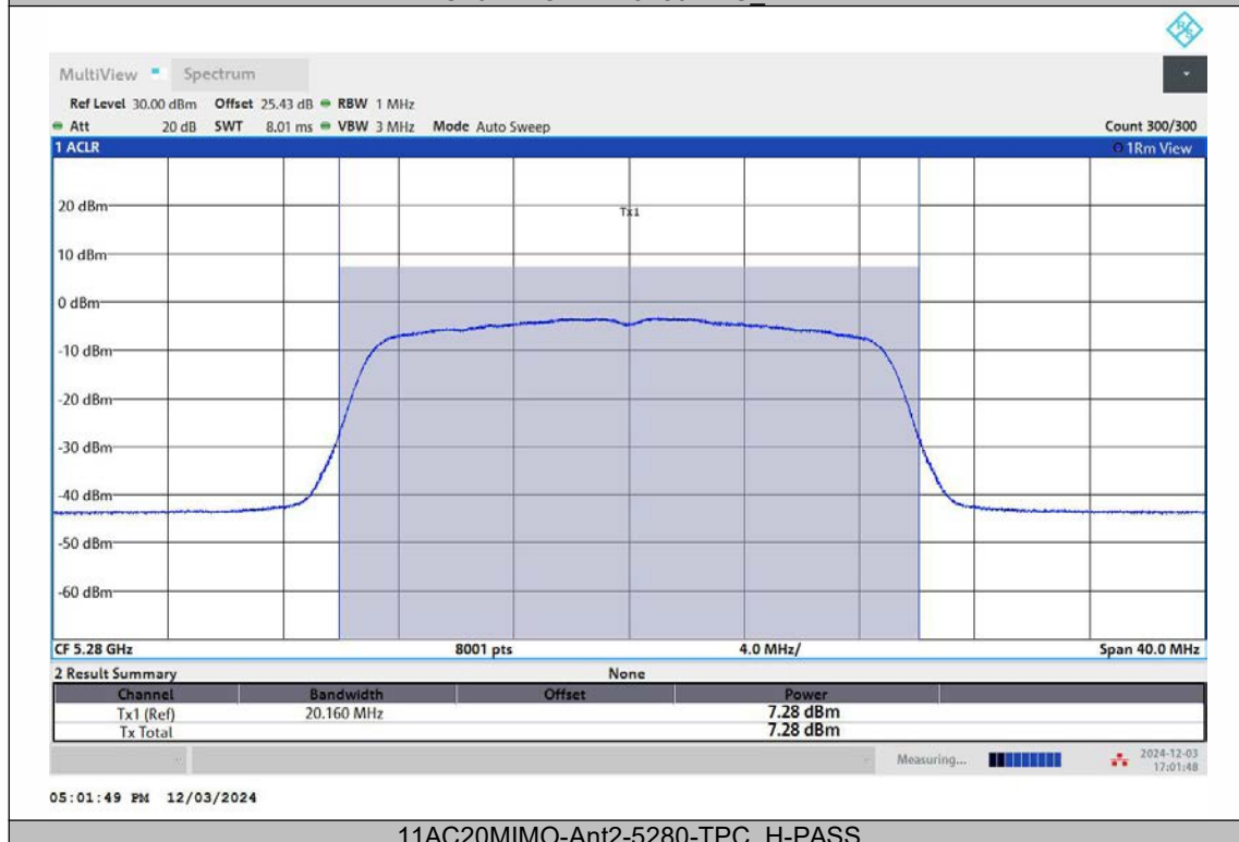
11AC20MIMO-Ant2-5280-TPC_H-PASS
