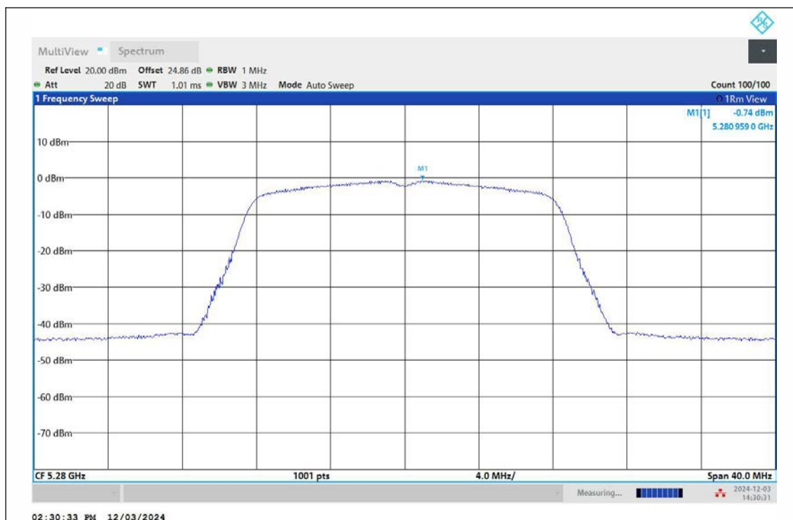
11A-Ant1-5280-PASS
