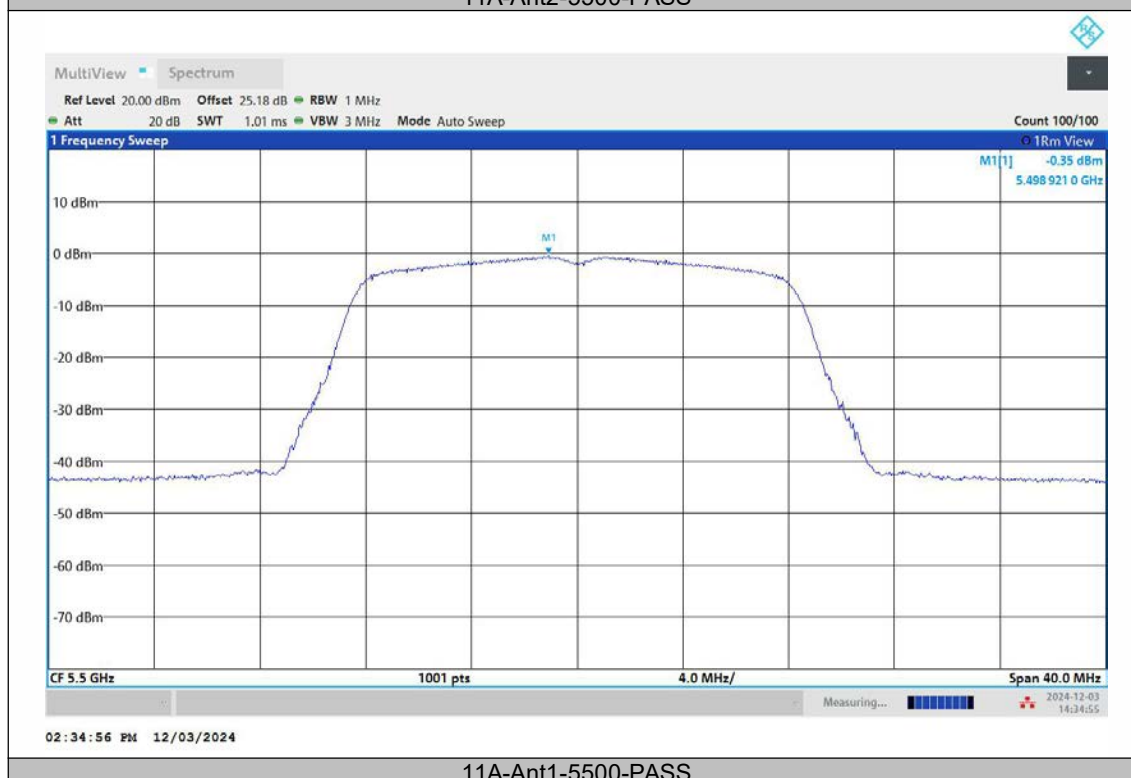
11A-Ant1-5500-PASS
