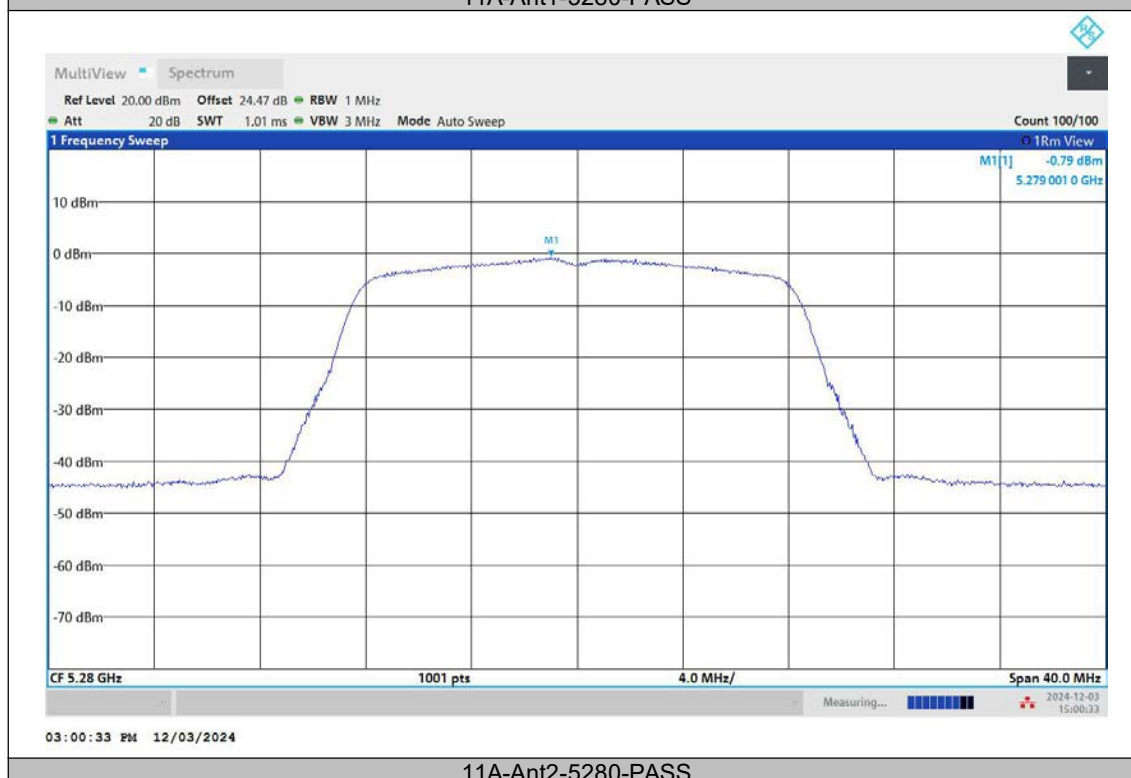
11A-Ant2-5280-PASS
