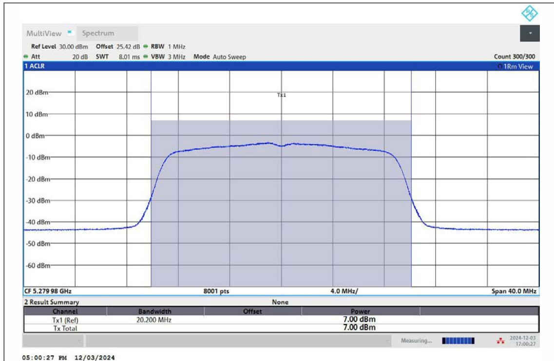
11AC20MIMO-Ant1-5280-TPC_H-PASS
