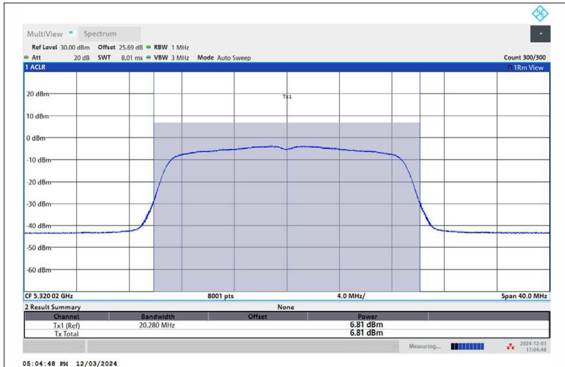
11AC20MIMO-Ant1-5320-TPC_H-PASS
