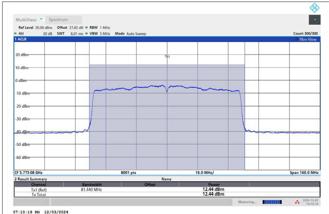
11AC80MIMO-Ant1-5775-PASS
