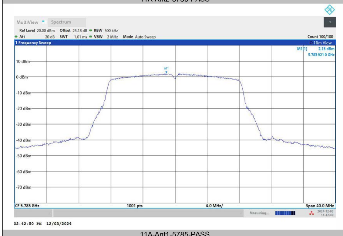
11A-Ant1-5785-PASS
