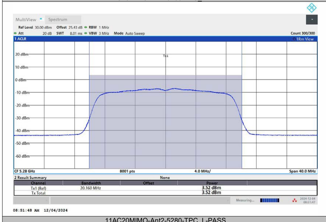
11AC20MIMO-Ant2-5280-TPC_L-PASS
