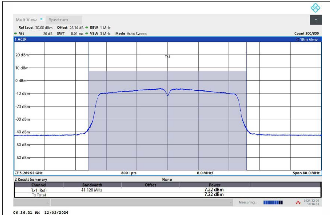
11AC40MIMO-Ant1-5270-TPC_H-PASS
