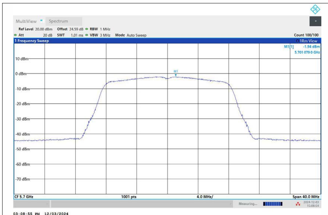
11A-Ant2-5700-PASS
