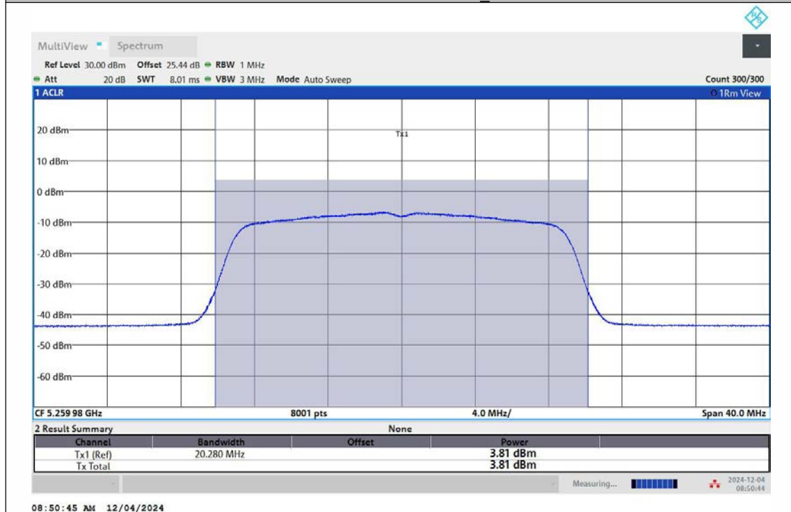
11AC20MIMO-Ant2-5260-TPC_L-PASS
