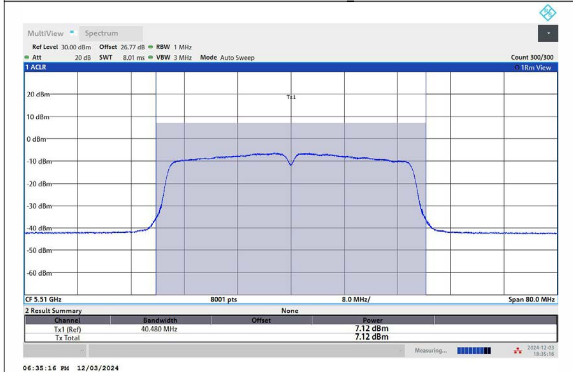
11AC40MIMO-Ant2-5510-TPC_H-PASS
