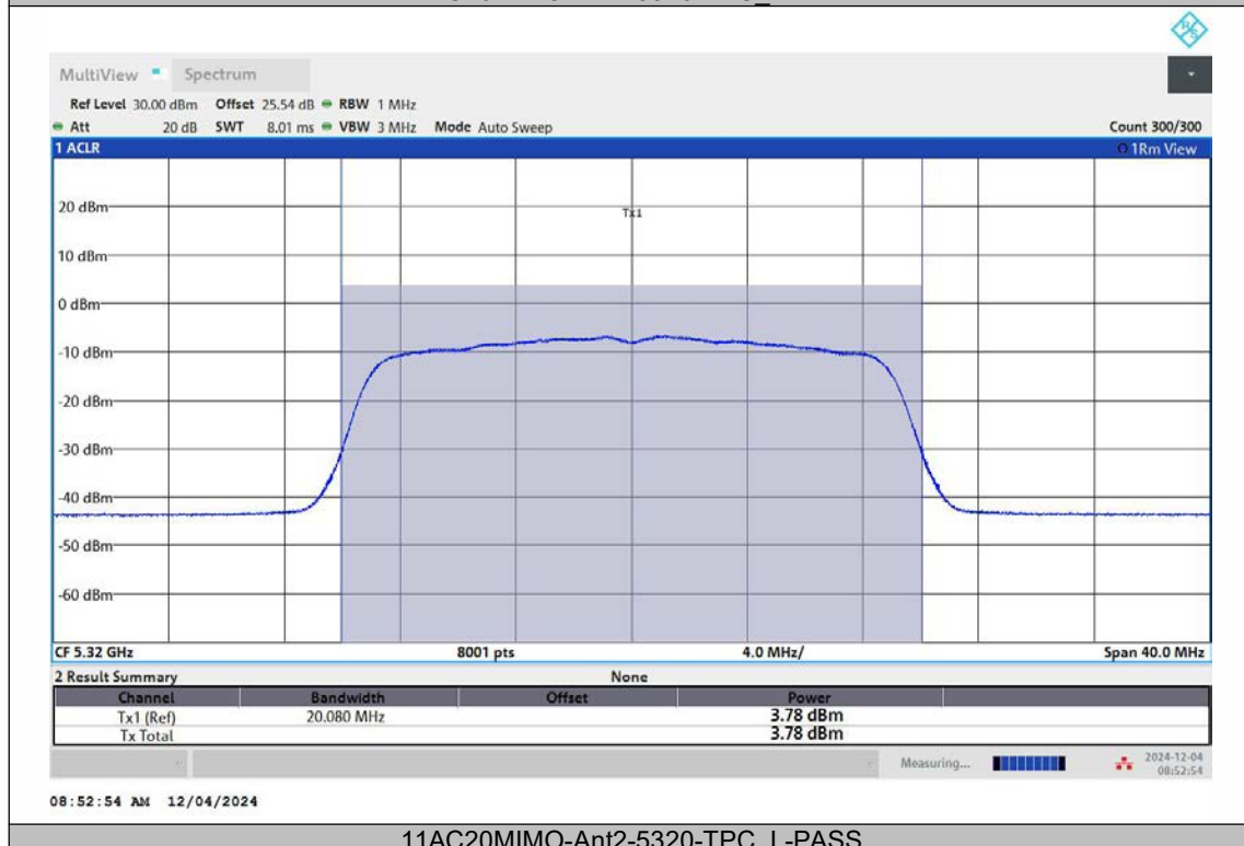
11AC20MIMO-Ant2-5320-TPC_L-PASS
