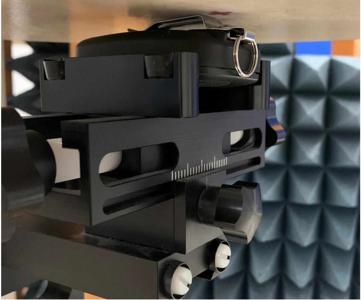
Belt Clip In Direct Contact with the Phantom
