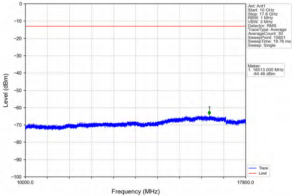
Band66_5MHz_16QAM_HCH_1777.5MHz_RB_1_0_NTNV
