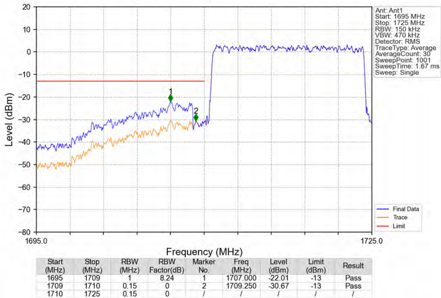
Band66_15MHz_16QAM_LCH_1717.5MHz_RB_75_0_NTNV
