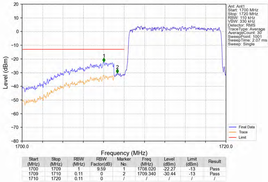
Band66_10MHz_16QAM_LCH_1715MHz_RB_50_0_NTNV
