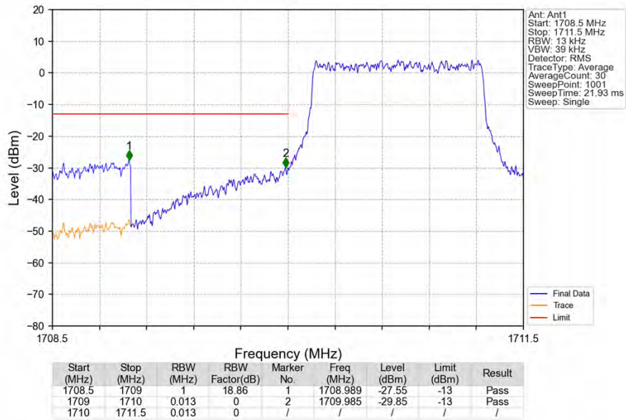
Band66_1.4MHz_16QAM_LCH_1710.7MHz_RB_6_0_NTNV
