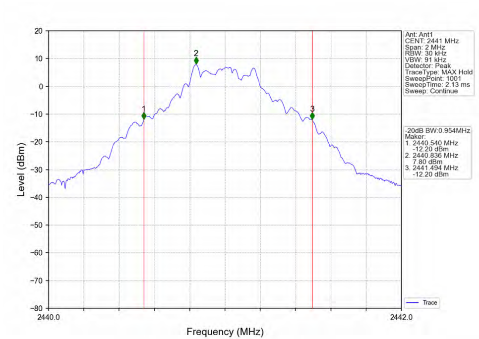
GFSK_DH5_MCH_2441MHz_Ant1_NTNV
