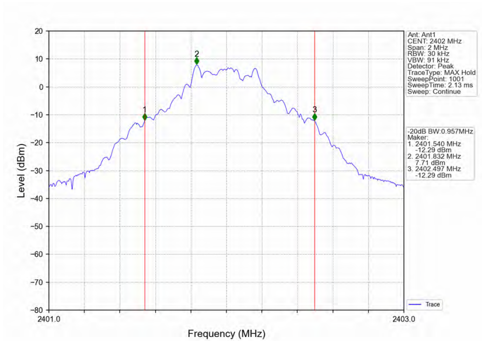
GFSK_DH5_LCH_2402MHz_Ant1_NTNV
