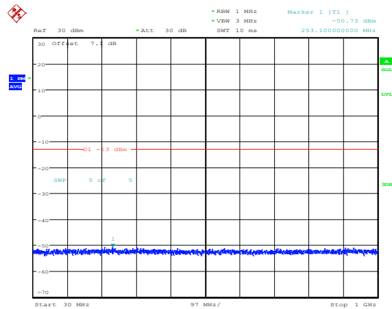
Band2-1.4MHz-QPSK-18900-1RB#0-Range3:30~1000MHz
