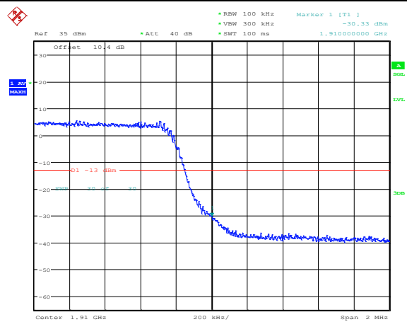
Band2-5MHz-16QAM-19175-25RB#0
