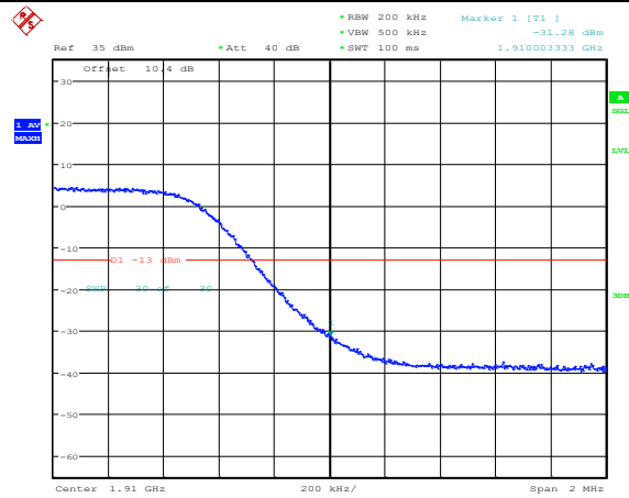
Band2-10MHz-16QAM-19150-50RB#0
