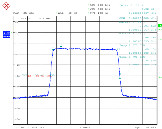
Band2-10MHz-16QAM-19150-50RB#0
