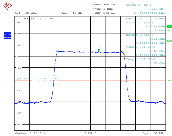
Band2-15MHz-16QAM-18900-75RB#0
