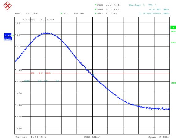
Band2-10MHz-16QAM-19150-1RB#49
