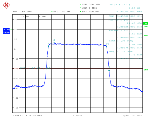
Band2-15MHz-16QAM-19125-75RB#0
