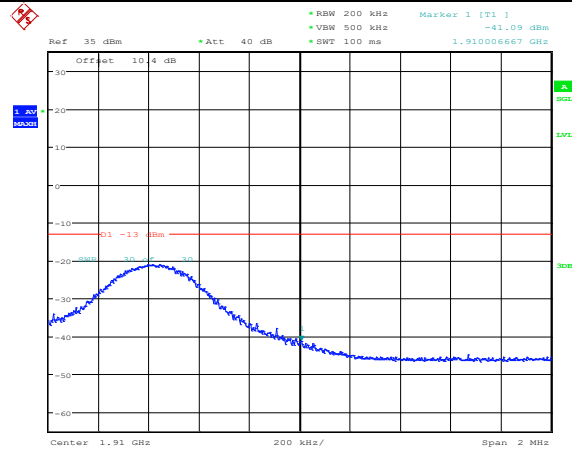
Band2-10MHz-16QAM-19150-1RB#49
