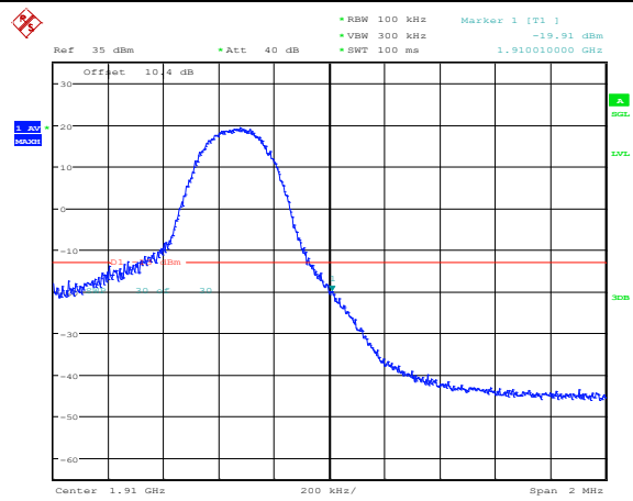
Band2-5MHz-16QAM-19175-1RB#24
