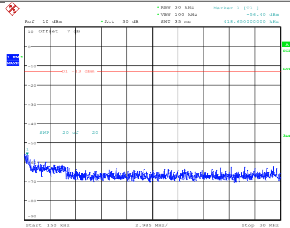
Band5-4233-1-0.15~30MHz
