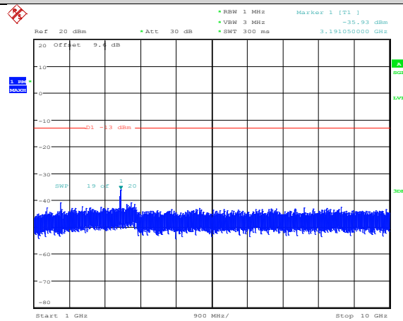
Band5-4182-4-1000~10000MHz
