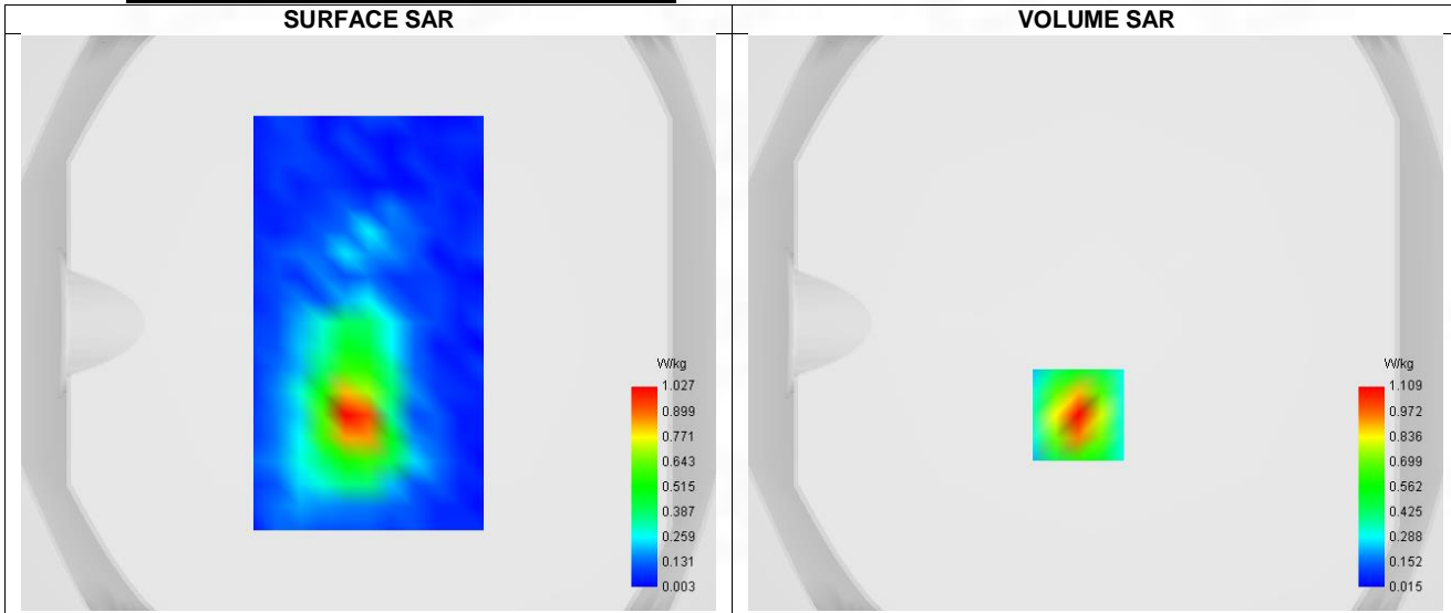
Maximum location: X=-6.00, Y=-32.00 ; SAR Peak: 1.84 W/kg
