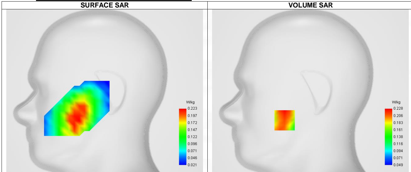
Maximum location: X=-41.00, Y=-47.00 ; SAR Peak: 0.30 W/kg
