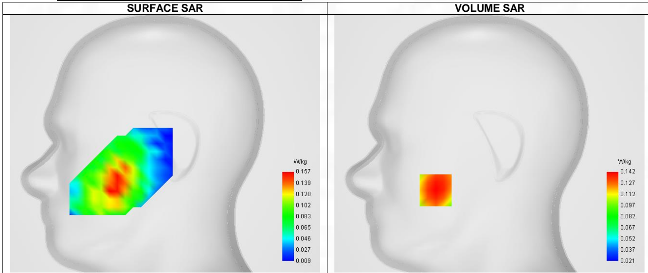
Maximum location: X=-54.00, Y=-47.00 ; SAR Peak: 0.17 W/kg
