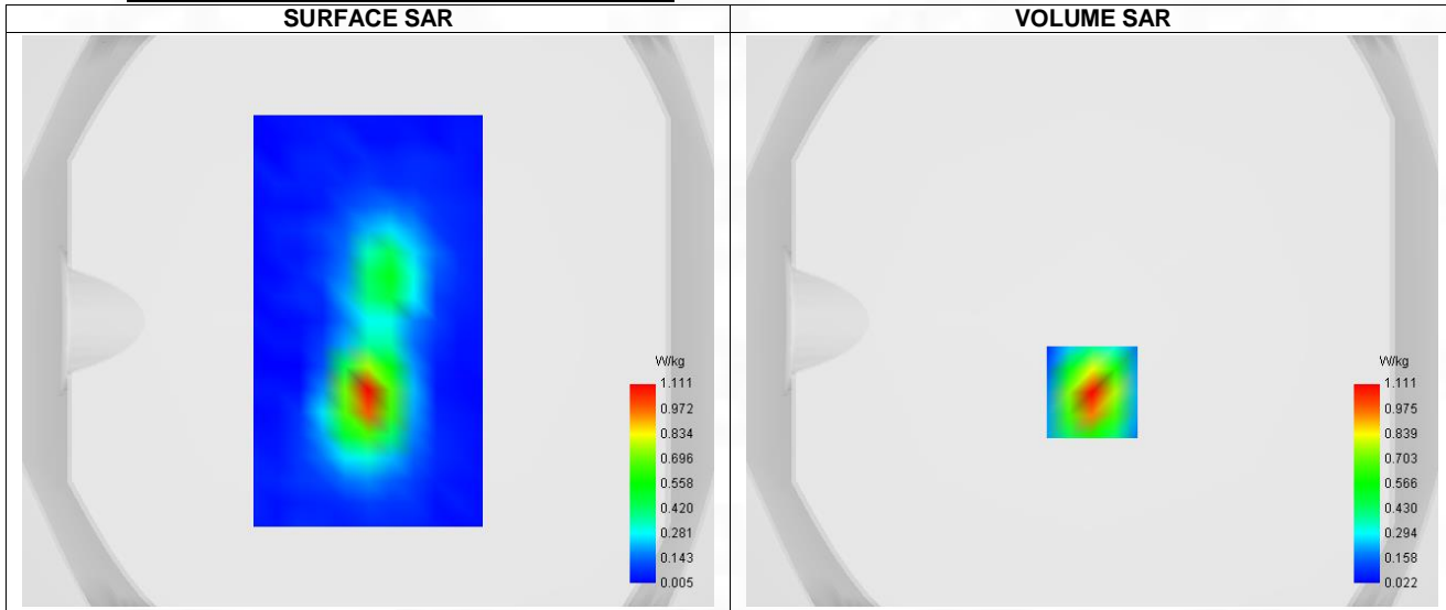
Maximum location: X=0.00, Y=-25.00 ; SAR Peak: 1.89 W/kg
