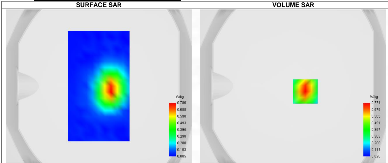
Maximum location: X=16.00, Y=-7.00 ; SAR Peak: 1.16 W/kg
