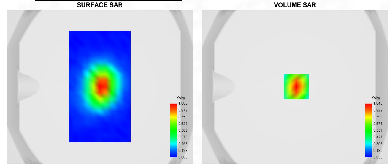
Maximum location: X=2.00, Y=0.00 ; SAR Peak: 1.57 W/kg
