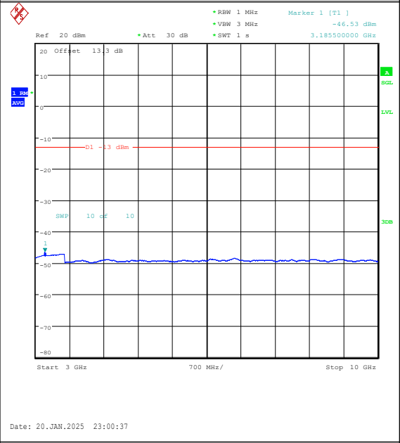
Band5-3MHz-QPSK-20525-1RB#14-3000~10000- PASS
