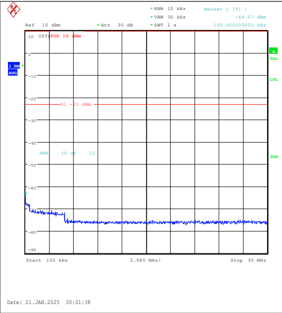
Band5-5MHz-QPSK-20625-25RB#0-0.15~30-PAS S
