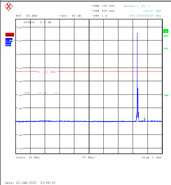
Band5-5MHz-QPSK-20525-1RB#0-30~1000-PAS S
