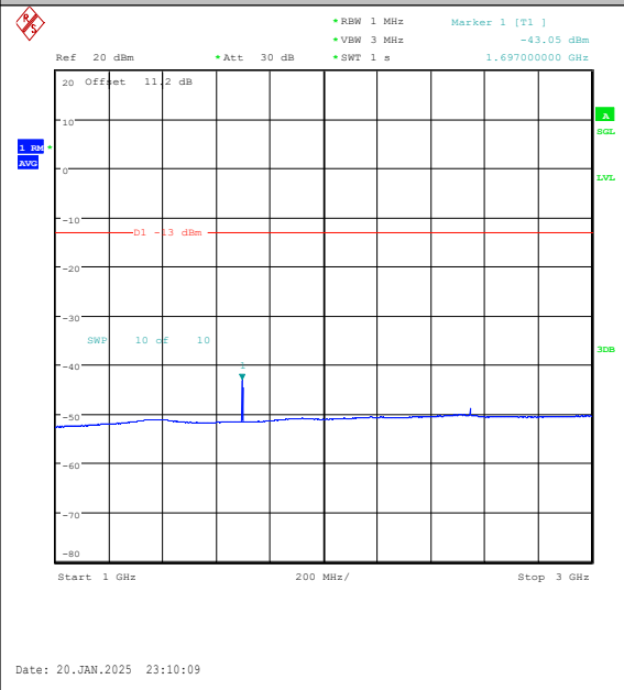
Band5-3MHz-16QAM-20635-1RB#14-1000~3000-PASS
