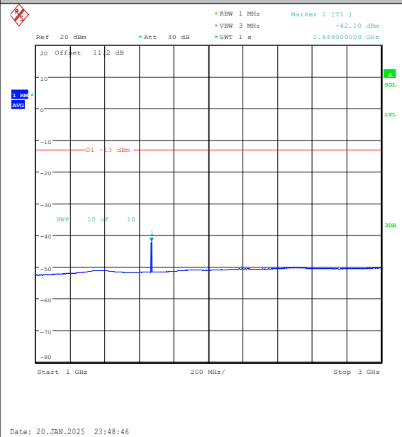
Band5-5MHz-QPSK-20525-1RB#0-1000~3000-PA SS
