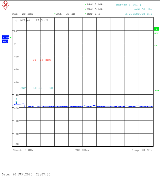
Band5-3MHz-16QAM-20635-1RB#0-3000~10000- PASS
