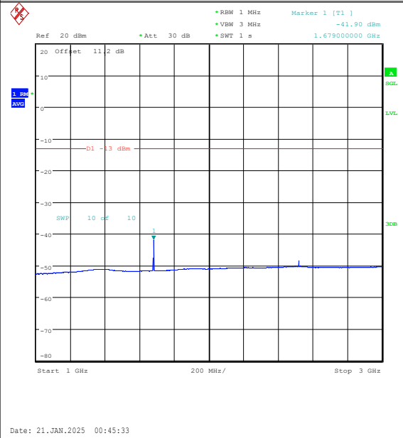
Band5-10MHz-QPSK-20600-1RB#0-1000~3000-P ASS
