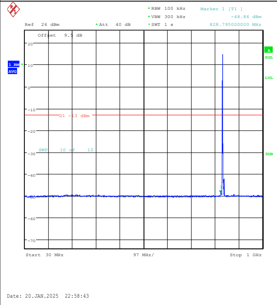
Band5-3MHz-16QAM-20525-1RB#0-30~1000-PA SS
