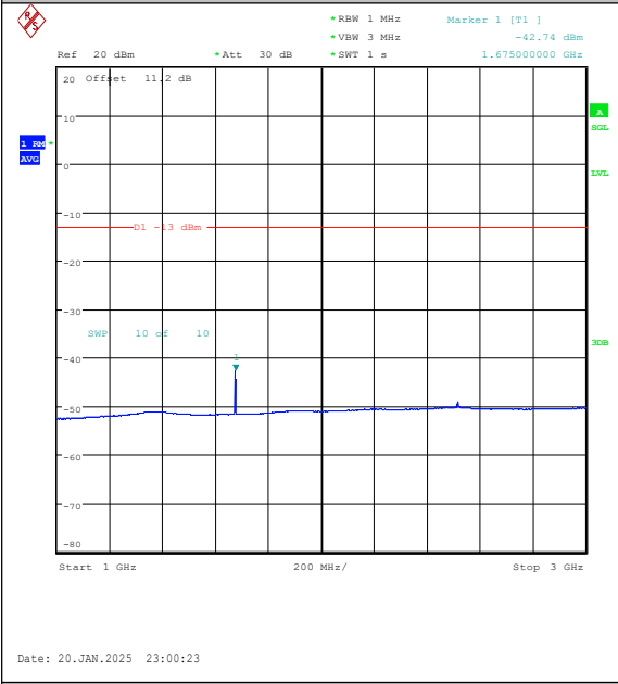
Band5-3MHz-QPSK-20525-1RB#14-1000~3000-P ASS
