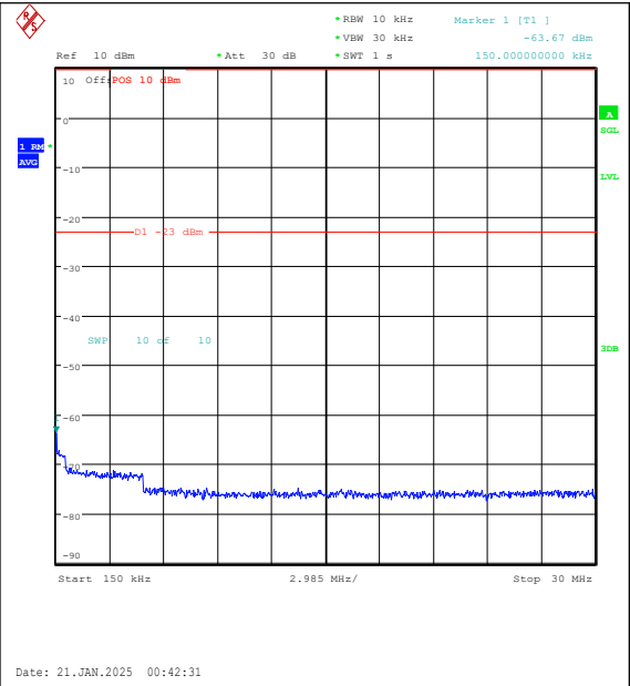
Band5-10MHz-QPSK-20525-50RB#0-0.15~30-PA-SS
