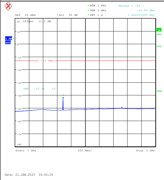
Band5-10MHz-QPSK-20525-1RB#49-1000~3000- PASS
