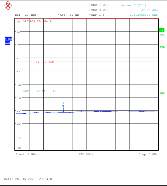
Band5-5MHz-QPSK-20525-25RB#0-1000~3000-P ASS
