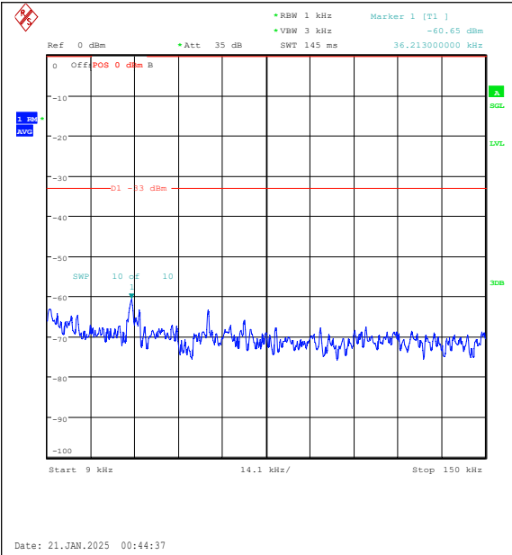
Band5-10MHz-QPSK-20600-1RB#0-0.009~0.15-P ASS
