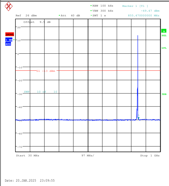
Band5-3MHz-16QAM-20635-1RB#14-30~1000-PA-SS
