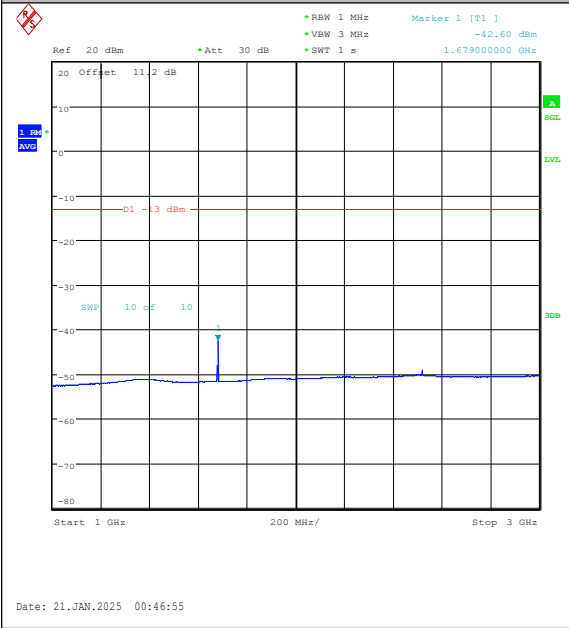
Band5-10MHz-16QAM-20600-1RB#0-1000~3000- PASS
