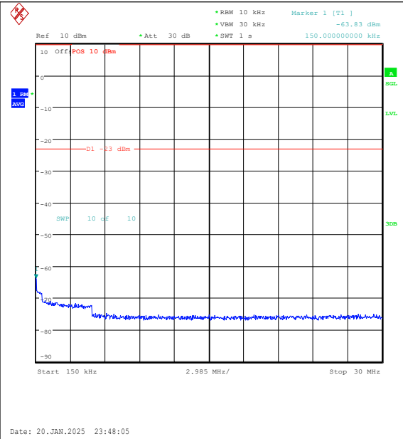
Band5-5MHz-QPSK-20525-1RB#0-0.15~30-PASS
