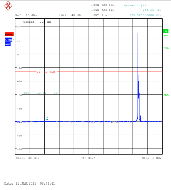
Band5-10MHz-16QAM-20600-1RB#0-30~1000-PA SS
