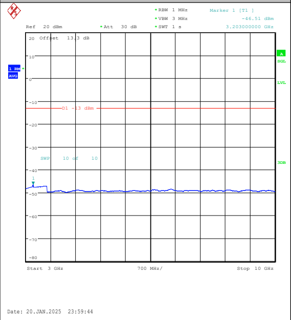
Band5-5MHz-QPSK-20625-1RB#24-3000~10000- PASS
