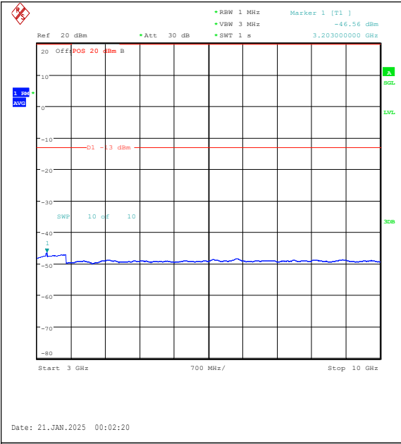
Band5-5MHz-QPSK-20625-25RB#0-3000~10000-PASS
