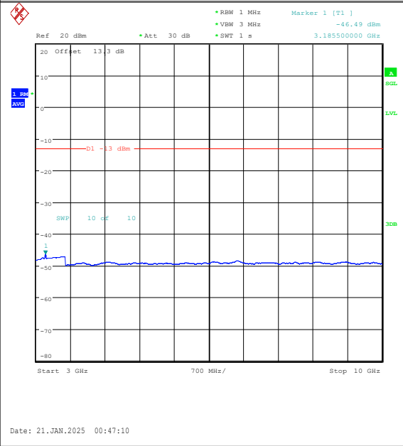
Band5-10MHz-16QAM-20600-1RB#0-3000~1000 0-PASS
