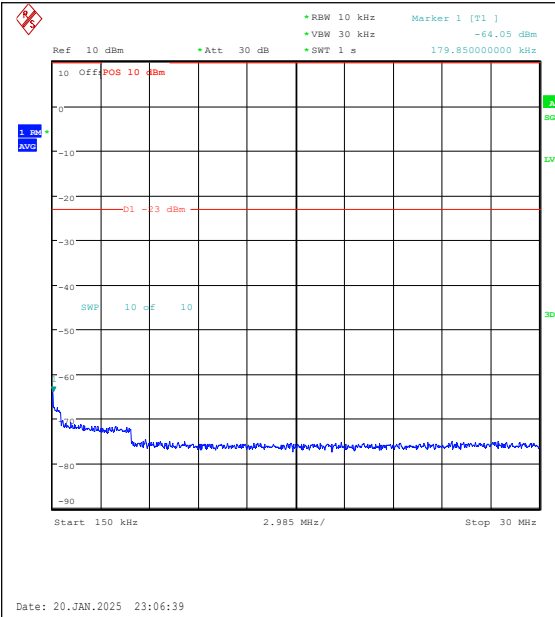
Band5-3MHz-16QAM-20635-1RB#0-0.15~30-PAS S
