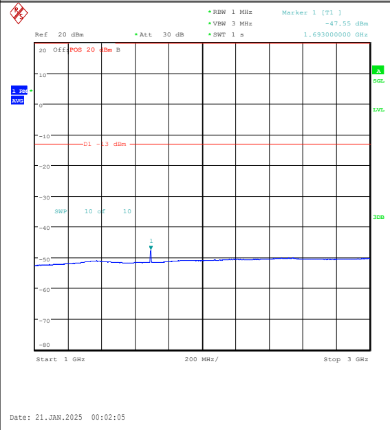
Band5-5MHz-QPSK-20625-25RB#0-1000~3000-P ASS
