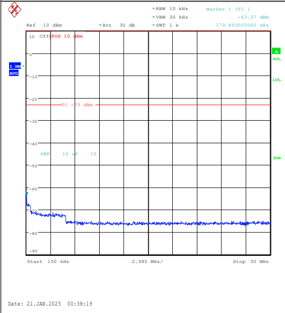
Band5-10MHz-16QAM-20525-1RB#0-0.15~30-PA SS
