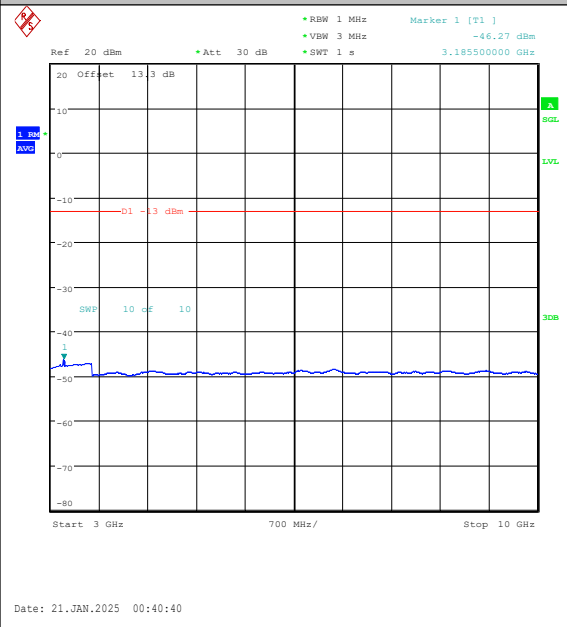
Band5-10MHz-QPSK-20525-1RB#49-3000~1000 0-PASS
