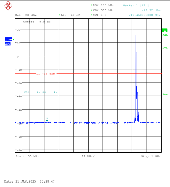
Band5-10MHz-16QAM-20525-1RB#0-30~1000-PA SS
