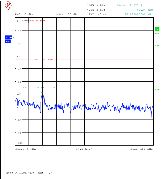
Band5-5MHz-QPSK-20625-25RB#0-0.009~0.15-P ASS
