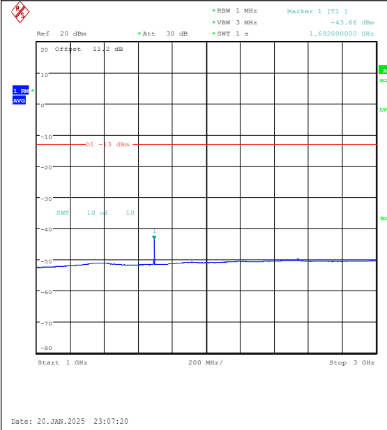
Band5-3MHz-16QAM-20635-1RB#0-1000~3000-P ASS
