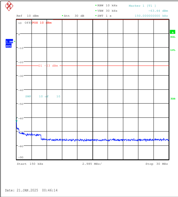
Band5-10MHz-16QAM-20600-1RB#0-0.15~30-PA SS
