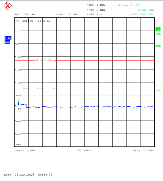
Band5-10MHz-16QAM-20525-1RB#0-3000~1000-0-PASS
