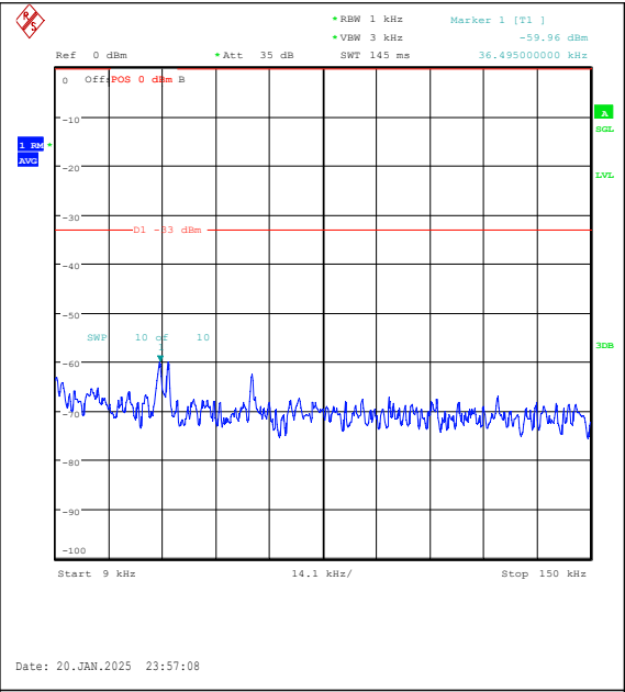
Band5-5MHz-16QAM-20625-1RB#0-0.009~0.15-P ASS
