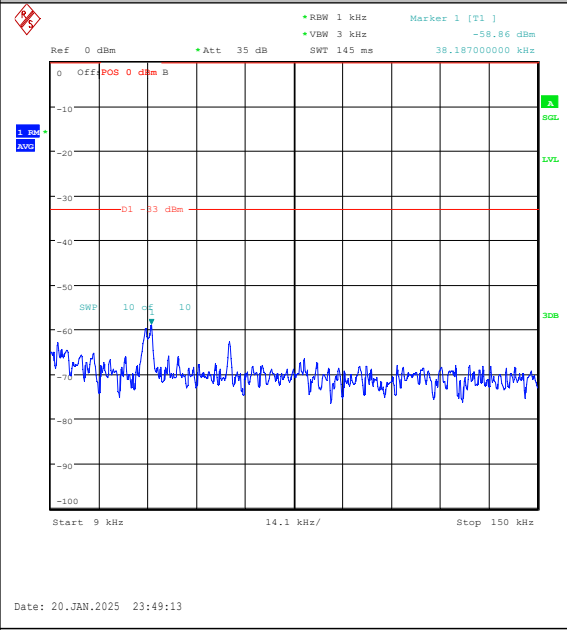
Band5-5MHz-16QAM-20525-1RB#0-0.009~0.15-P ASS
