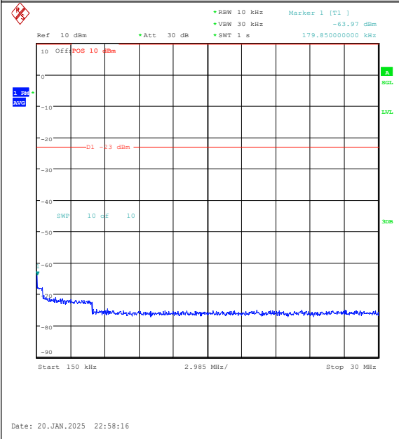
Band5-3MHz-16QAM-20525-1RB#0-0.15~30-PAS S
