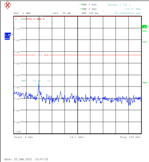
Band5-5MHz-QPSK-20525-1RB#0-0.009~0.15-PA SS
