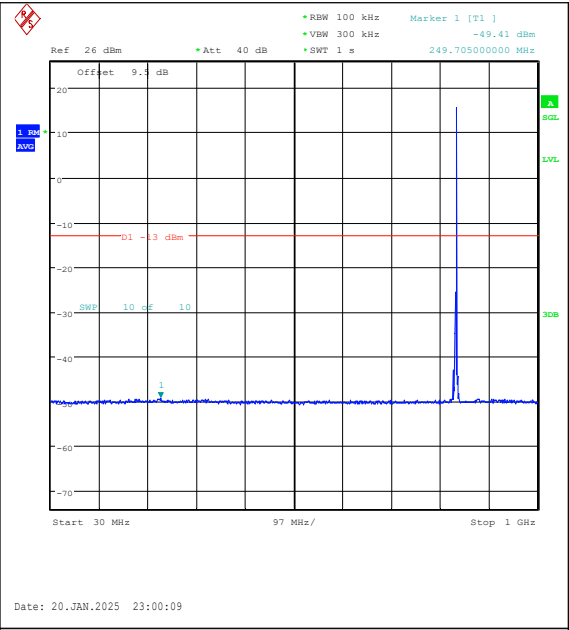
Band5-3MHz-QPSK-20525-1RB#14-30~1000-PA SS
