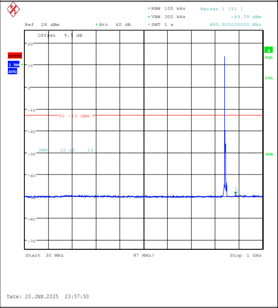
Band5-5MHz-16QAM-20625-1RB#0-30~1000-PA SS
