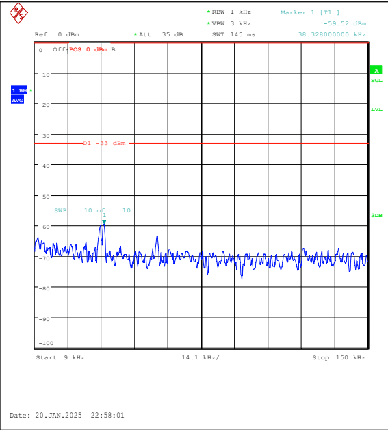
Band5-3MHz-16QAM-20525-1RB#0-0.009~0.15-P ASS
