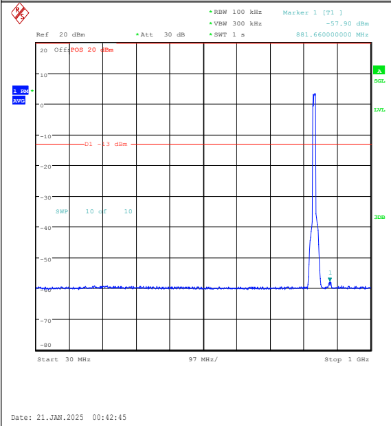
Band5-10MHz-QPSK-20525-50RB#0-30~1000-PA-SS
