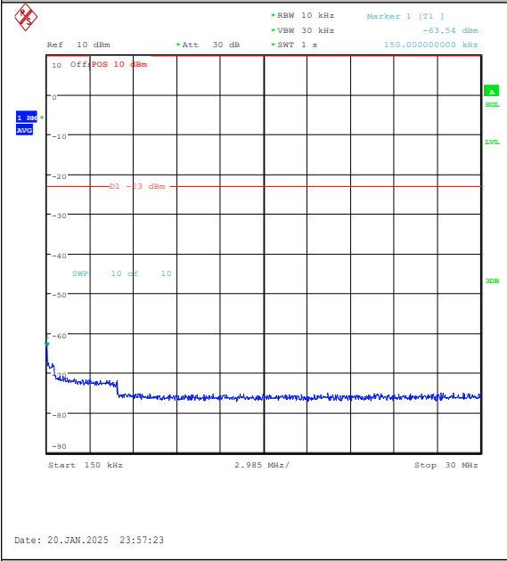
Band5-5MHz-16QAM-20625-1RB#0-0.15~30-PAS S
