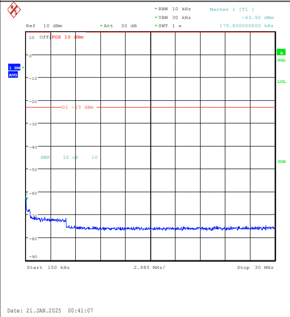
Band5-10MHz-16QAM-20525-1RB#49-0.15~30-PASS
