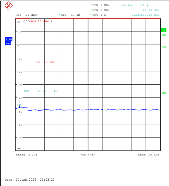
Band5-3MHz-QPSK-20525-15RB#0-3000~10000-PASS
