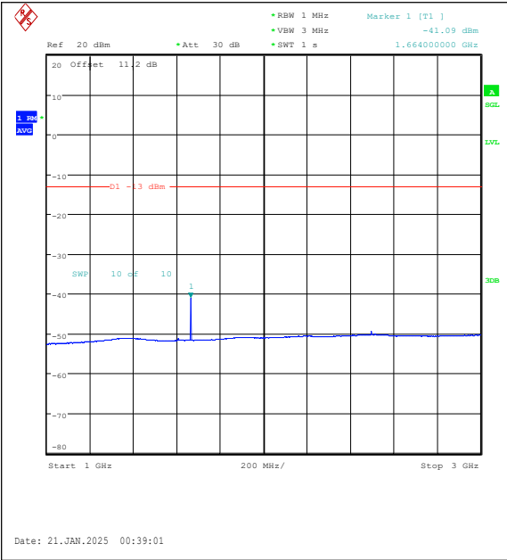
Band5-10MHz-16QAM-20525-1RB#0-1000~3000-PASS
