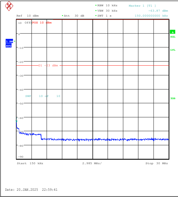
Band5-3MHz-QPSK-20525-1RB#14-0.15~30-PAS S
