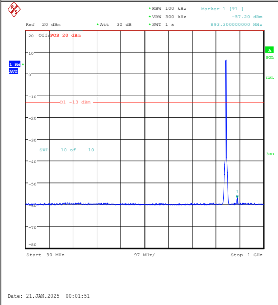
Band5-5MHz-QPSK-20625-25RB#0-30~1000-PA SS
