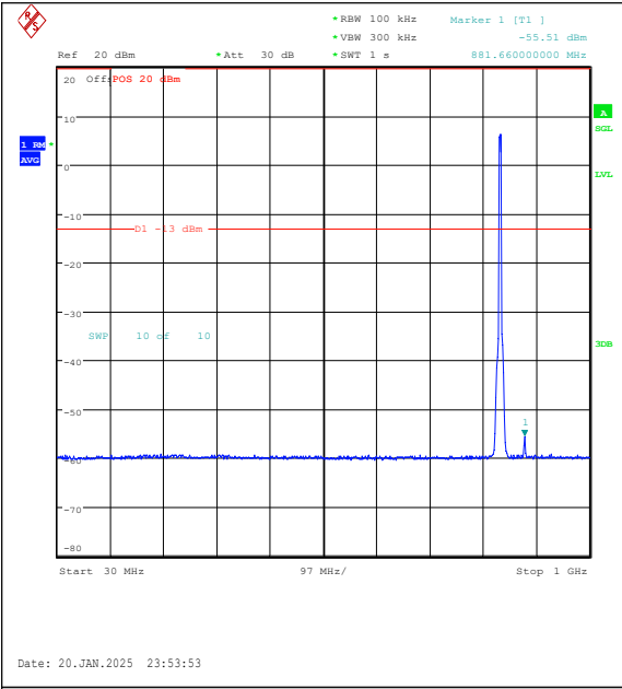
Band5-5MHz-QPSK-20525-25RB#0-30~1000-PA SS
