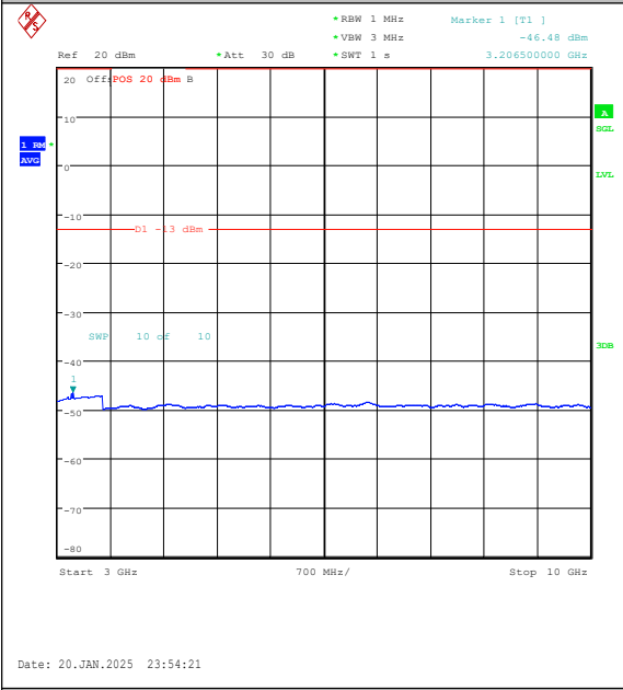
Band5-5MHz-QPSK-20525-25RB#0-3000~10000- PASS
