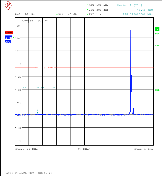
Band5-10MHz-QPSK-20600-1RB#0-30~1000-PA SS
