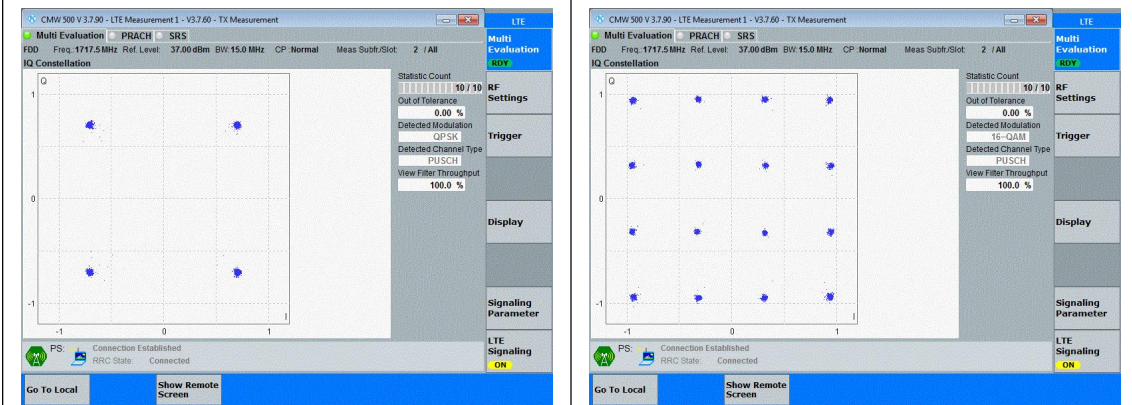
Band4-15MHz-QPSK-20025-75RB#0-PASS
