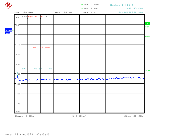
Band4-20MHz-16QAM-20050-1RB#0-3000~20000 -PASS
