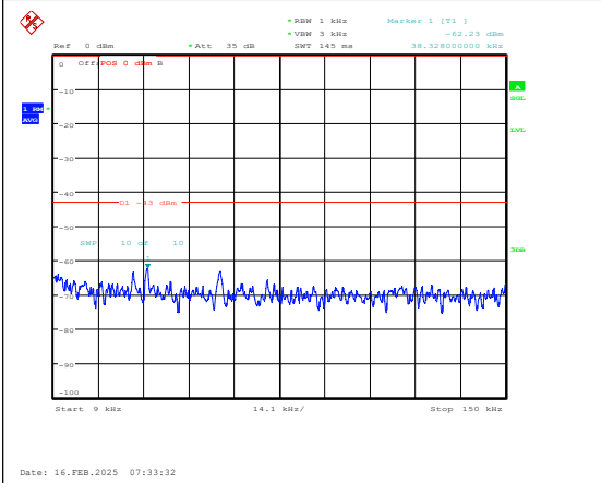
Band4-20MHz-QPSK-20050-1RB#0-0.009~0.15- PASS
