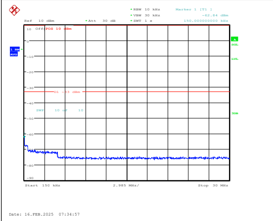
Band4-20MHz-16QAM-20050-1RB#0-0.15~30-PA SS
