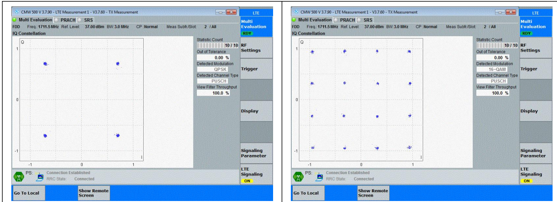
Band4-3MHz-QPSK-19965-15RB#0-PASS
