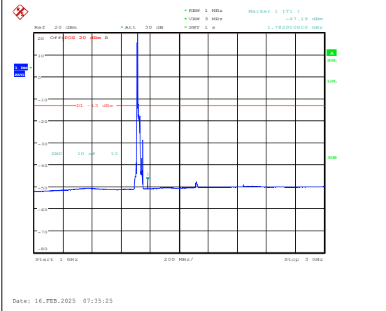
Band4-20MHz-16QAM-20050-1RB#0-1000~3000 -PASS
