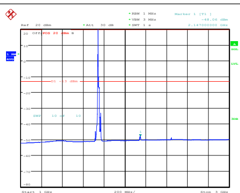
Band4-15MHz-QPSK-20325-1RB#0-1000~3000-P ASS
