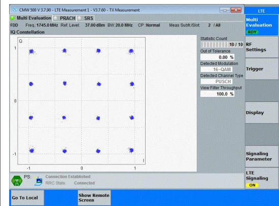
Band4-20MHz-16QAM-20300-100RB#0-PASS
