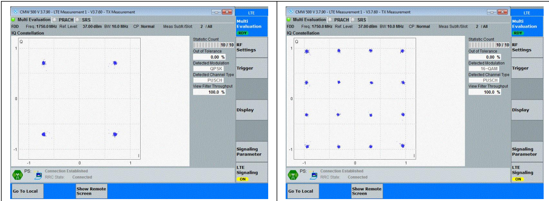
Band4-10MHz-QPSK-20350-50RB#0-PASS
