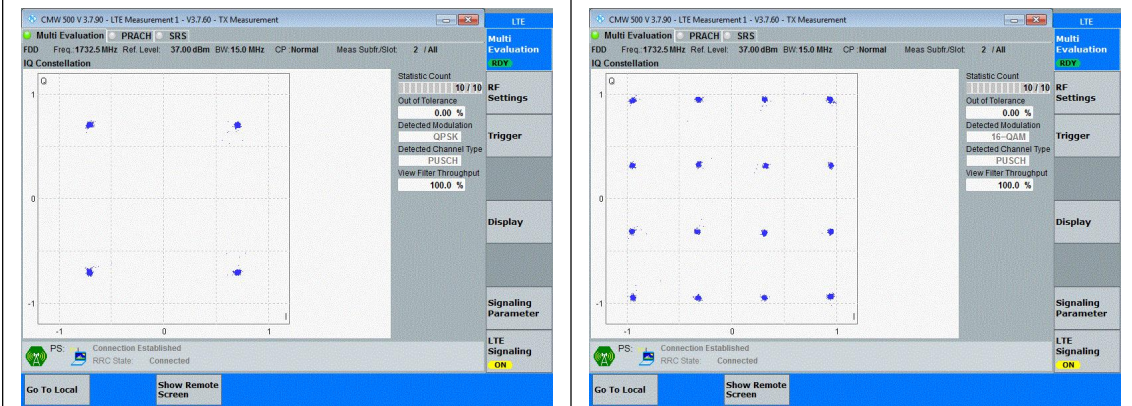
Band4-15MHz-QPSK-20175-75RB#0-PASS
