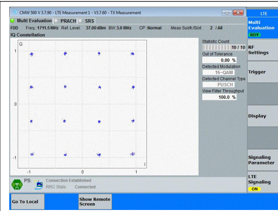
Band4-3MHz-16QAM-19965-15RB#0-PASS
