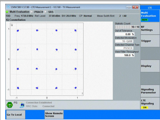
Band4-20MHz-16QAM-20050-100RB#0-PASS
