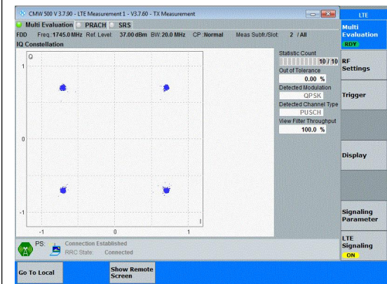
Band4-20MHz-QPSK-20300-100RB#0-PASS
