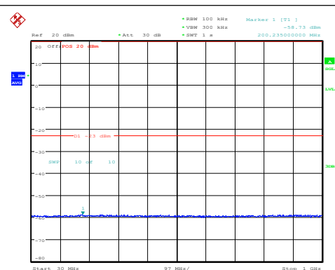
Band4-15MHz-QPSK-20325-1RB#0-30~1000-PA SS
