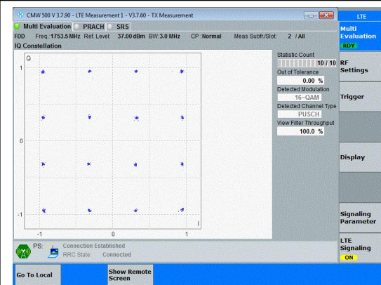
Band4-3MHz-16QAM-20385-15RB#0-PASS
