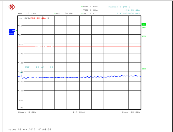
Band4-15MHz-16QAM-20325-1RB#0-3000~20000 -PASS
