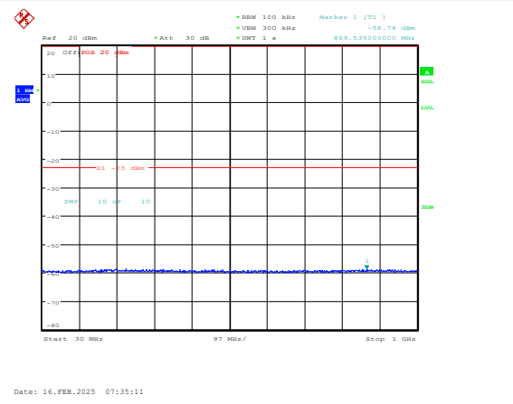
Band4-20MHz-16QAM-20050-1RB#0-30~1000-PA SS
