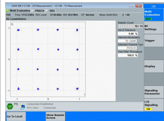
Band4-20MHz-16QAM-20175-100RB#0-PASS
