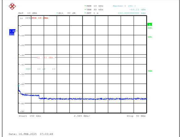
Band4-20MHz-QPSK-20050-1RB#0-0.15~30-PAS S
