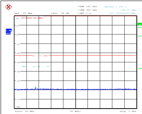
Band4-20MHz-QPSK-20300-1RB#0-30~1000-PA SS
