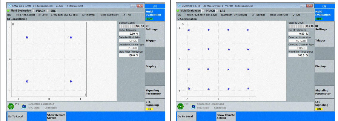
Band4-5MHz-QPSK-20375-25RB#0-PASS
