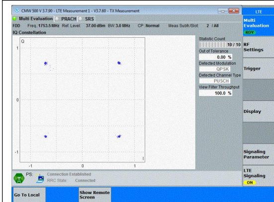
Band4-3MHz-QPSK-20385-15RB#0-PASS
