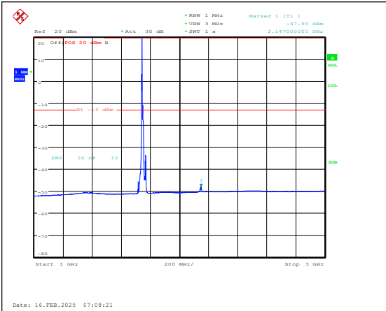
Band4-15MHz-16QAM-20325-1RB#0-1000~3000 -PASS
