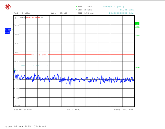
Band4-20MHz-16QAM-20050-1RB#0-0.009~0.15- PASS
