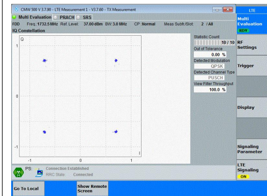
Band4-3MHz-QPSK-20175-15RB#0-PASS
