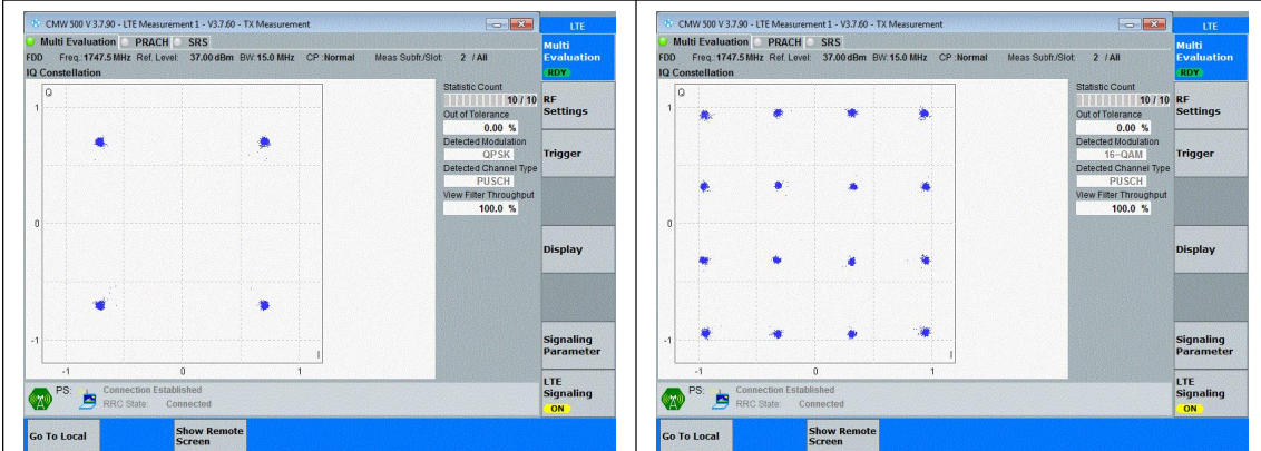
Band4-15MHz-QPSK-20325-75RB#0-PASS
