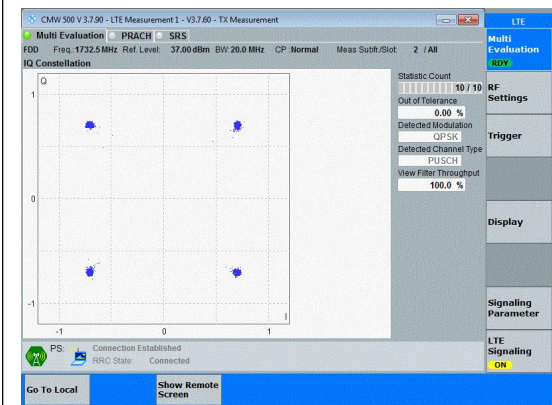
Band4-20MHz-QPSK-20175-100RB#0-PASS
