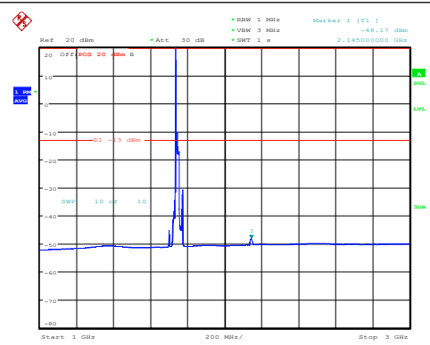
Band4-20MHz-QPSK-20300-1RB#0-1000~3000-P ASS
