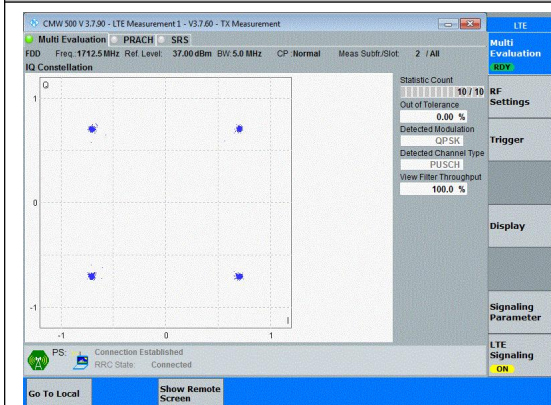
Band4-5MHz-QPSK-19975-25RB#0-PASS
