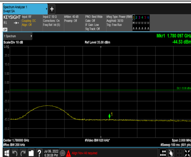
Band66-10MHz-QPSK-132622-1RB#0
