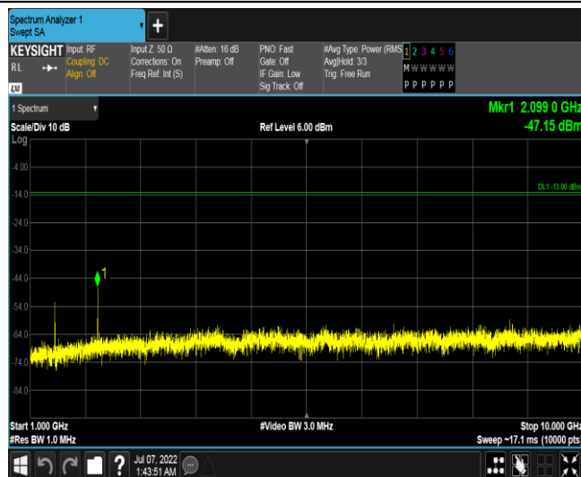
Band12-3MHz-16QAM-23025-1RB#0-Range3:1000~10000MHz
