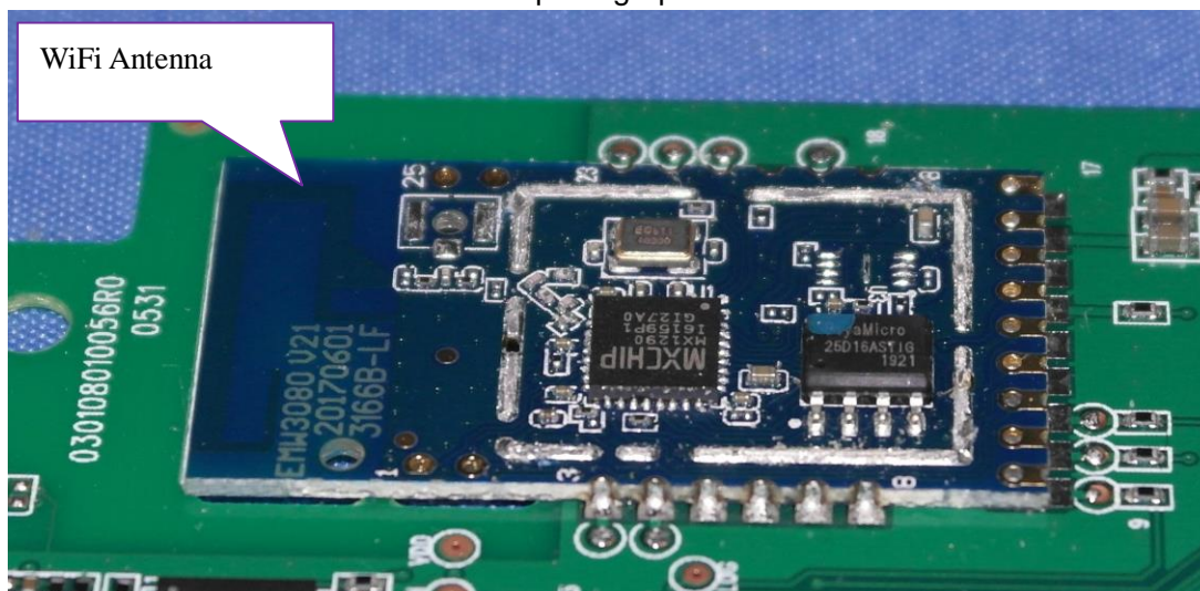
Internal photograph of EUT
