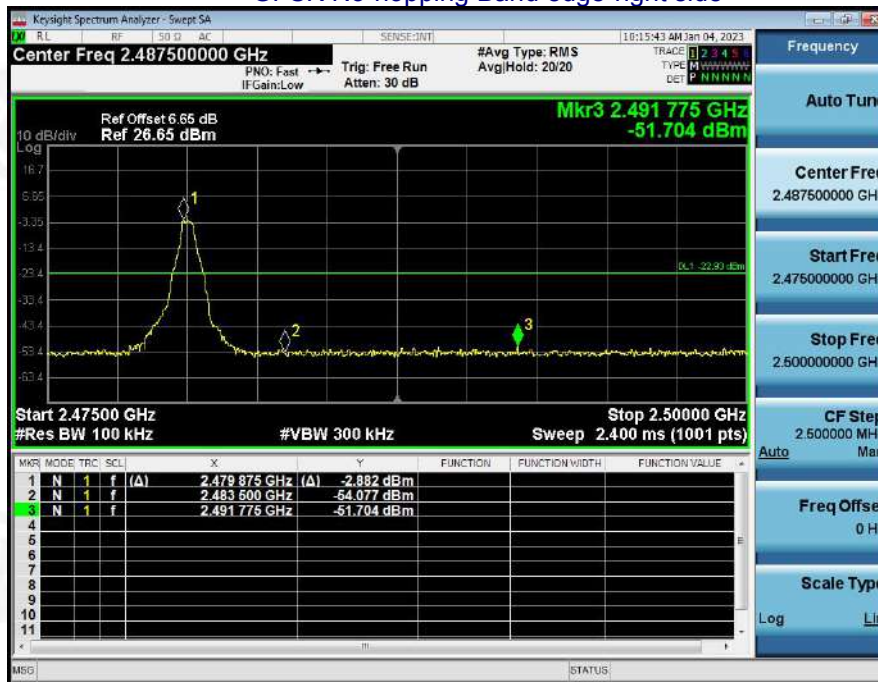
GFSK No-hopping Band edge-right side
