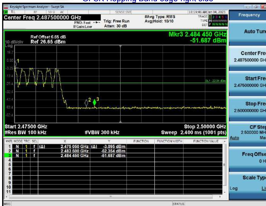
GFSK Hopping Band edge-right side
