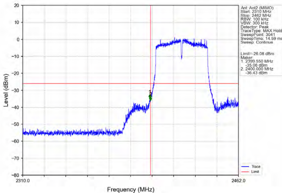
802.11ac(VHT40)_LCH_2422MHz_Ant2 (MIMO)_NTNV
