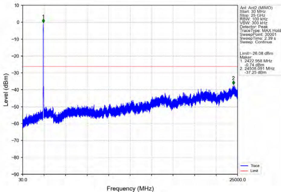
802.11ac(VHT40)_LCH_2422MHz_Ant2 (MIMO)_NTNV
