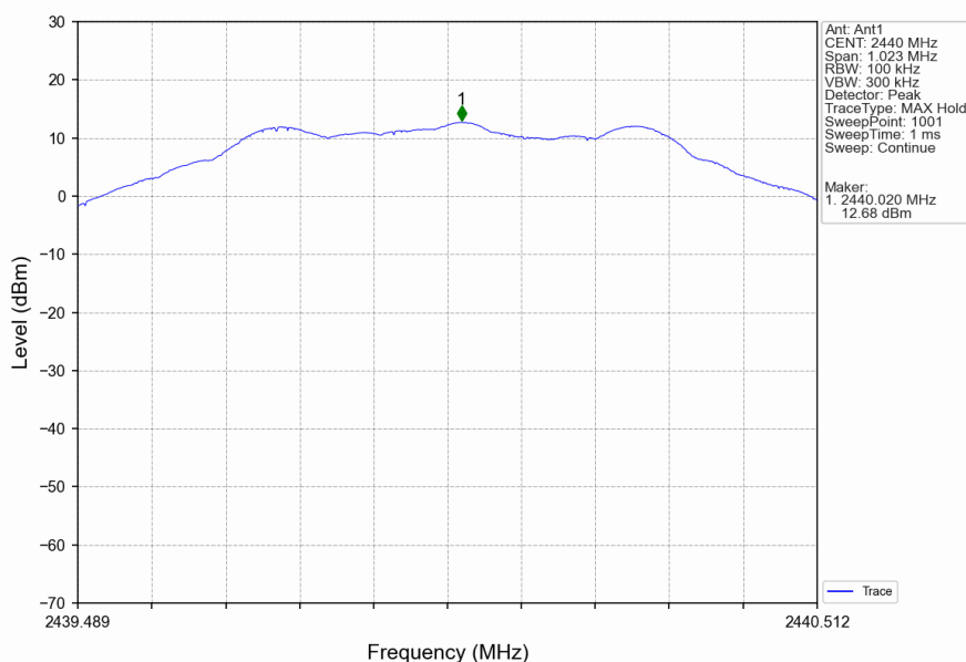
1M_MCH_2440MHz_Ant1_NTNV
