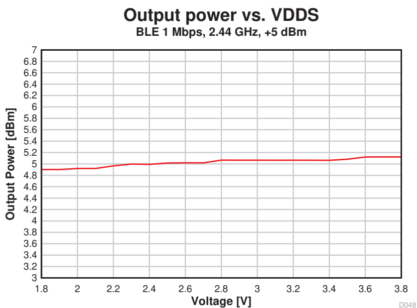
Figure 5-17. Output Power vs. Supply Voltage (VDD) (BLE 1 Mbps, 2.44 GHz, +5 dBm)
