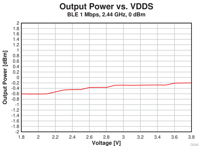
Figure 5-16. Output Power vs. Supply Voltage (VDD) (BLE 1 Mbps, 2.44 GHz)
