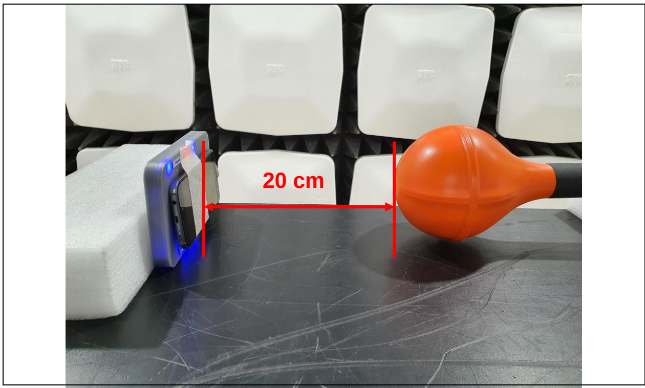
H-field Measurements _ Distance : 20 cm
