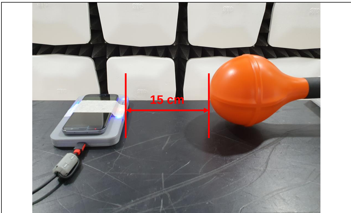
H-field Measurements _ Distance : 15 cm
