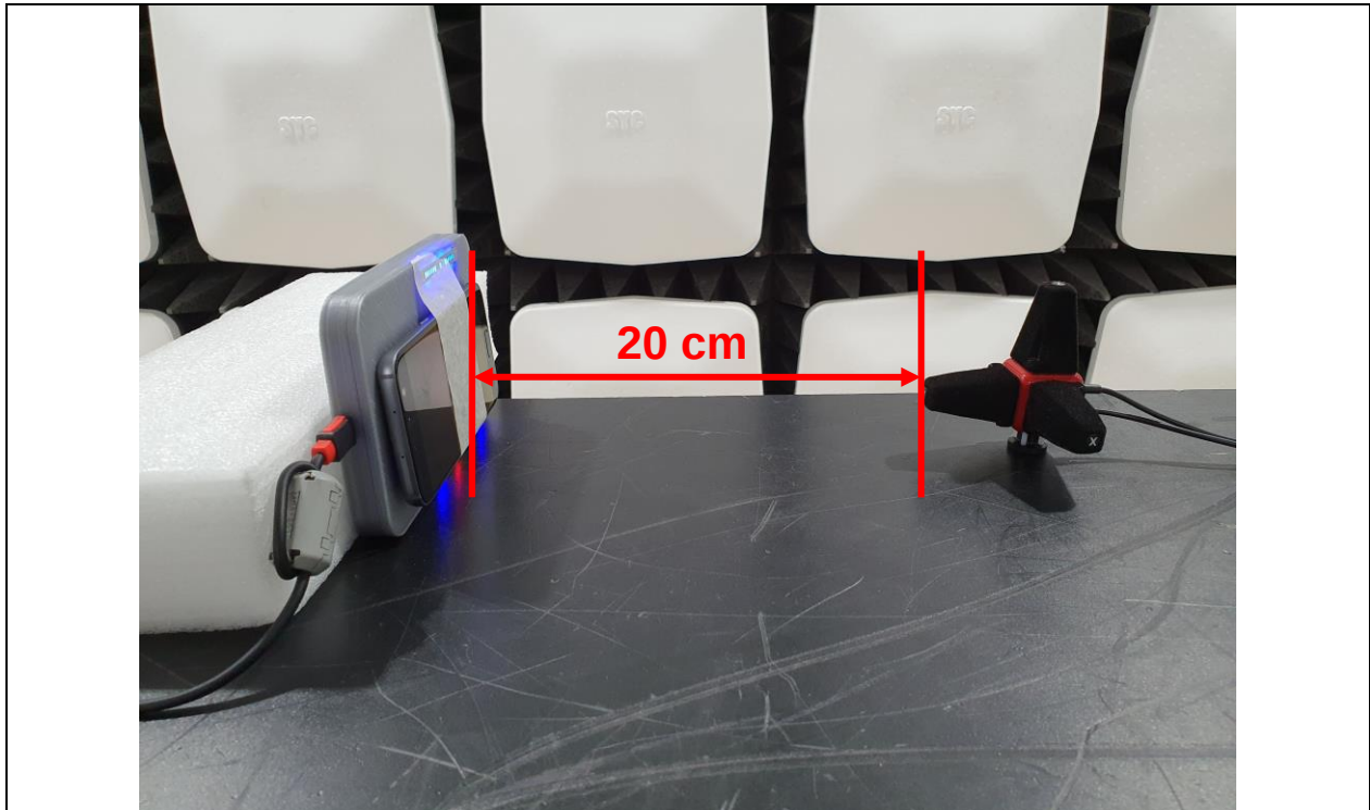
E-field Measurements _ Distance : 20 cm
