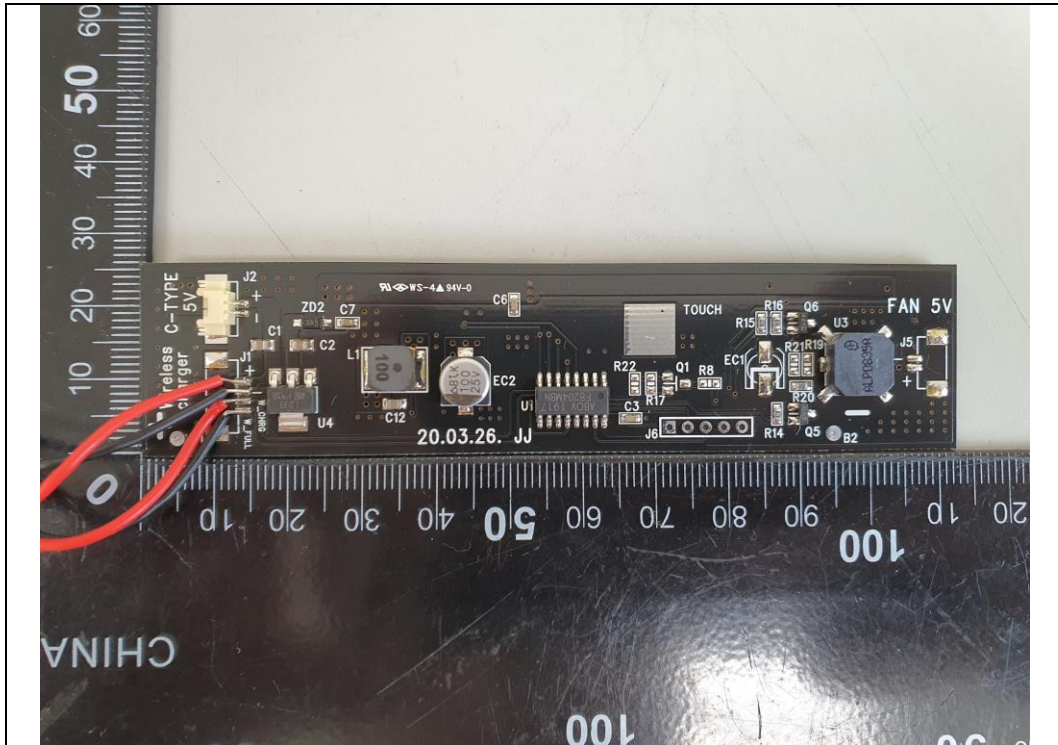
Sub Board#1_Front
