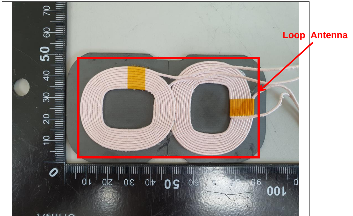
Coil
