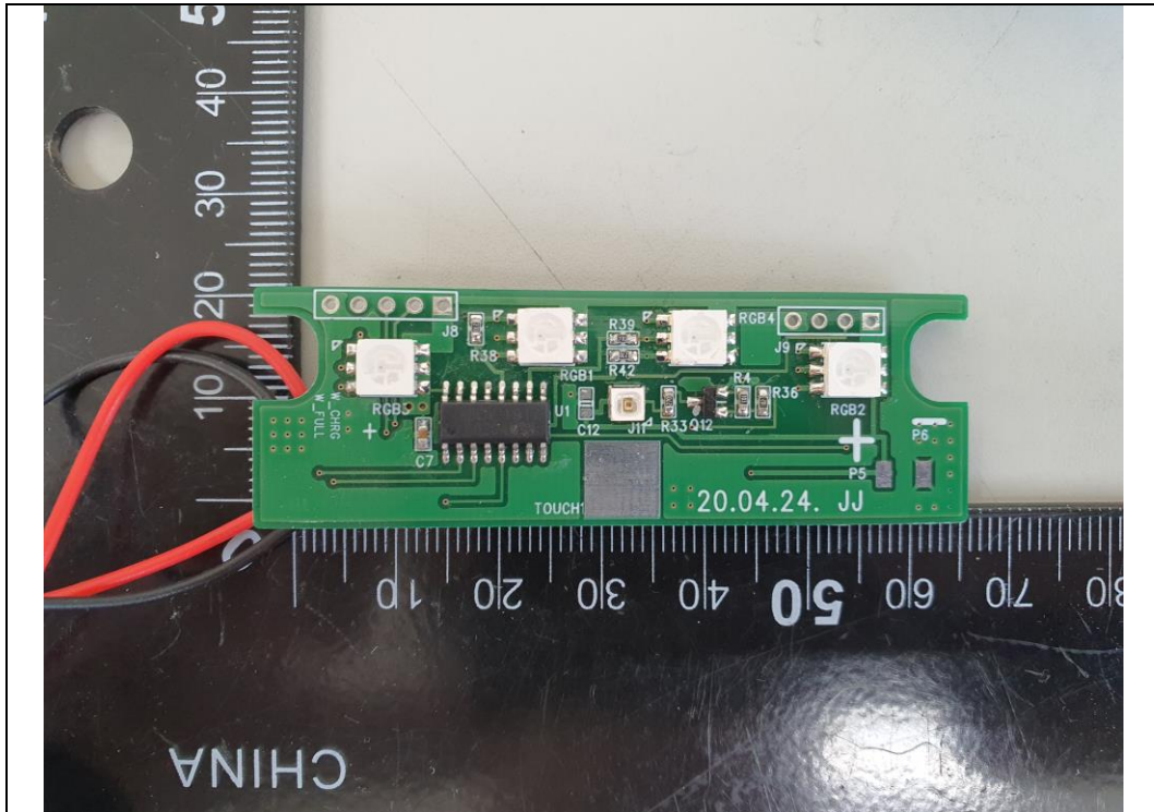
Sub Board#2 Front
