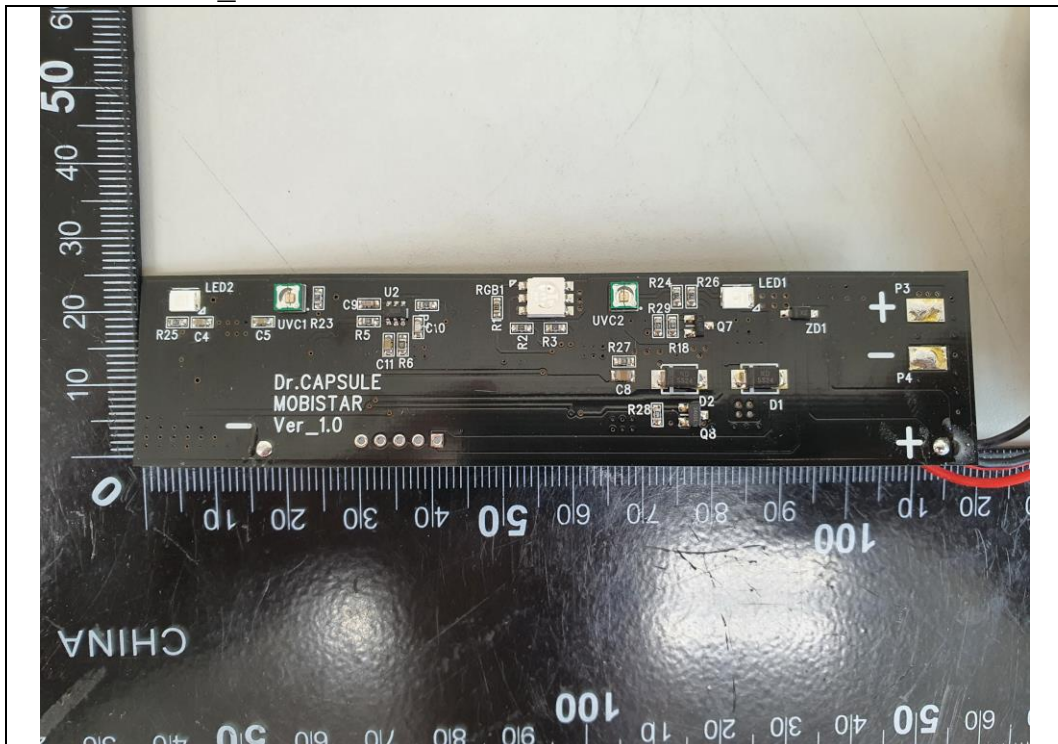
Sub Board#1_Rear
