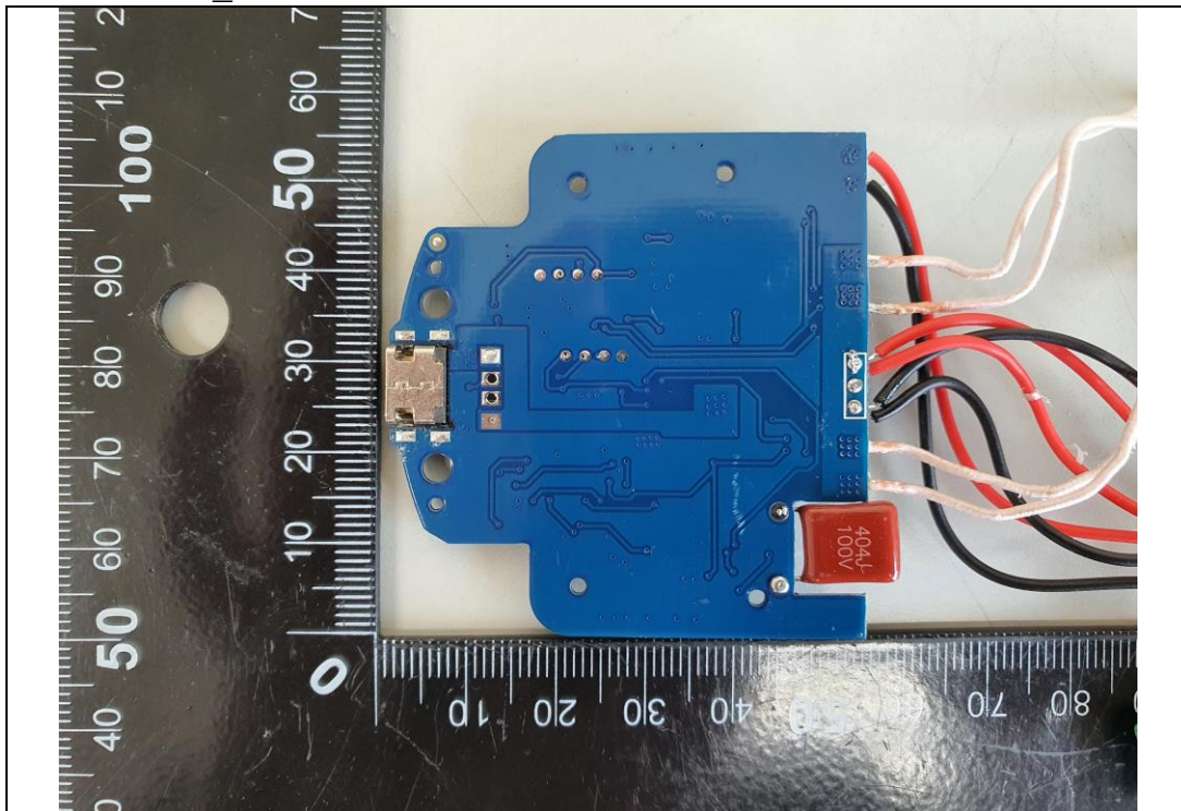
Main Board_Rear
