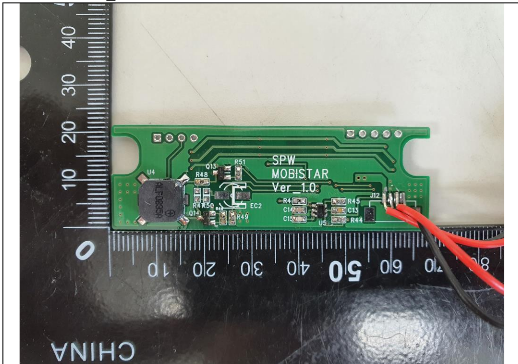
Sub Board#2 Rear
