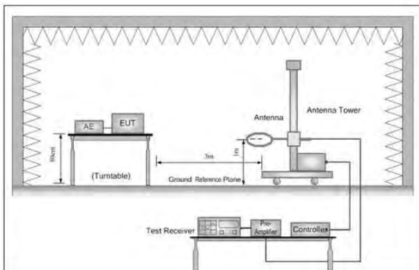
Below 30MHz
