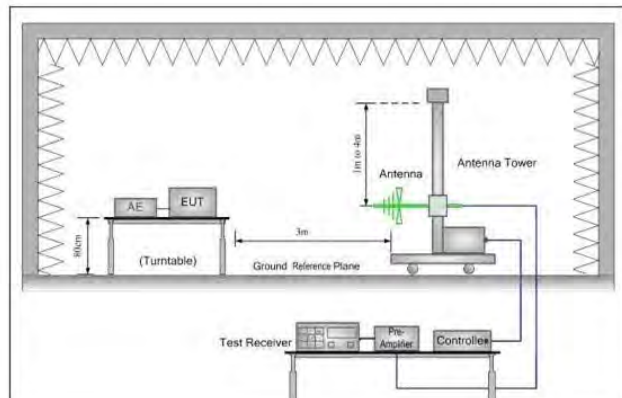
30MHz-1GHz
