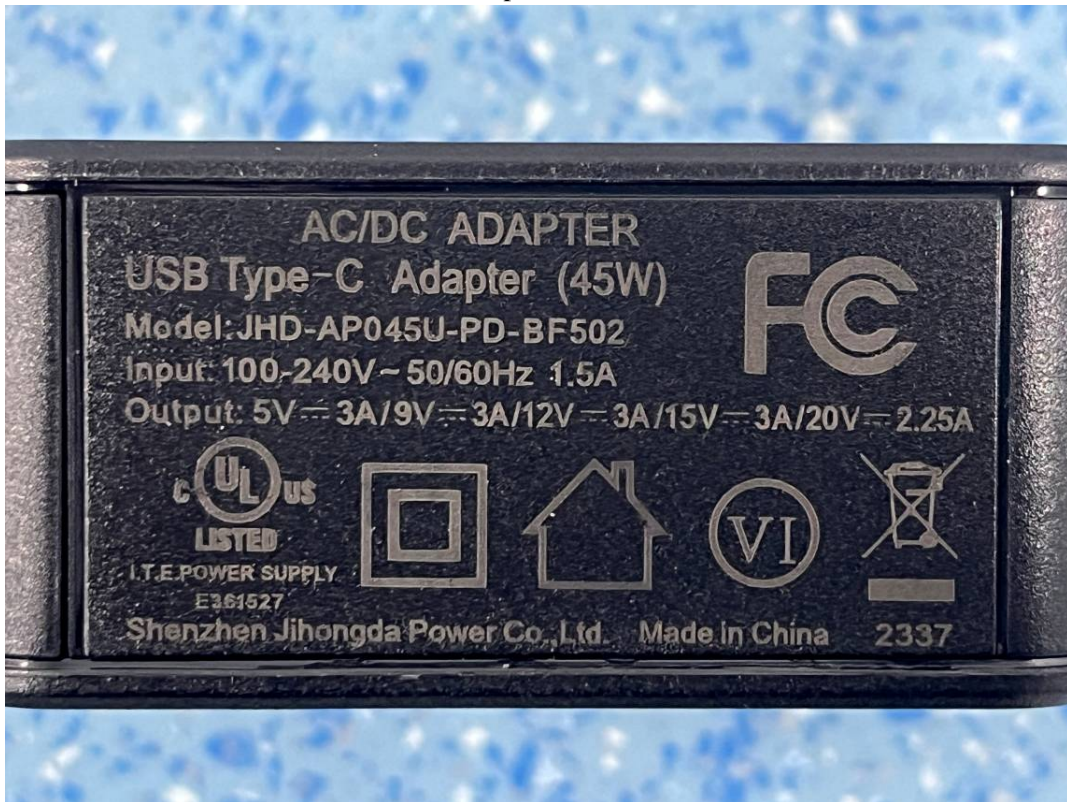
Adapter Label
