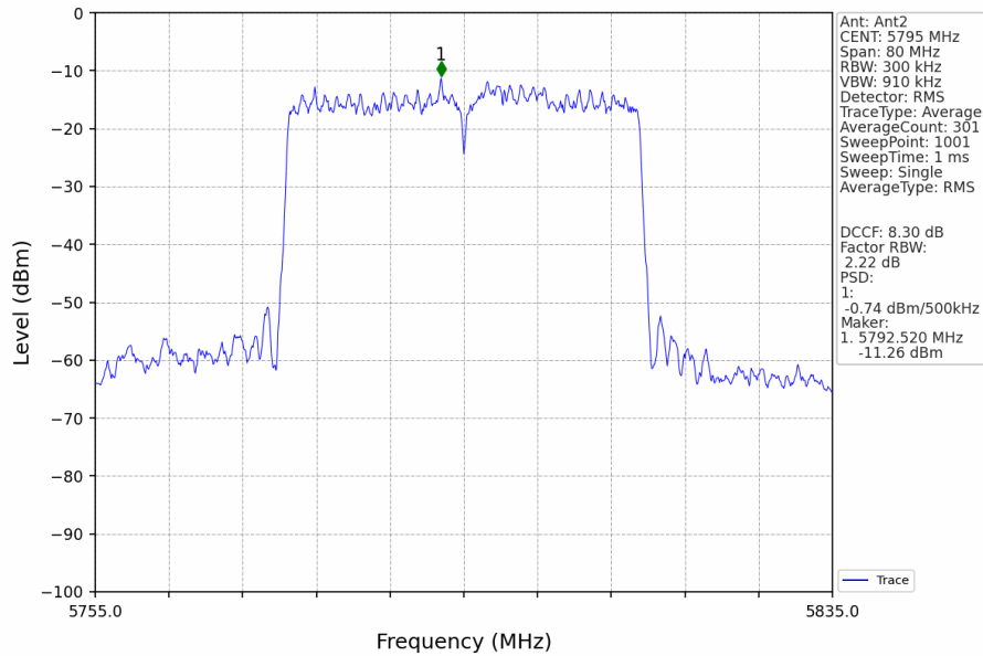
802.11ax(HEW40)_HCH_5795MHz_RU484_Left_MIMO_NTNV
