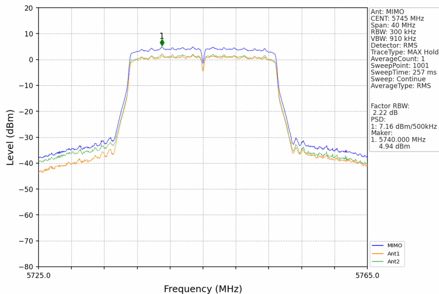
802.11ac(VHT20)_LCH_5745MHz_MIMO_NTNV
