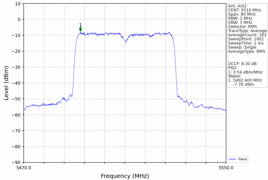
802.11ax(HEW40)_LCH_5510MHz_RU484_Left_MIMO_NTNV
