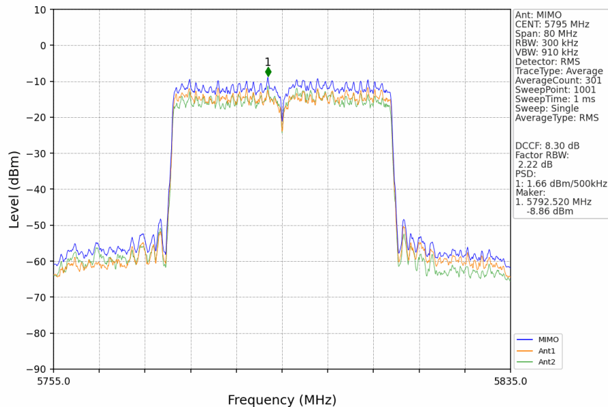
802.11ax(HEW40)_HCH_5795MHz_RU484_Left_MIMO_NTNV
