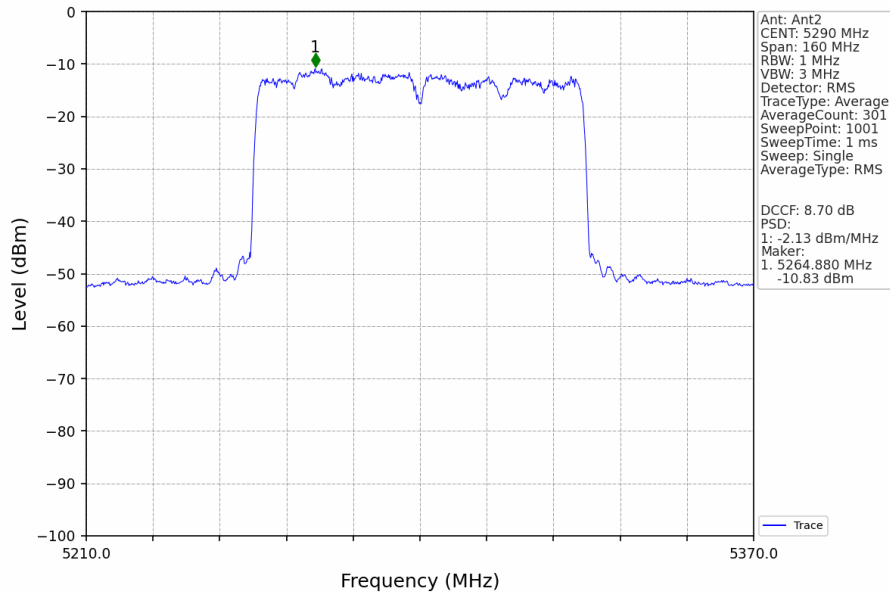
802.11ax(HEW80)_MCH_5290MHz_RU996_Left_MIMO_NTNV
