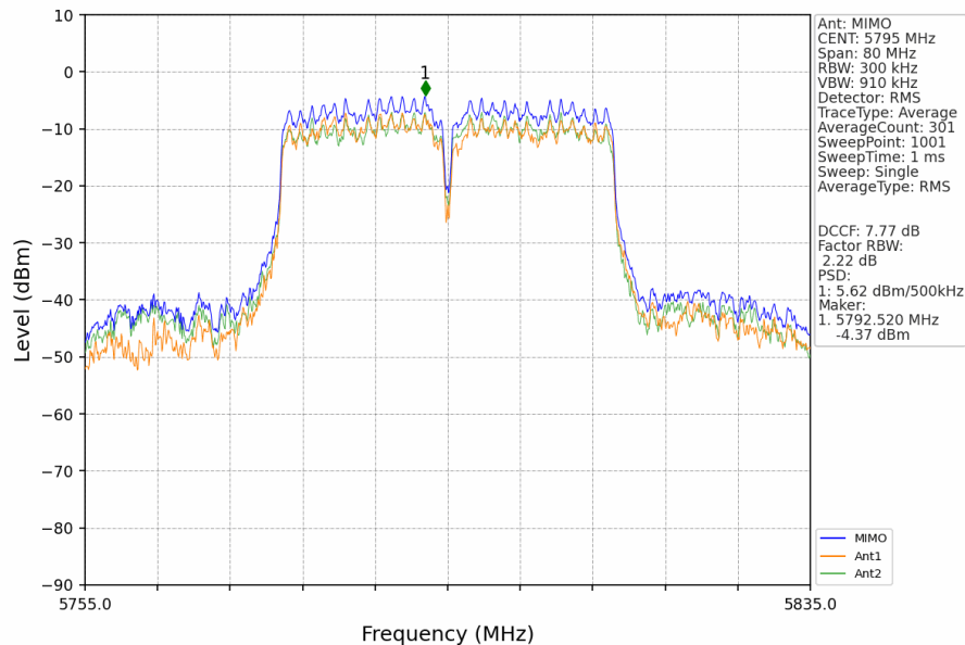
802.11ac(VHT40)_HCH_5795MHz_MIMO_NTNV
