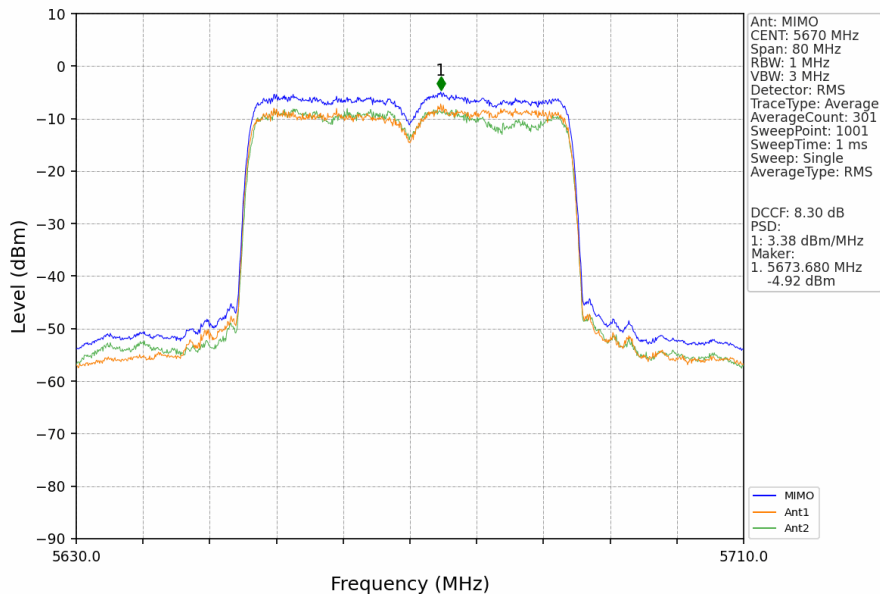
802.11ax(HEW40)_HCH_5670MHz_RU484_Left_MIMO_NTNV
