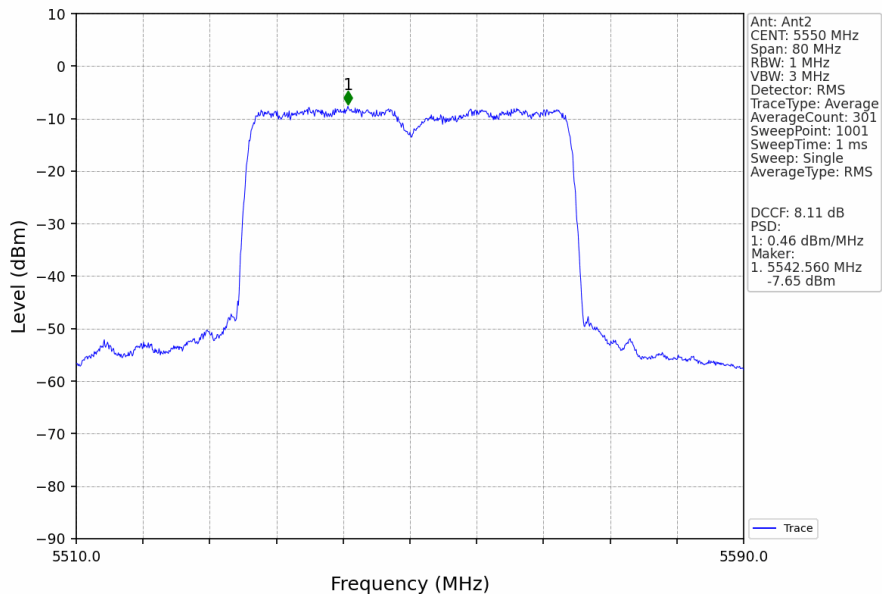
802.11ax(HEW40)_MCH_5550MHz_RU484_Left_Ant2_NTNV
