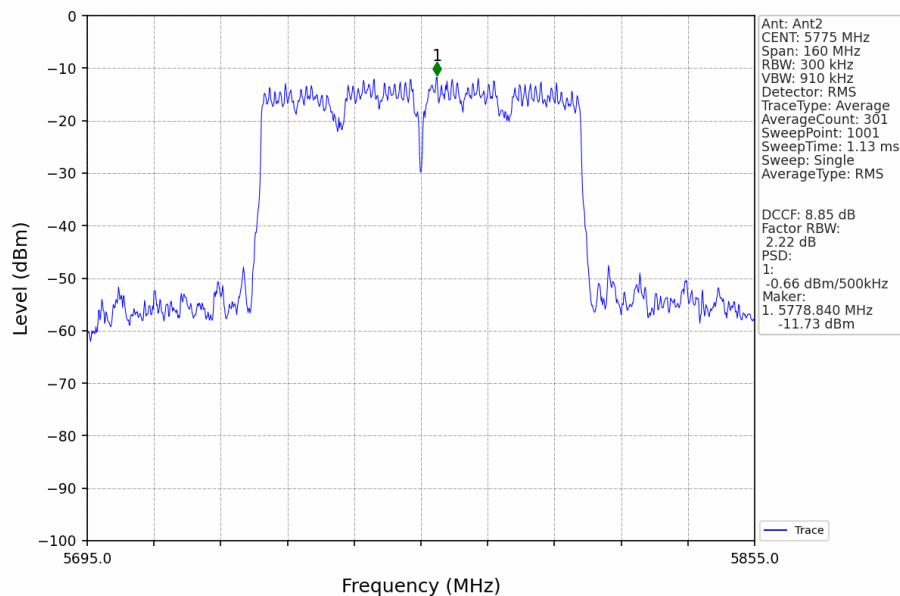
802.11ac(VHT80)_MCH_5775MHz_Ant2_NTNV
