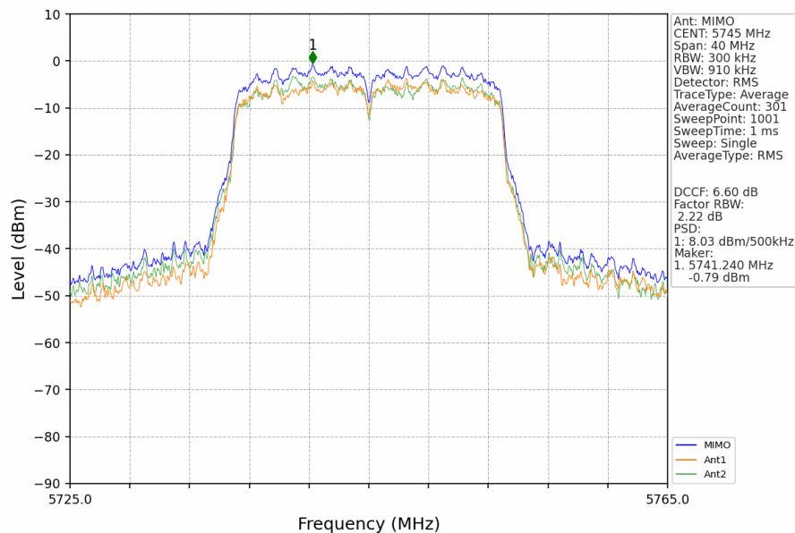
802.11ax(HEW20)_LCH_5745MHz_RU242_Left_MIMO_NTNV
