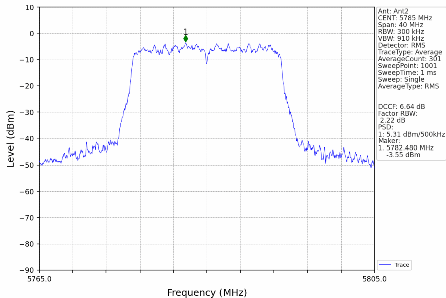
802.11ax(HEW20)_MCH_5785MHz_RU242_Left_Ant2_NTNV
