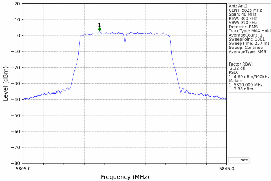
802.11ac(VHT20)_HCH_5825MHz_MIMO_NTNV
