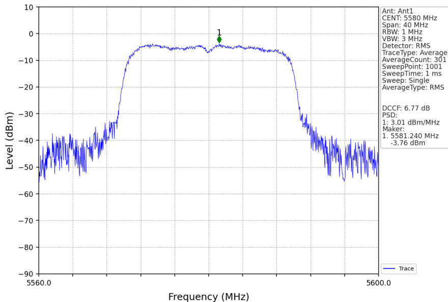
802.11ax(HEW20)_MCH_5580MHz_RU242_Left_Ant1_NTNV
