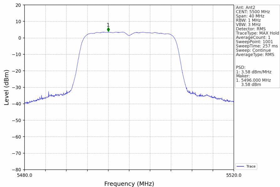
802.11ac(VHT20)_LCH_5500MHz_Ant2_NTNV
