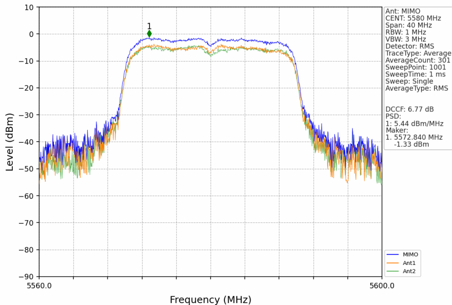
802.11ax(HEW20)_MCH_5580MHz_RU242_Left_MIMO_NTNV
