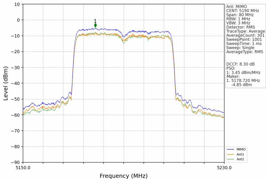
802.11ax(HEW40)_LCH_5190MHz_RU484_Left_MIMO_NTNV
