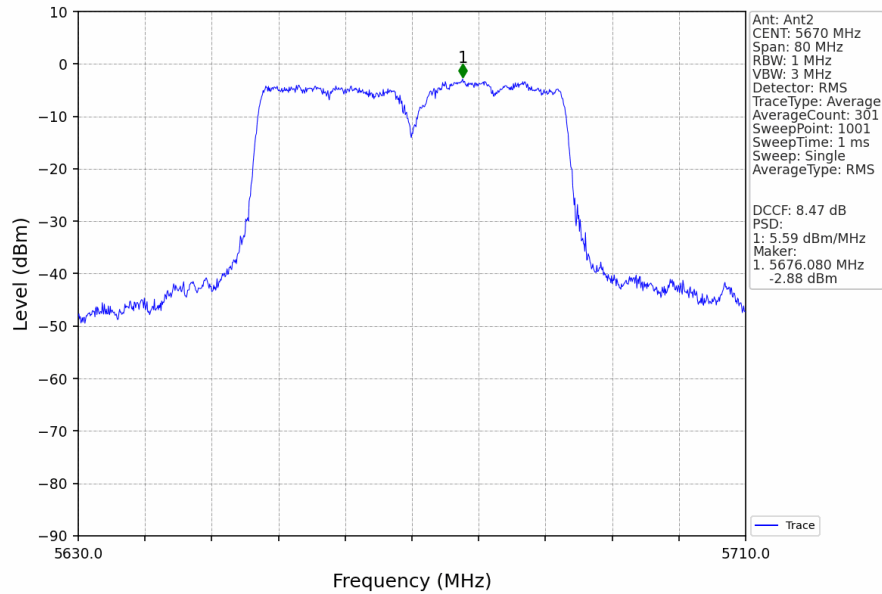
802.11ac(VHT40)_HCH_5670MHz_MIMO_NTNV
