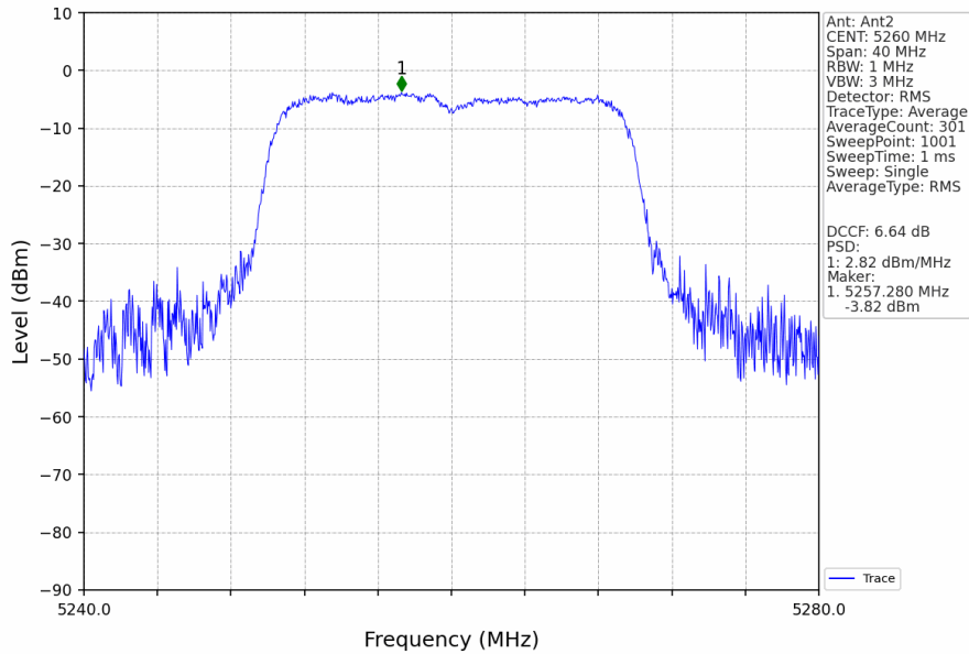
802.11ax(HEW20)_LCH_5260MHz_RU242_Left_MIMO_NTNV
