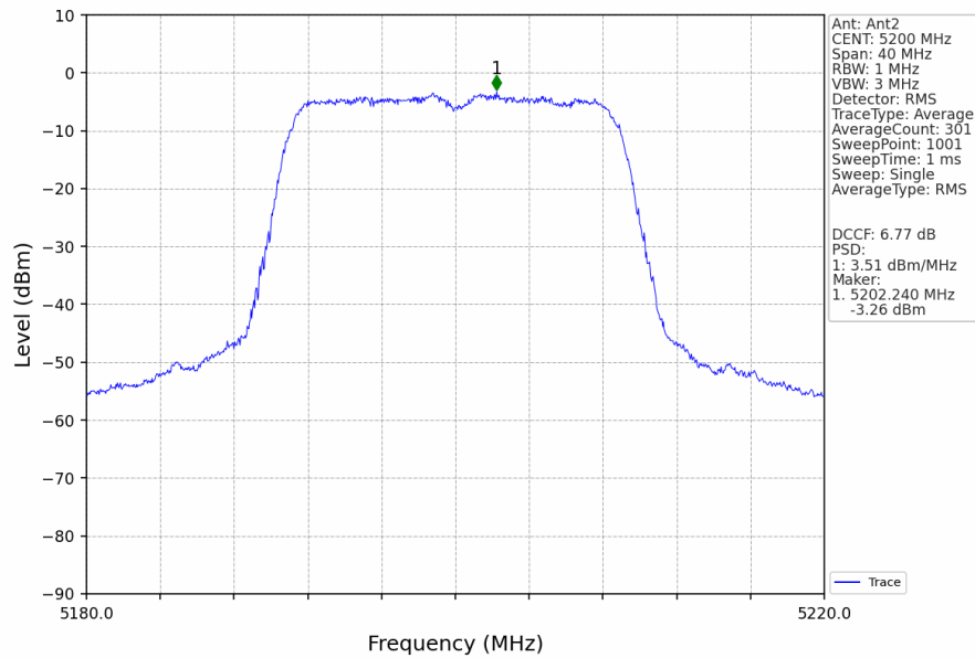
802.11ax(HEW20)_MCH_5200MHz_RU242_Left_MIMO_NTNV
