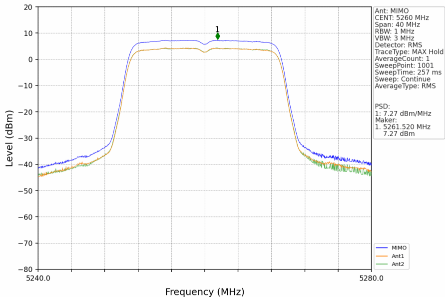
802.11ac(VHT20)_LCH_5260MHz_MIMO_NTNV
