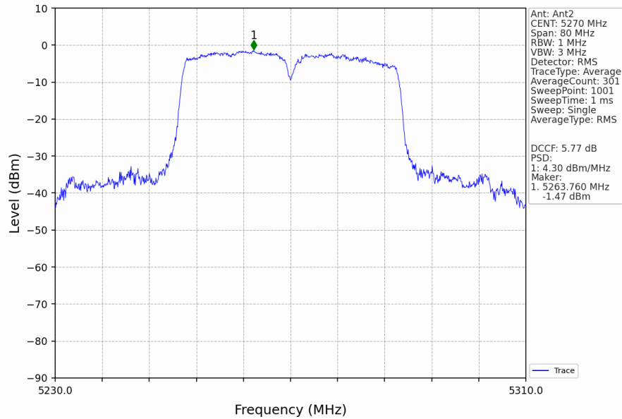
802.11ac(VHT40)_LCH_5270MHz_MIMO_NTNV
