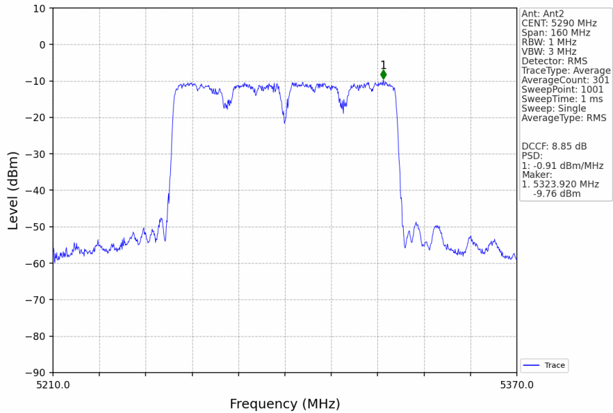
802.11ac(VHT80)_MCH_5290MHz_MIMO_NTNV
