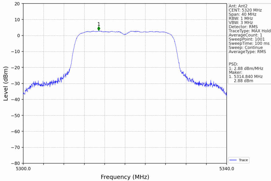
802.11ax(HEW20)_HCH_5320MHz_RU242_Left_MIMO_NTNV
