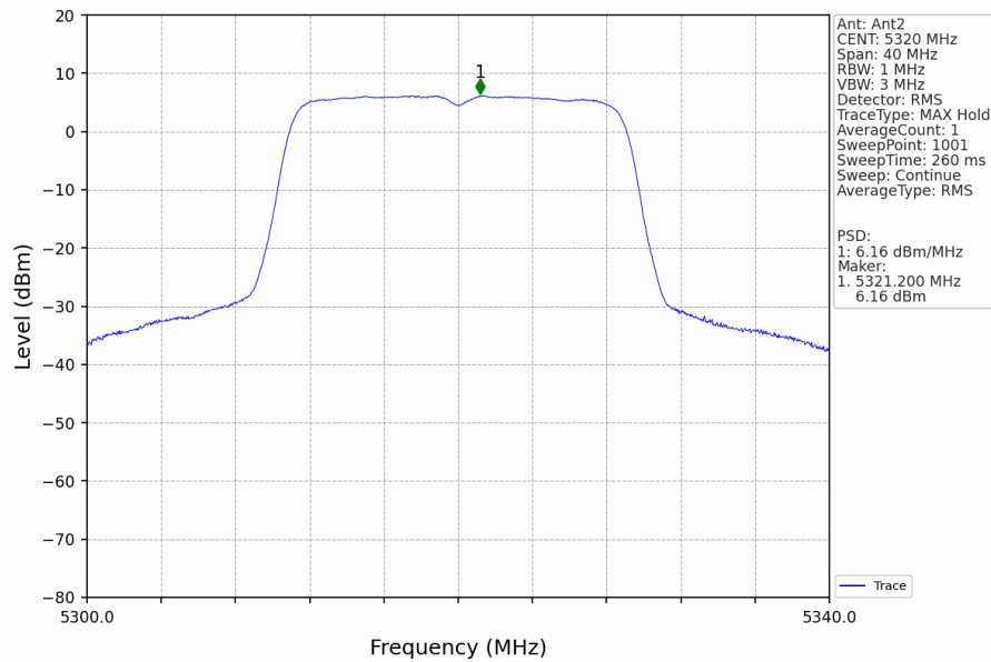
802.11ac(VHT20)_HCH_5320MHz_MIMO_NTNV
