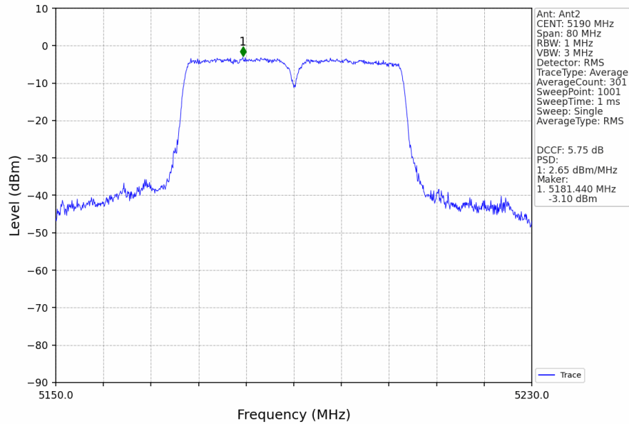
802.11ac(VHT40)_LCH_5190MHz_MIMO_NTNV
