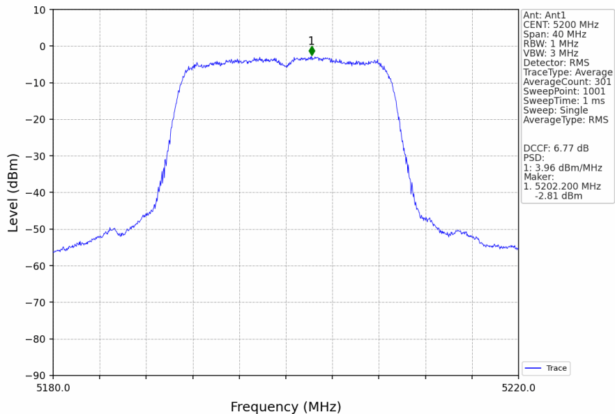
802.11ax(HEW20)_MCH_5200MHz_RU242_Left_Ant1_NTNV
