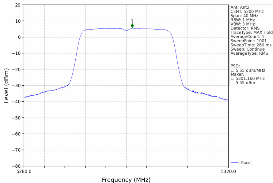
802.11ac(VHT20)_MCH_5300MHz_Ant2_NTNV
