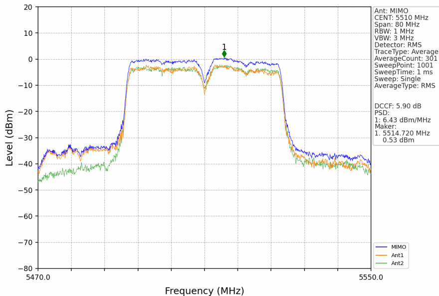
802.11ac(VHT40)_LCH_5510MHz_MIMO_NTNV
