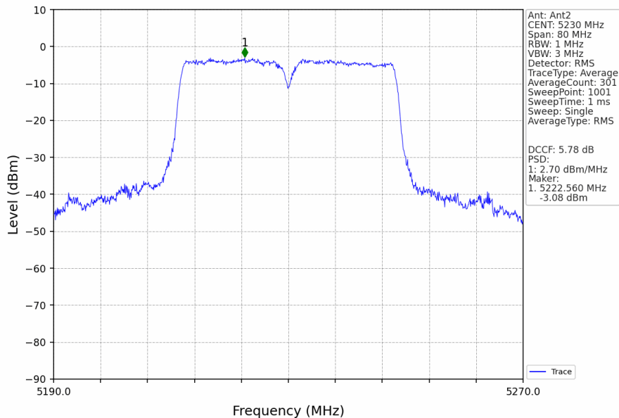
802.11ac(VHT40)_HCH_5230MHz_Ant2_NTNV
