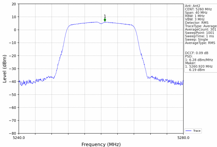
802.11a_LCH_5260MHz_Ant2_NTNV
