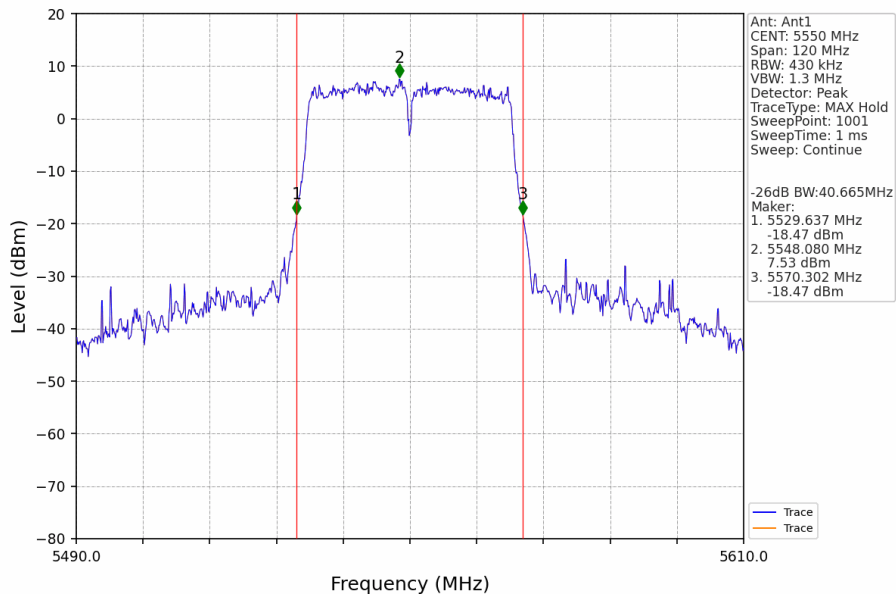
802.11ax(HEW40)_MCH_5550MHz_RU484_Left_Ant1_NTNV
