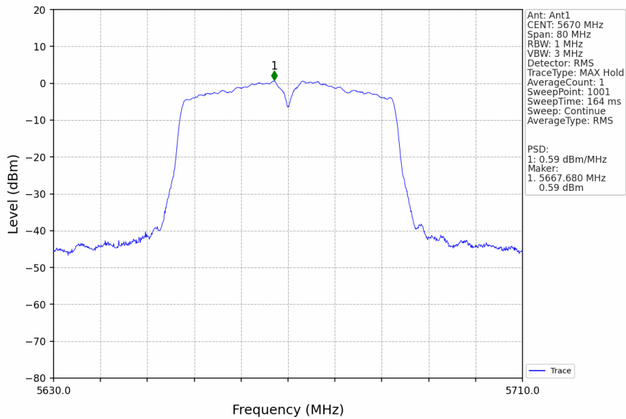
802.11n(HT40)_HCH_5670MHz_Ant1_NTNV
