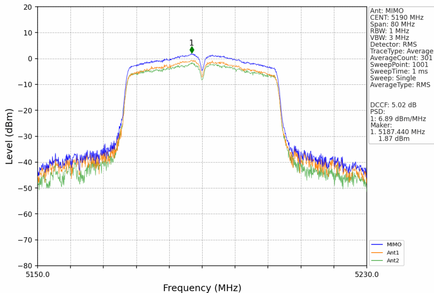
802.11n(HT40)_LCH_5190MHz_MIMO_NTNV
