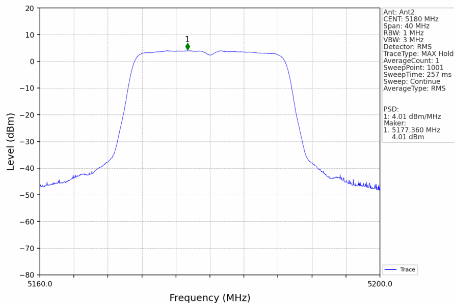
802.11ac(VHT20)_LCH_5180MHz_Ant2_NTNV
