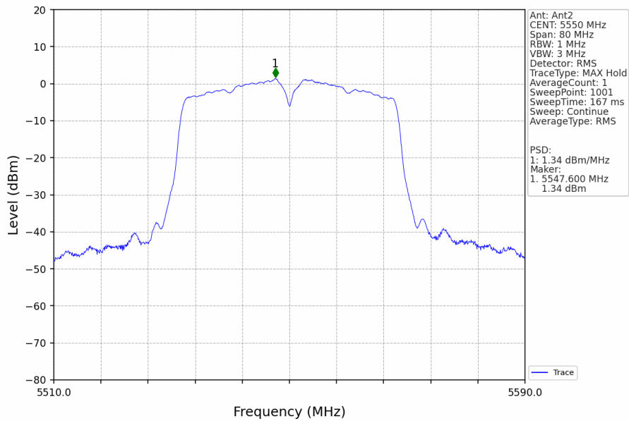
802.11n(HT40)_MCH_5550MHz_Ant2_NTNV
