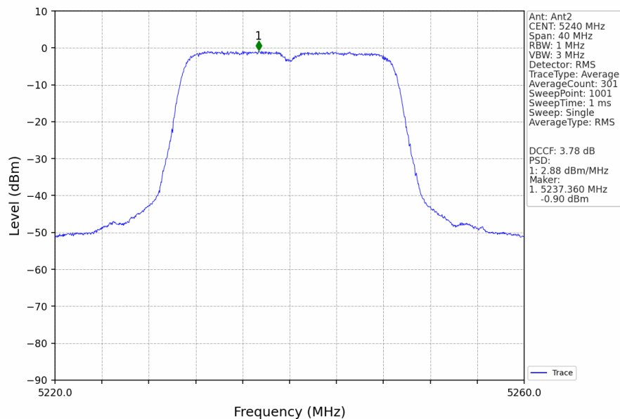
802.11ac(VHT20)_HCH_5240MHz_Ant2_NTNV
