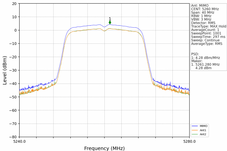
802.11n(HT20)_LCH_5260MHz_MIMO_NTNV
