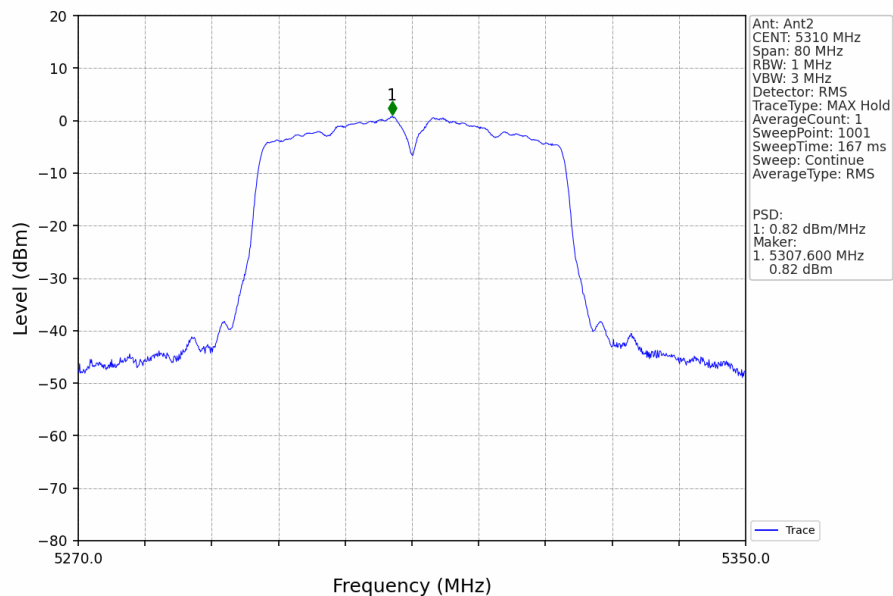
802.11n(HT40)_HCH_5310MHz_Ant2_NTNV
