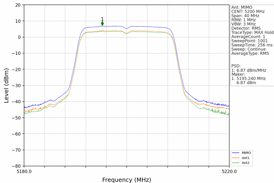
802.11ac(VHT20)_MCH_5200MHz_MIMO_NTNV
