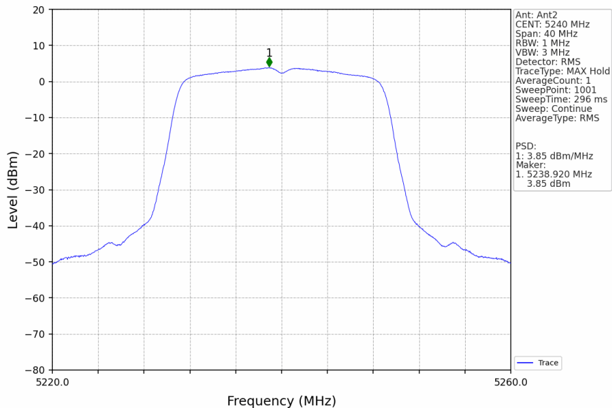
802.11n(HT20)_HCH_5240MHz_Ant2_NTNV
