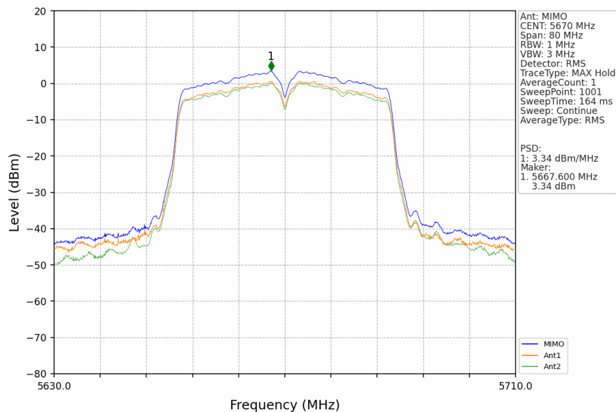
802.11n(HT40)_HCH_5670MHz_MIMO_NTNV
