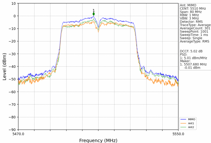
802.11n(HT40)_LCH_5510MHz_MIMO_NTNV
