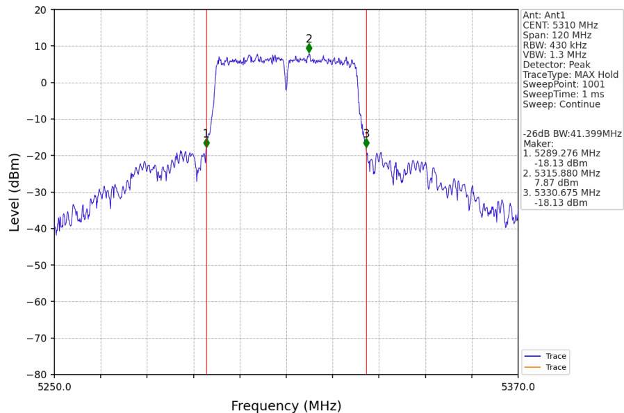
802.11ac(VHT40)_HCH_5310MHz_Ant1_NTNV
