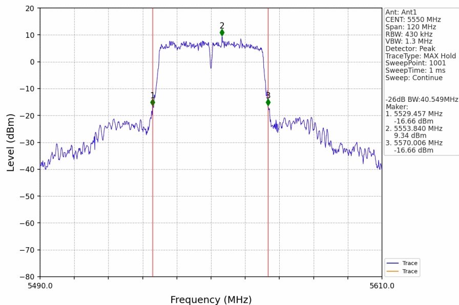
802.11ac(VHT40)_MCH_5550MHz_Ant1_NTNV
