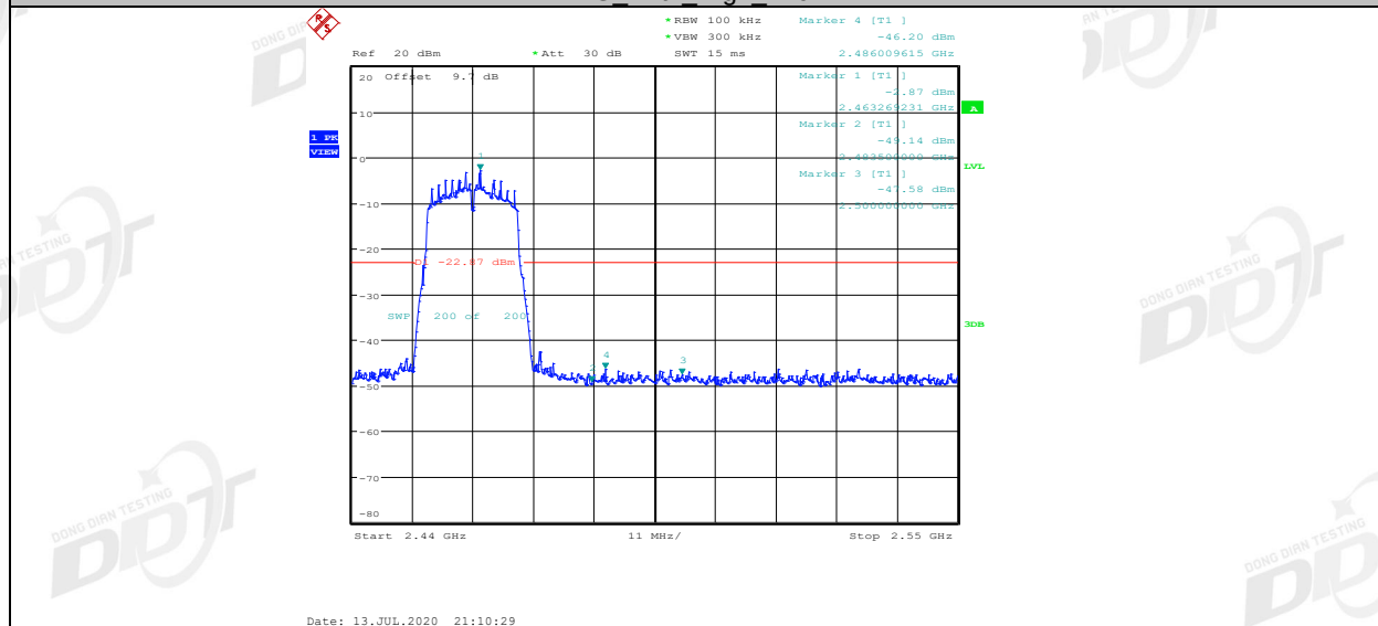
11G_Ant2_High_2462
