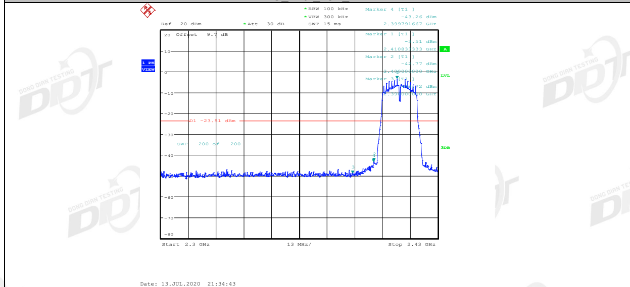
11G_Ant1_High_2462
