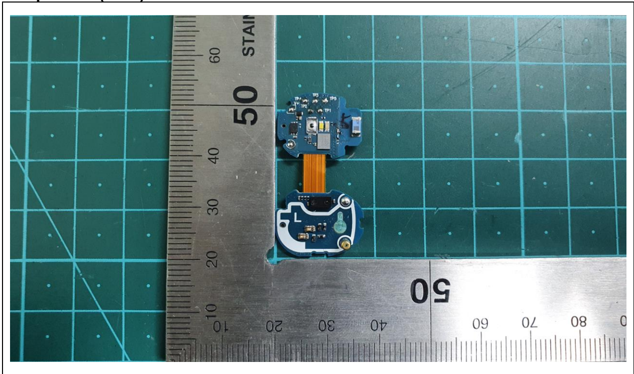
Earphone L(Rear)
