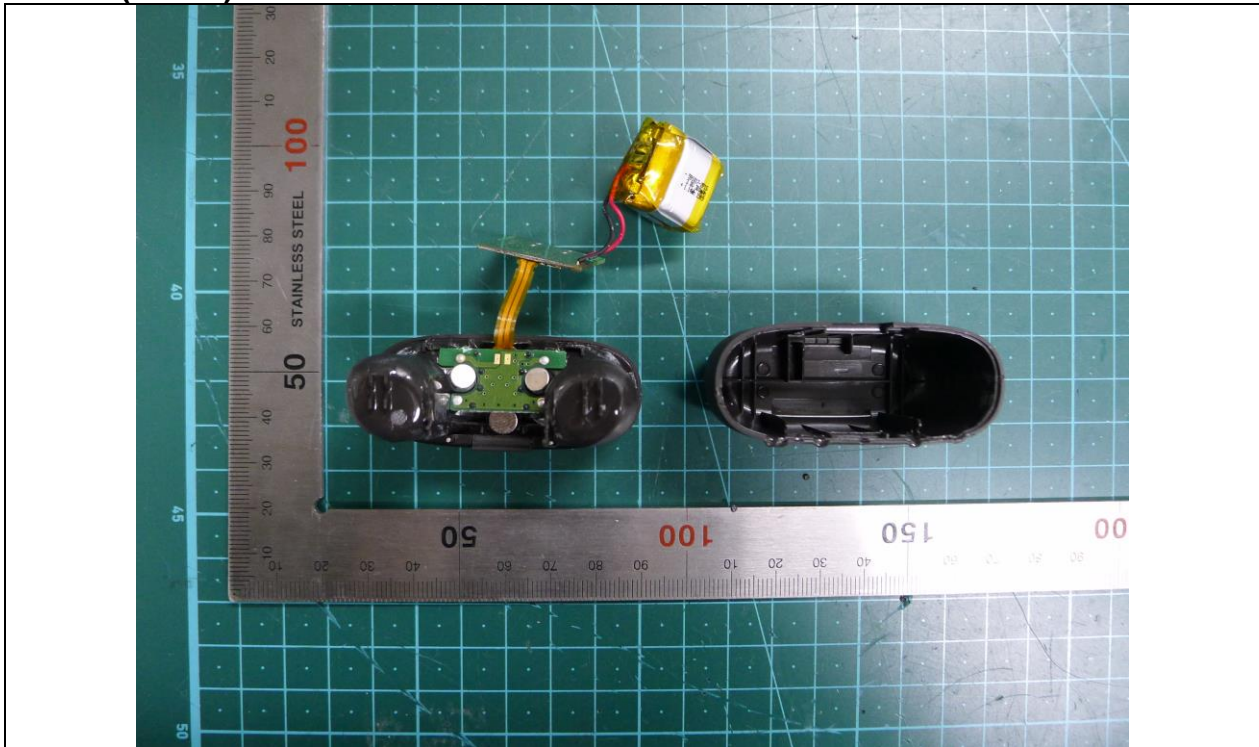
Cradle(Inside)
