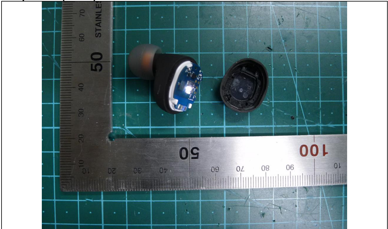
Earphone R(Inside)
