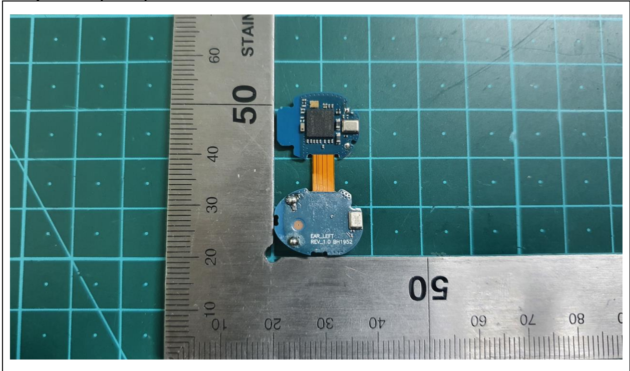
Earphone L(Front)
