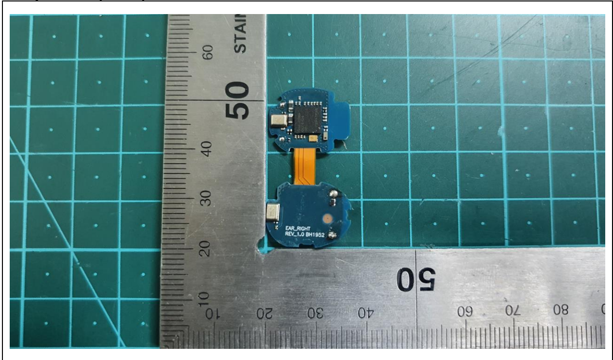
Earphone R(Front)
