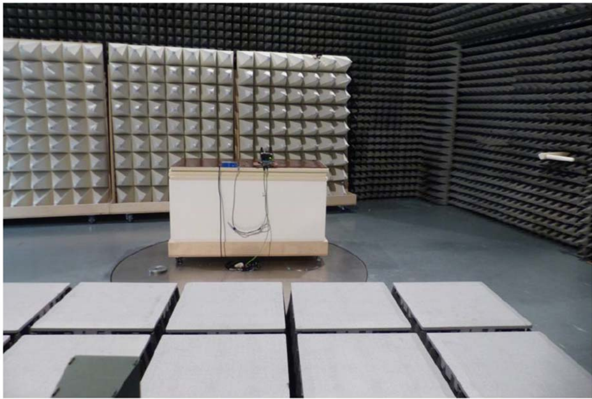
Test setup 26.5-30GHz
