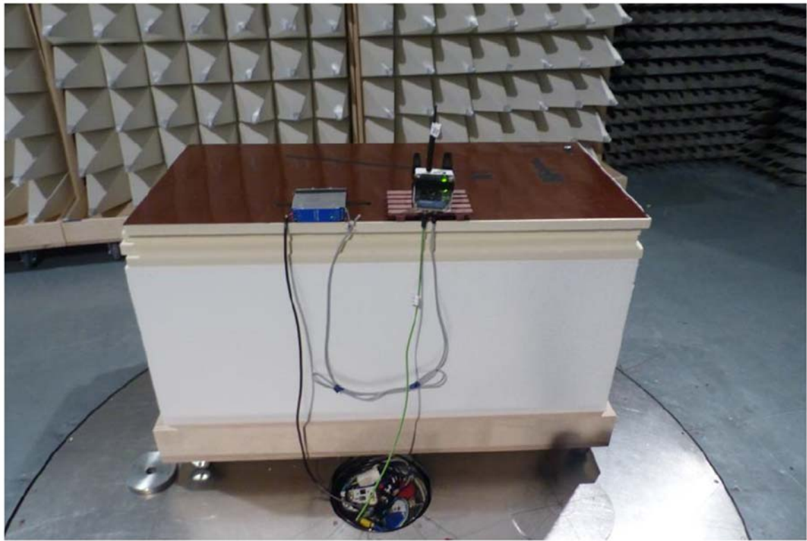
Test setup
