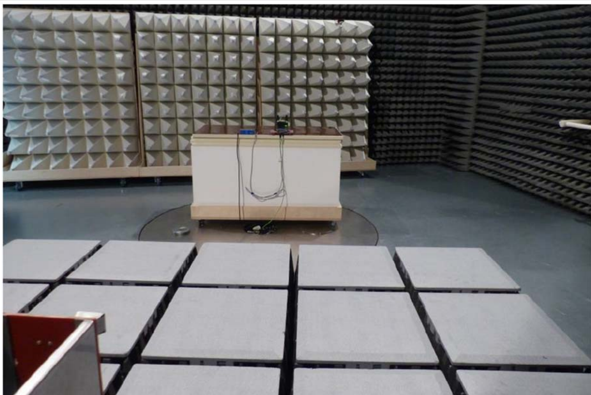
Test setup 17-26.5GHz
