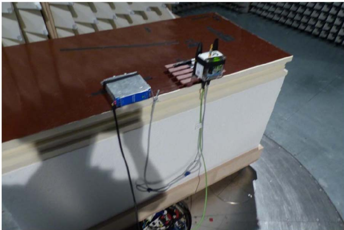
Test setup at 1GHz
