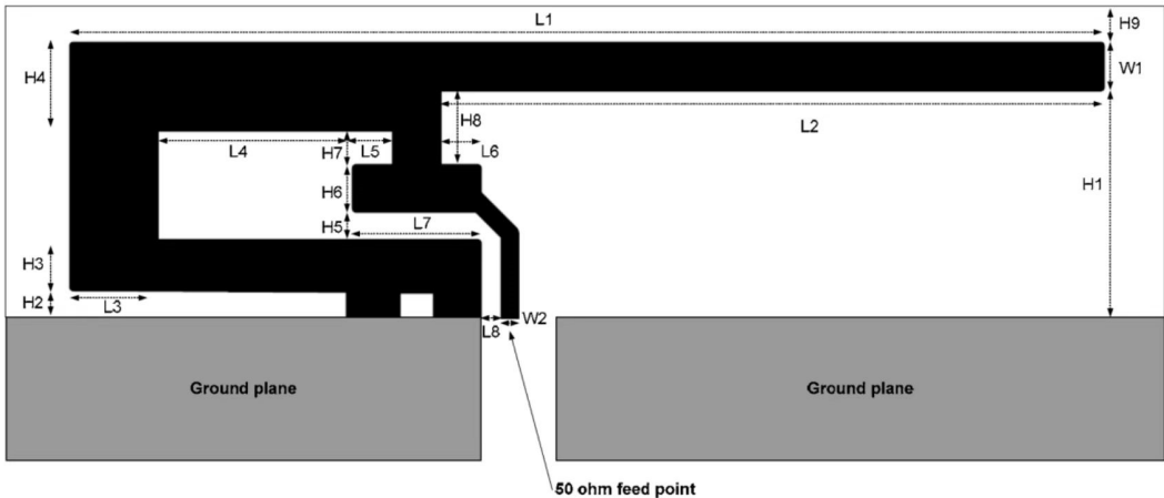
Figure 1-1. IFA Dimensions
