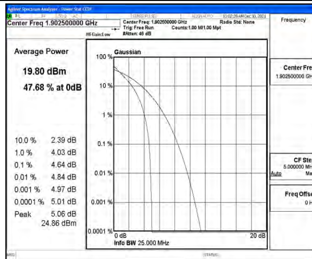
Band2-15MHz-16QAM-18675
