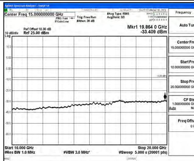
Band2-20MHz-16QAM-19100-Range5:10000~20000MHz
