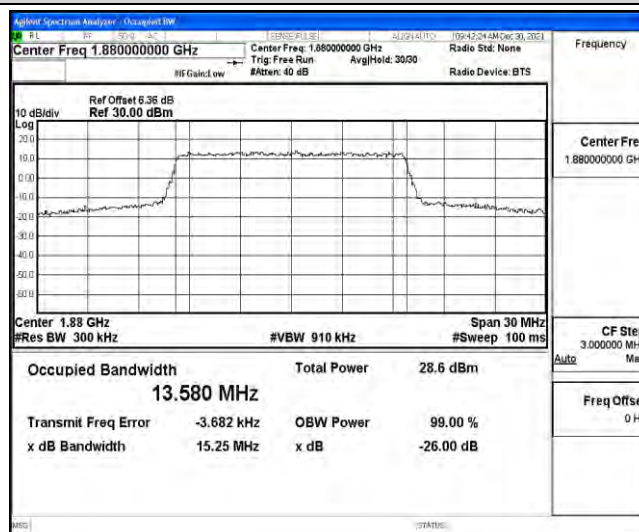
Band2-15MHz-QPSK-19125
