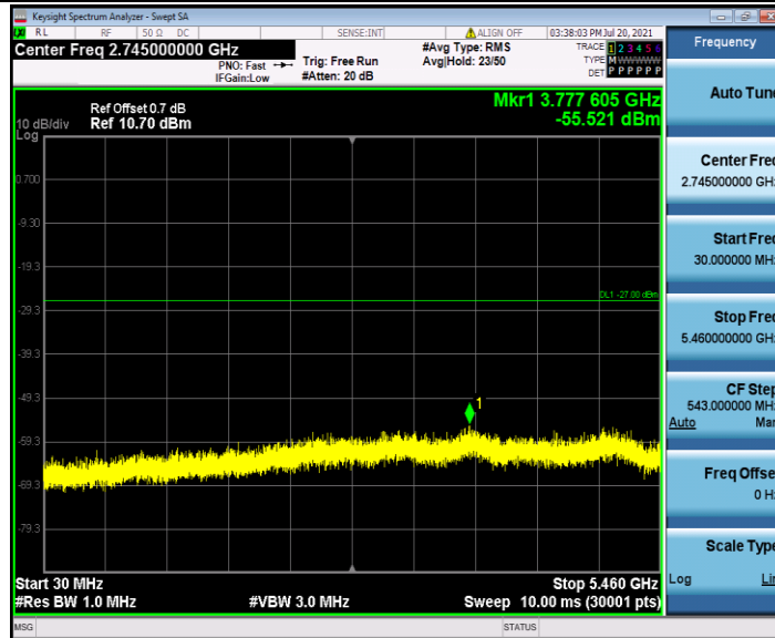
11AC40SISO_Ant2_5670_5735~40000
