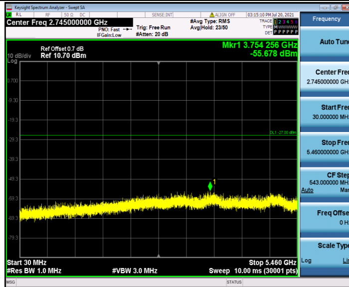
11AC40SISO_Ant1_5510_5735~40000
