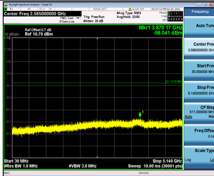
11AC40SISO_Ant2_5310_5360~40000
