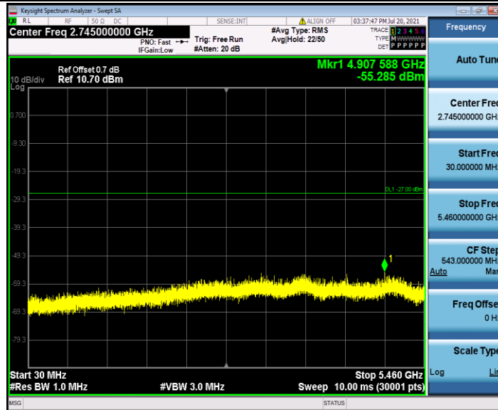
11AC40SISO_Ant2_5550_5735~40000
