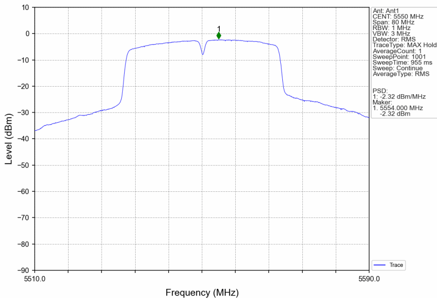
802.11ac(VHT40)_MCH_5550MHz_Ant1_NTNV
