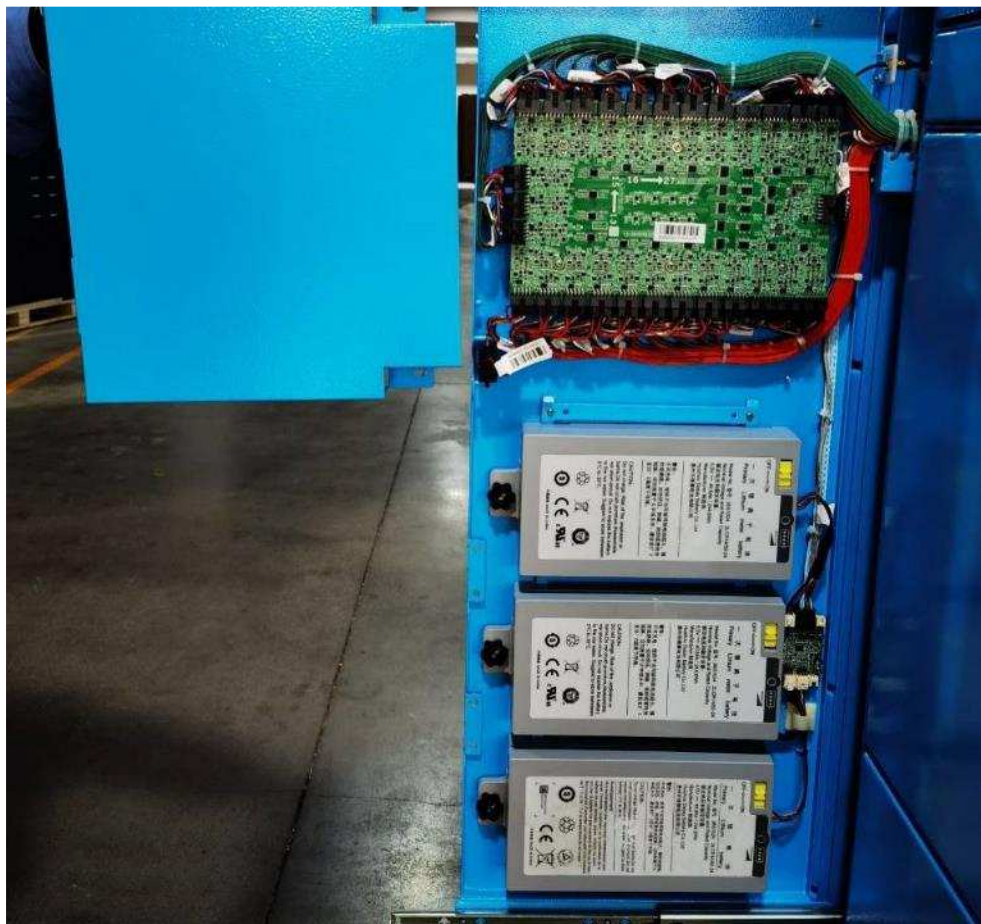
Internal view with 3pcs batteries
