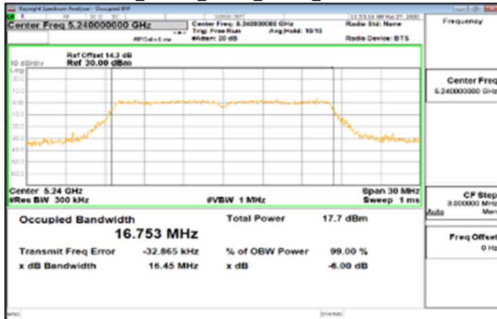
IC_802.11a_20MHz_Chain0_5240MHz
