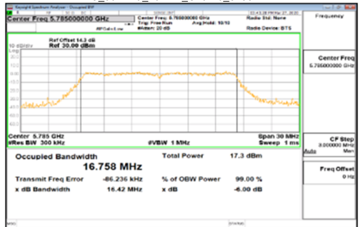
IC_802.11a_20MHz_Chain0_5785MHz
