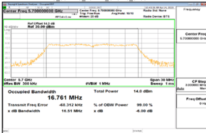
IC_802.11a_20MHz_Chain0_5700MHz
