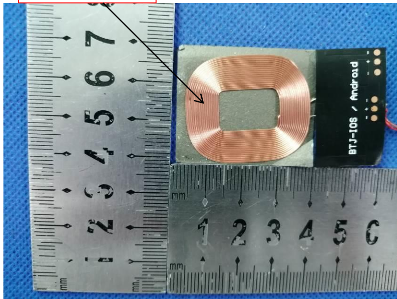
receiver antenna
