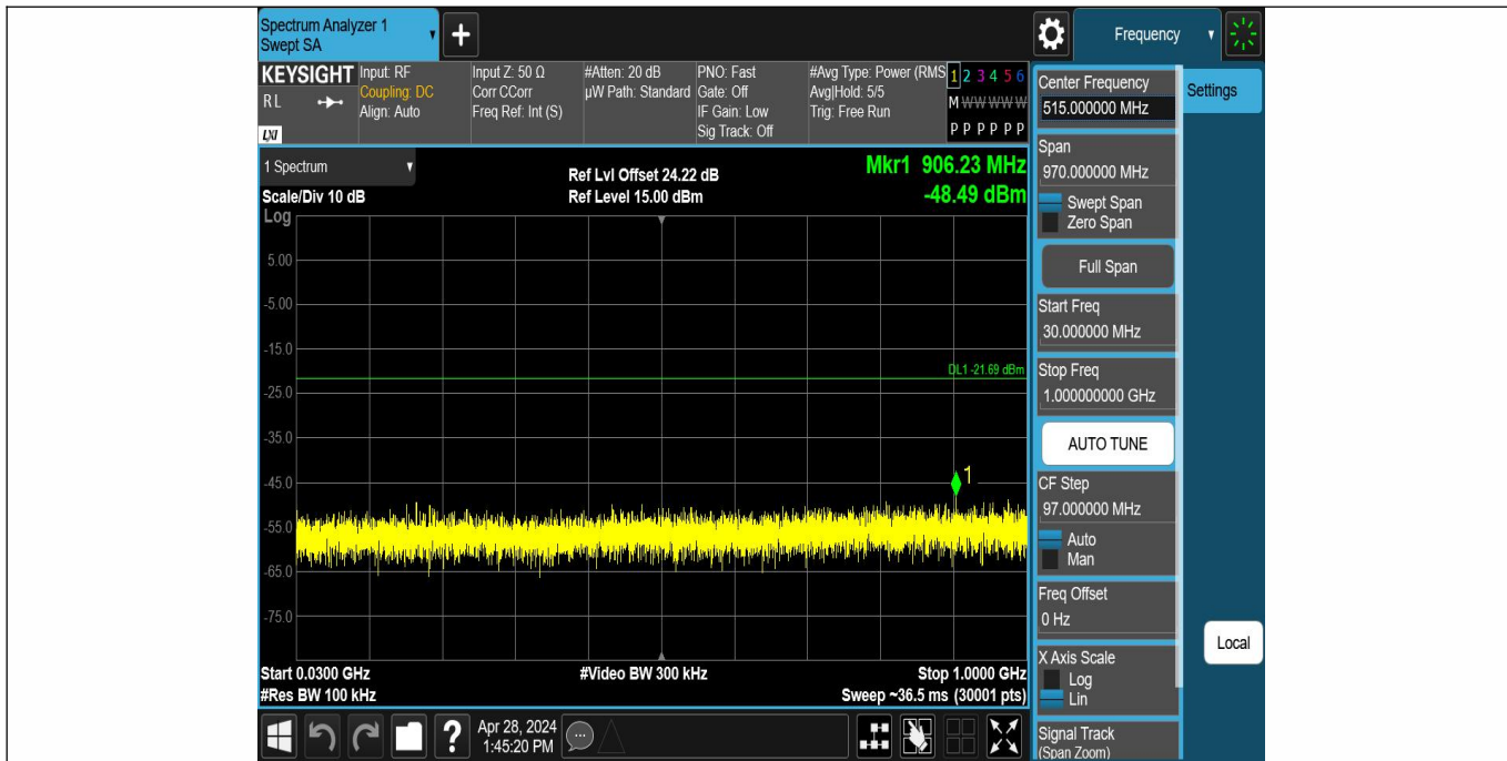
DH5-Ant1-2441-30~1000-PASS
