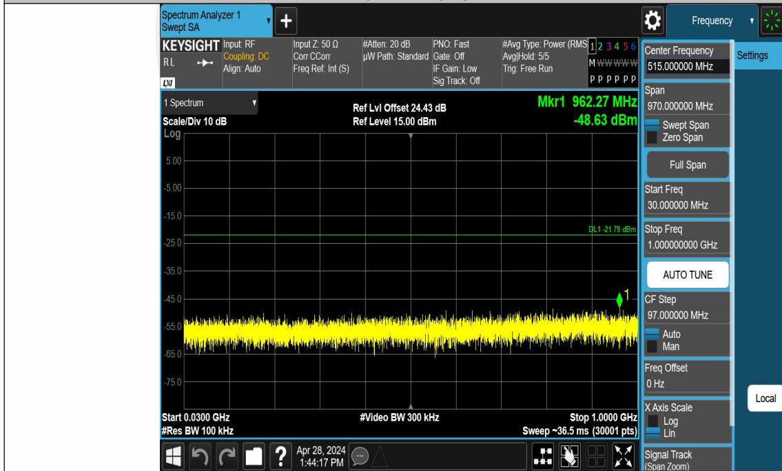
DH5-Ant1-2402-30~1000-PASS
