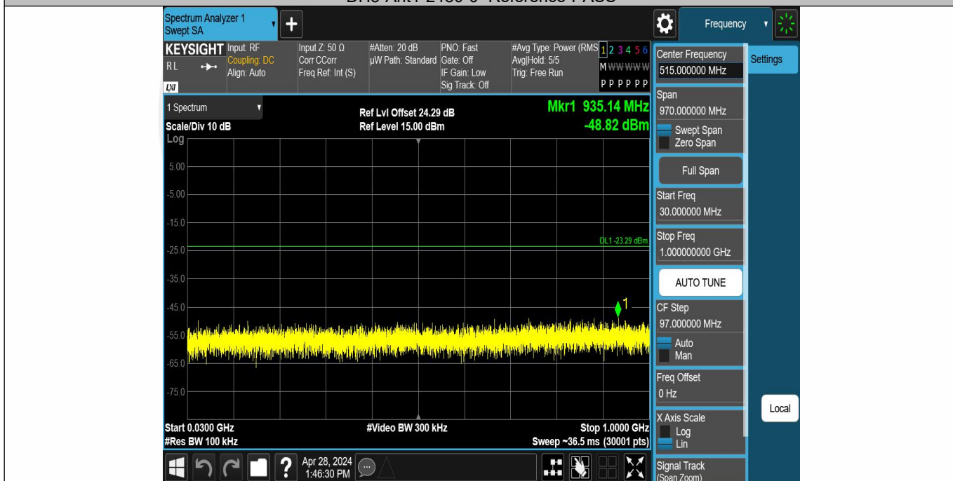
DH5-Ant1-2480-30~1000-PASS
