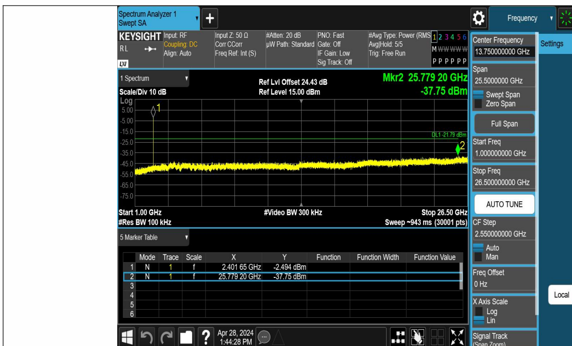
DH5-Ant1-2402-1000~26500-PASS
