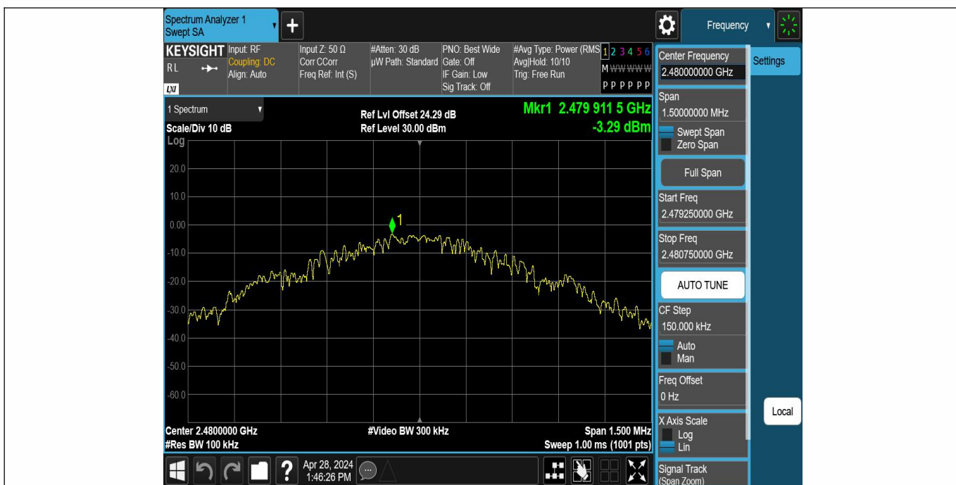
DH5-Ant1-2480-0~Reference-PASS
