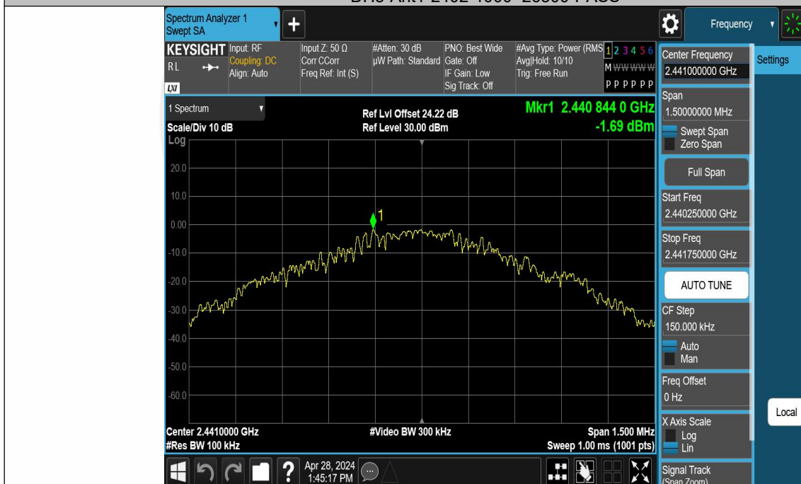
DH5-Ant1-2441-0~Reference-PASS
