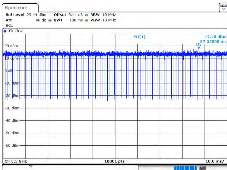
Duty Cycle NVNT 802.11ax20 5500MHz
