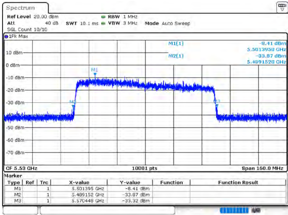
-26 dB BW NVNT 802.11ax80 5530MHz Ant 2
