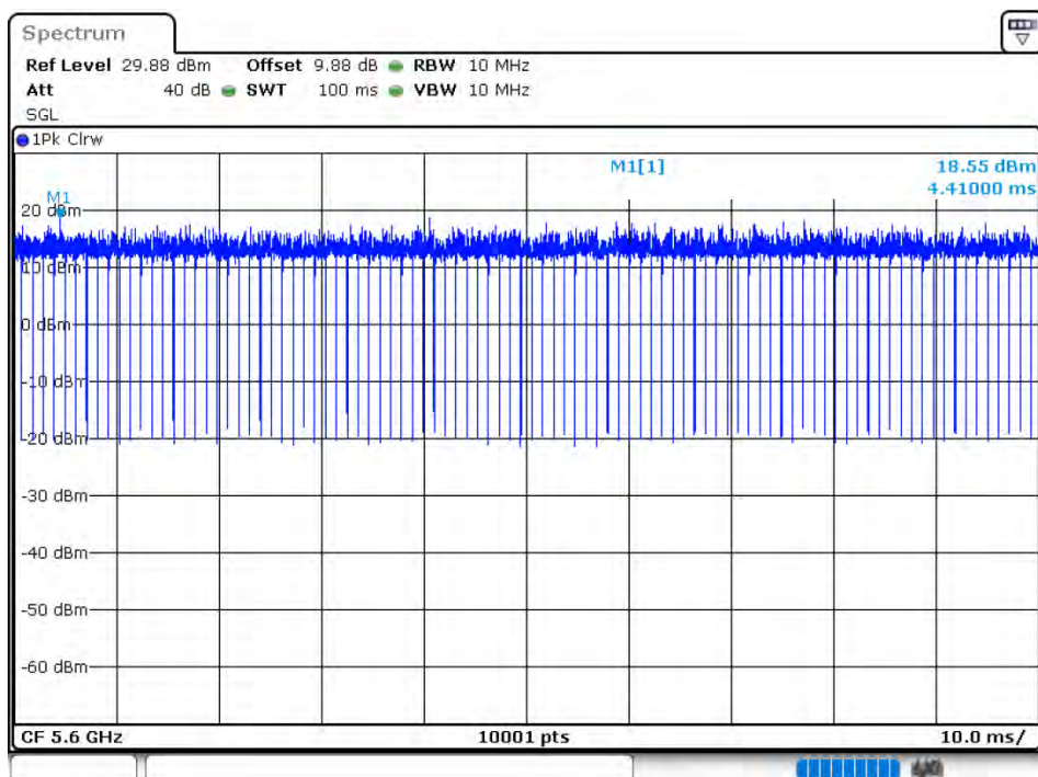
Duty Cycle NVNT 802.11ax20 5600MHz
