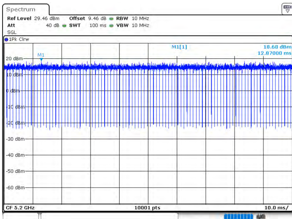
Duty Cycle NVNT 802.11ax20 5200MHz
