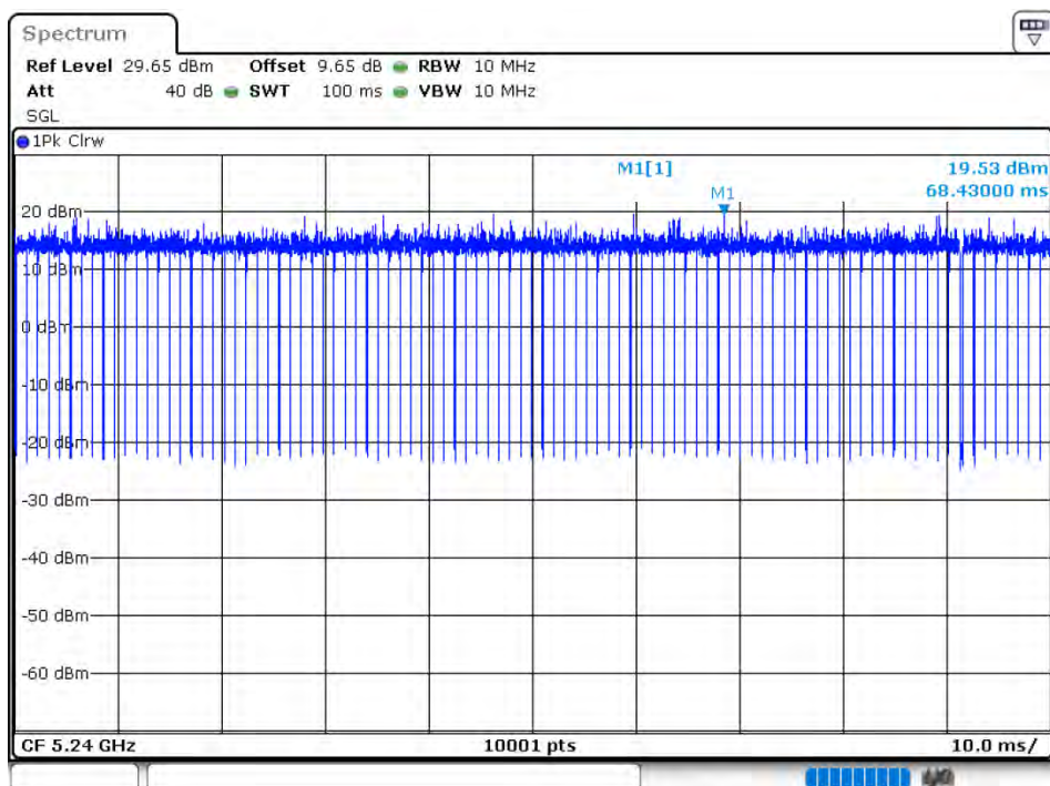
Duty Cycle NVNT 802.11ax20 5240MHz
