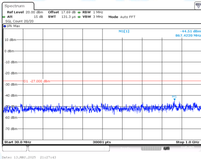
11AX40-CDD-Ant1-5795-30~1000-PASS
