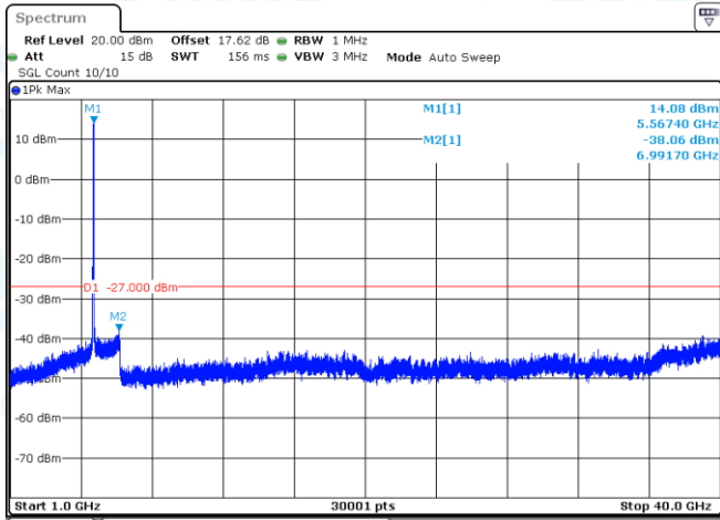
11AX40-CDD-Ant1-5550-1000~40000-PASS
