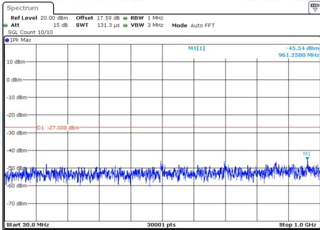
11AX20-CDD-Ant1-5580-30~1000-PASS
