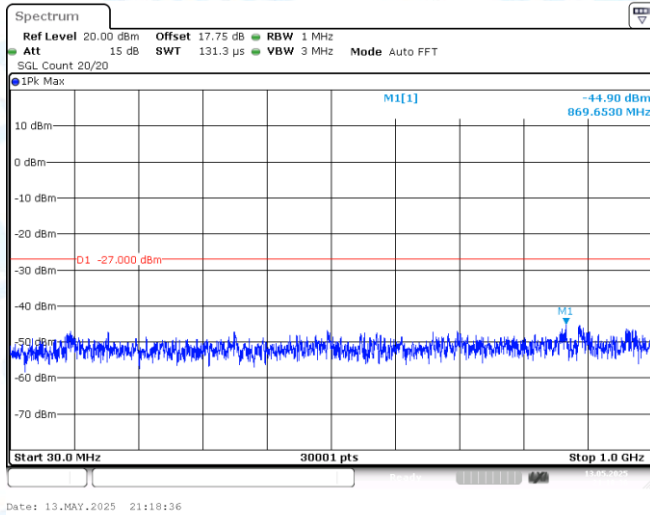
11AX40-CDD-Ant1-5755-30~1000-PASS
