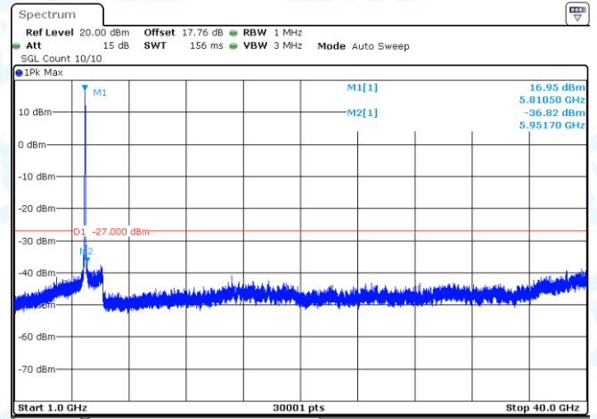
11AX40-CDD-Ant2-5795-1000~40000-PASS
