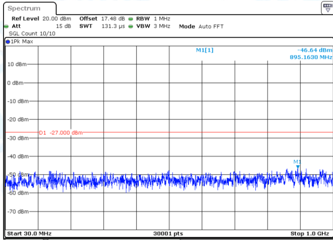
11AX40-CDD-Ant1-5230-30~1000-PASS
