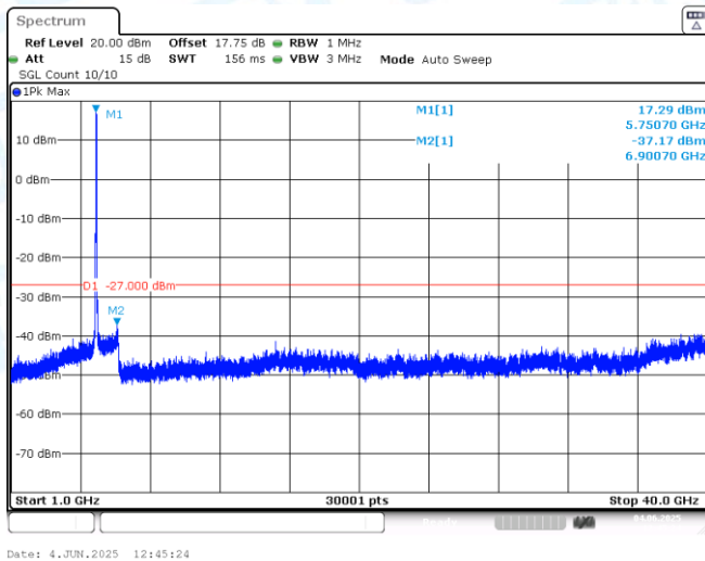
11AX40-CDD-Ant1-5755-1000~40000-PASS
