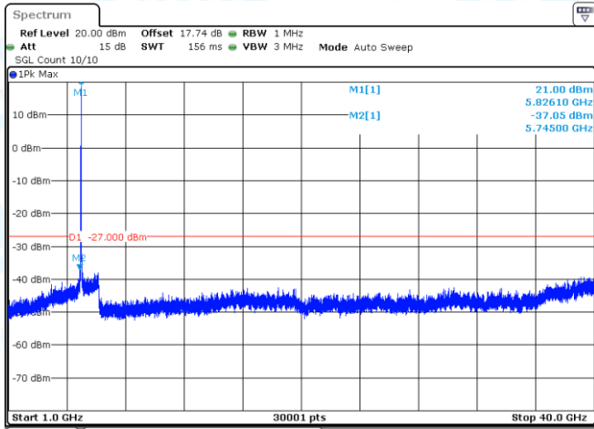
11AX20-CDD-Ant1-5825-1000~40000-PASS
