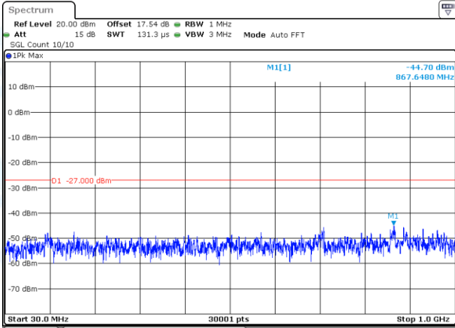
11AX40-CDD-Ant1-5510-30~1000-PASS
