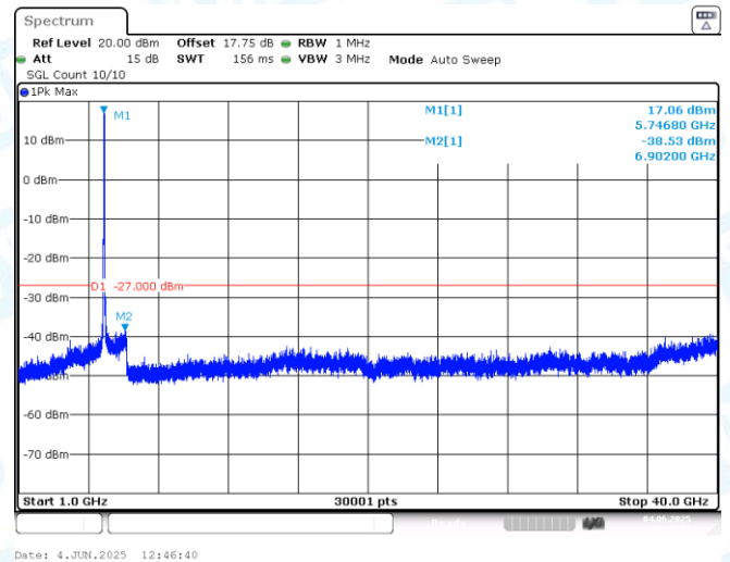
11AX40-CDD-Ant2-5755-1000~40000-PASS
