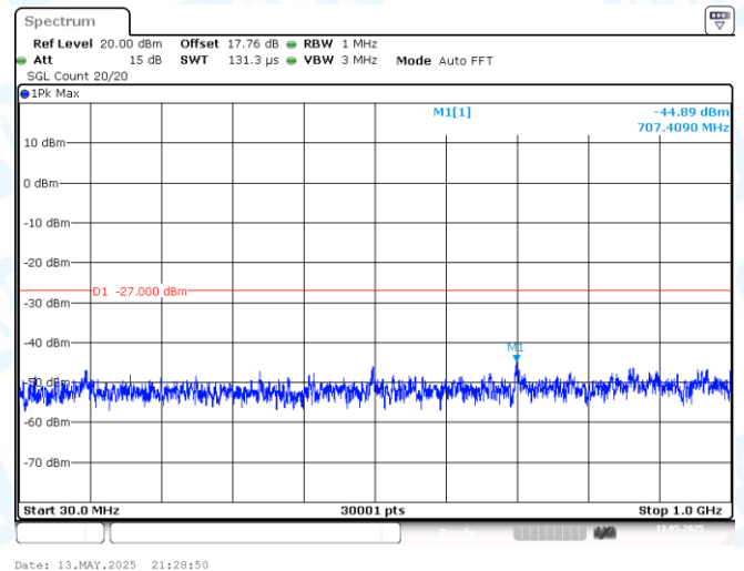
11AX40-CDD-Ant2-5795-30~1000-PASS
