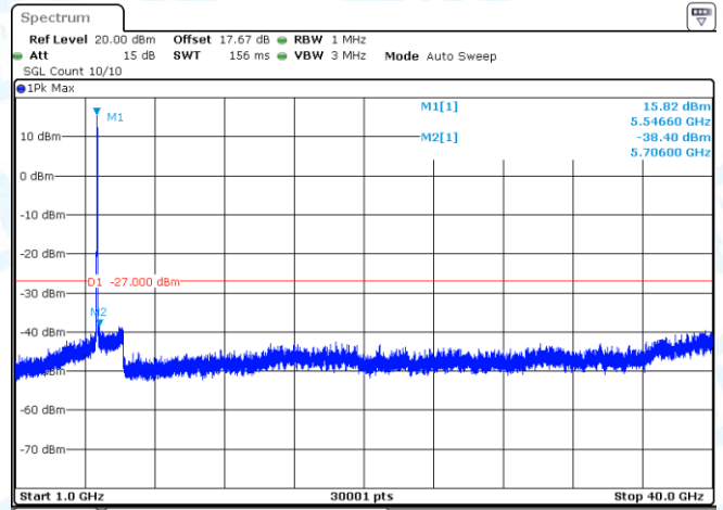
11AX40-CDD-Ant2-5550-1000~40000-PASS
