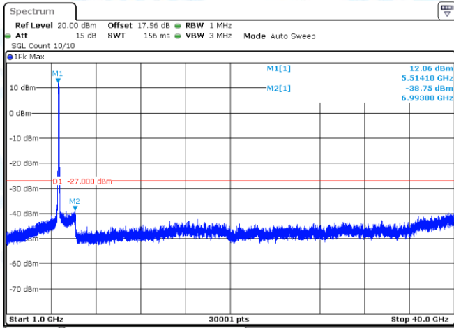
11AX80-CDD-Ant1-5530-1000~40000-PASS
