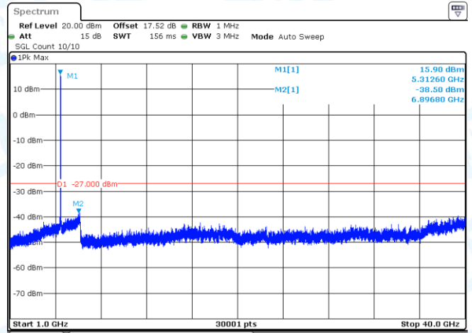
11AX20-CDD-Ant2-5320-1000~40000-PASS
