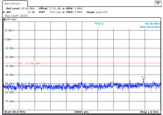
11AX40-CDD-Ant2-5510-30~1000-PASS
