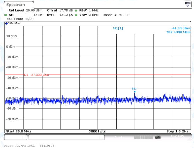
11AX40-CDD-Ant2-5755-30~1000-PASS
