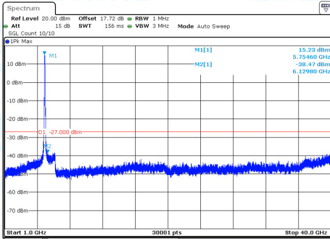
11AX80-CDD-Ant1-5775-1000~40000-PASS
