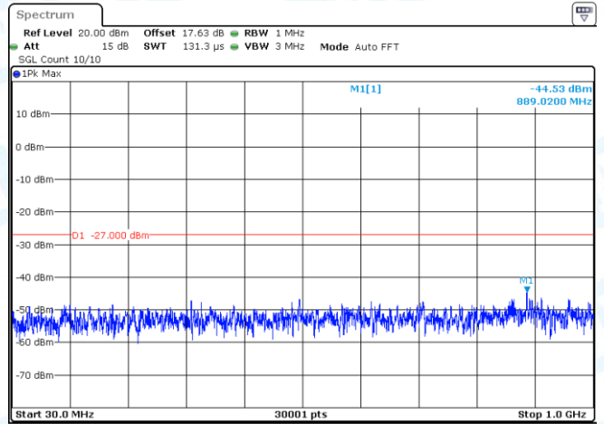
11AX20-CDD-Ant2-5580-30~1000-PASS
