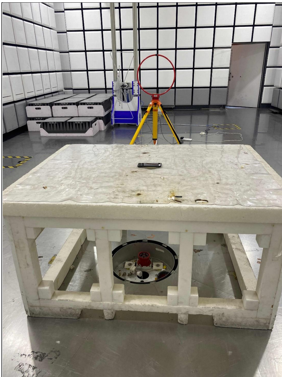
RADIATED EMISSION TEST (Below 30MHz)
